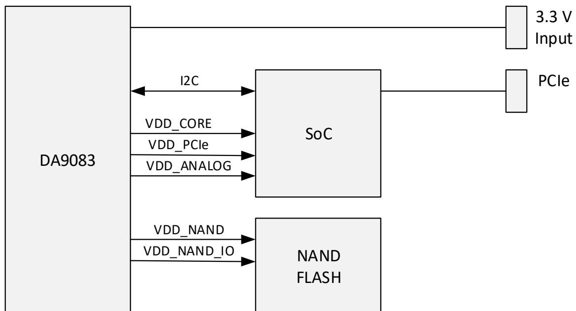
Figure 1. System Diagram
