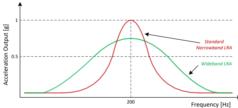
Figure 6: Narrowband and Wideband LRA Response across Frequency
