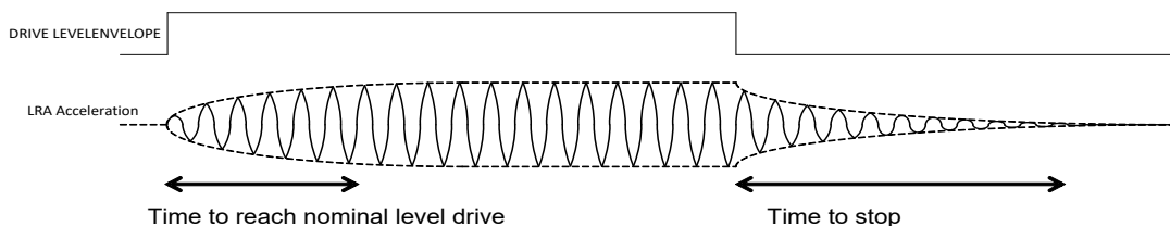
Figure 10: LRA Single Step Drive without Acceleration and Rapid Stop
