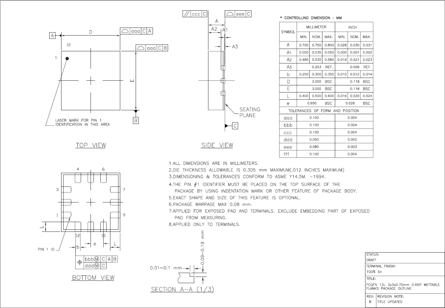
Figure 40: QFN Package Outline Drawing
