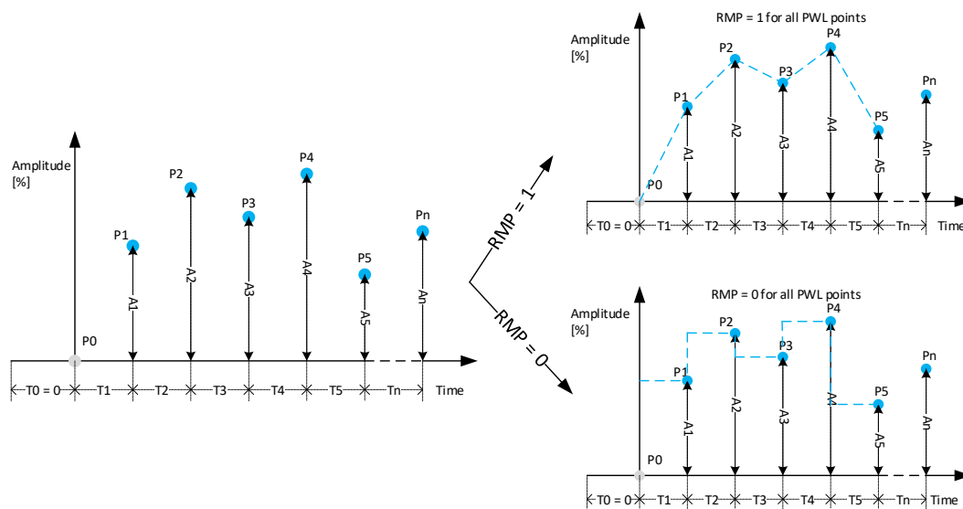
Figure 26: Snippet Example
