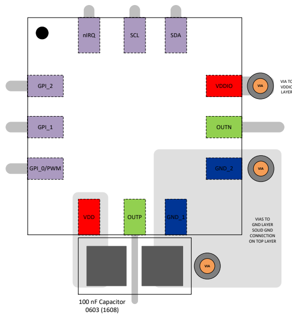
Figure 42: QFN Example PCB Layout
