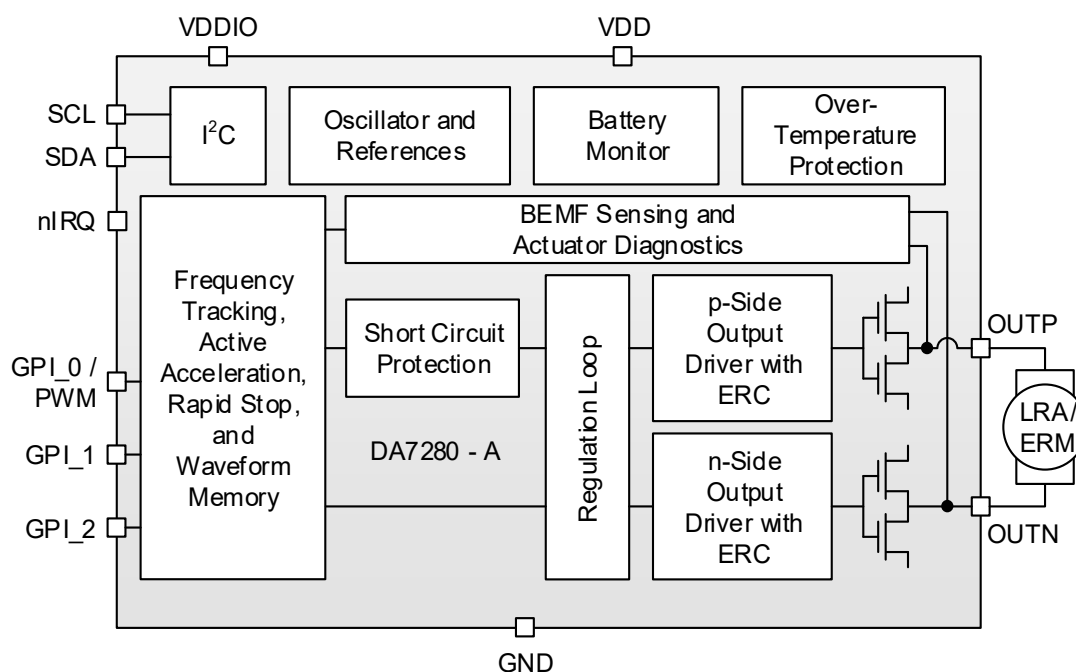
Figure 2: DA7280-A Block Diagram
