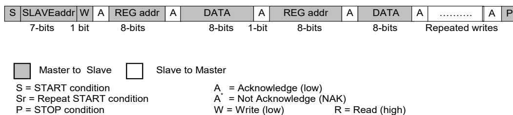
Figure 38: I²C Repeated Write (SDA line)
