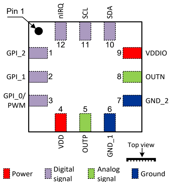
Figure 3: DA7280-A QFN Pinout Diagram (Top View)
