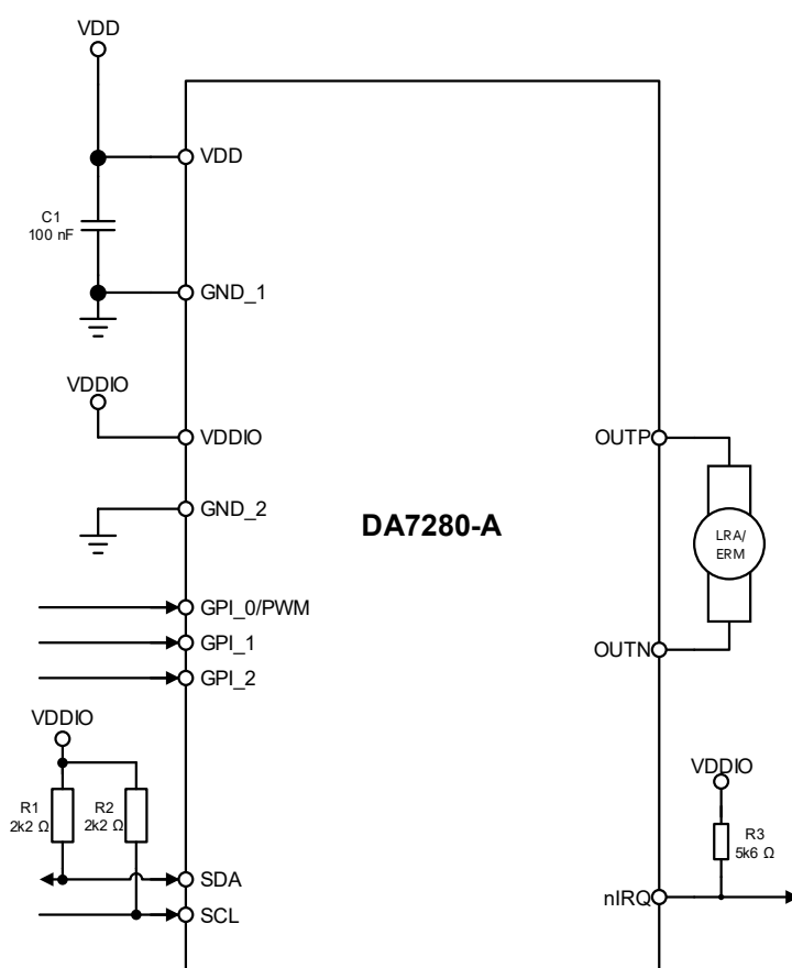
Figure 41: External Components Diagram
