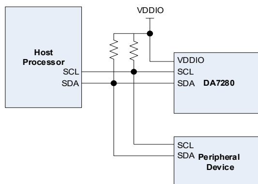
Figure 32: Schematic of the I²C Control Interface Bus
