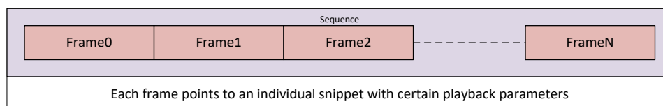
Figure 28: Sequence Structure
