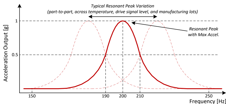
Figure 5: LRA Output Acceleration Swept in Frequency with Constant Power Input Signal
