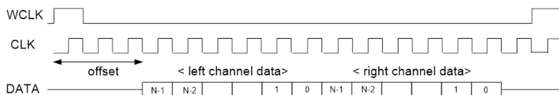
Figure 34. TDM DSP format
