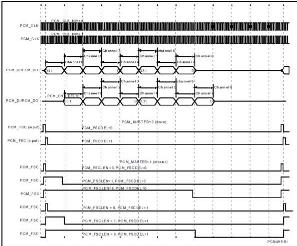
Figure 64. PCM interface formats
