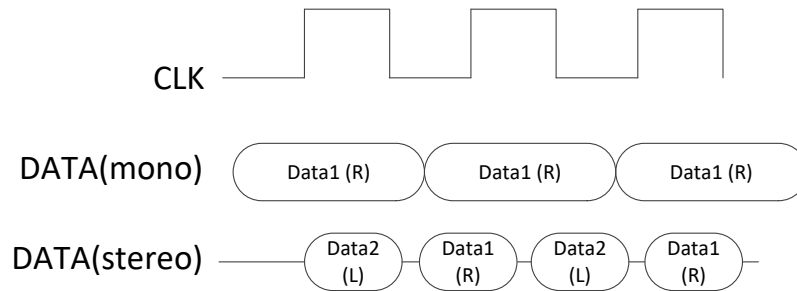
Figure 68. PDM Mono/Stereo formats
