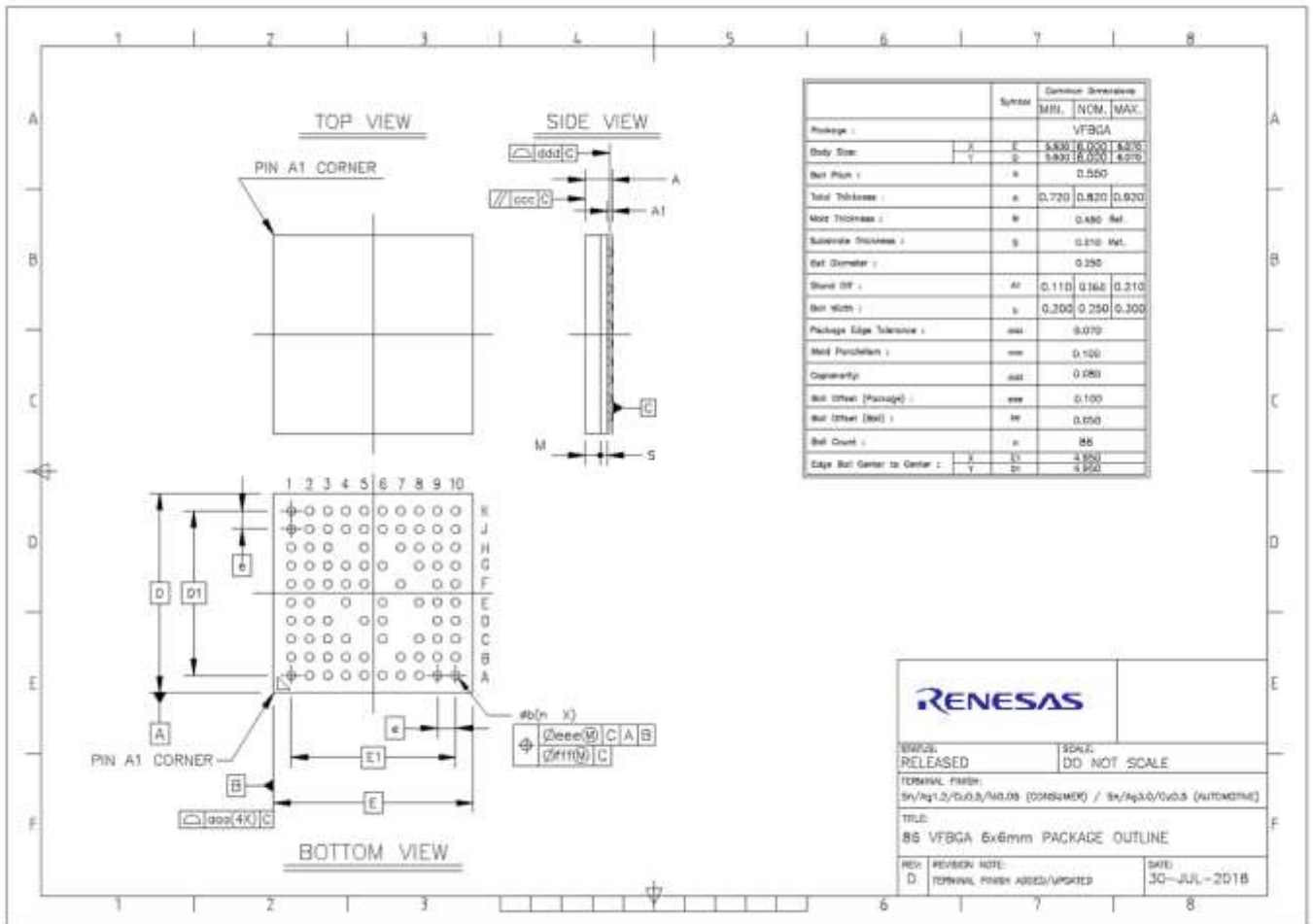
Figure 112. VFBGA86 Package outline drawing
