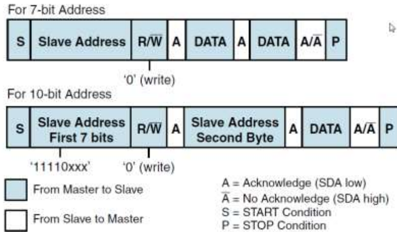
Figure 75. Master-Transmitter protocol
