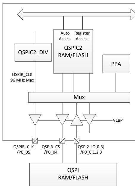
Figure 44. Quad SPI RAM/Flash controller
