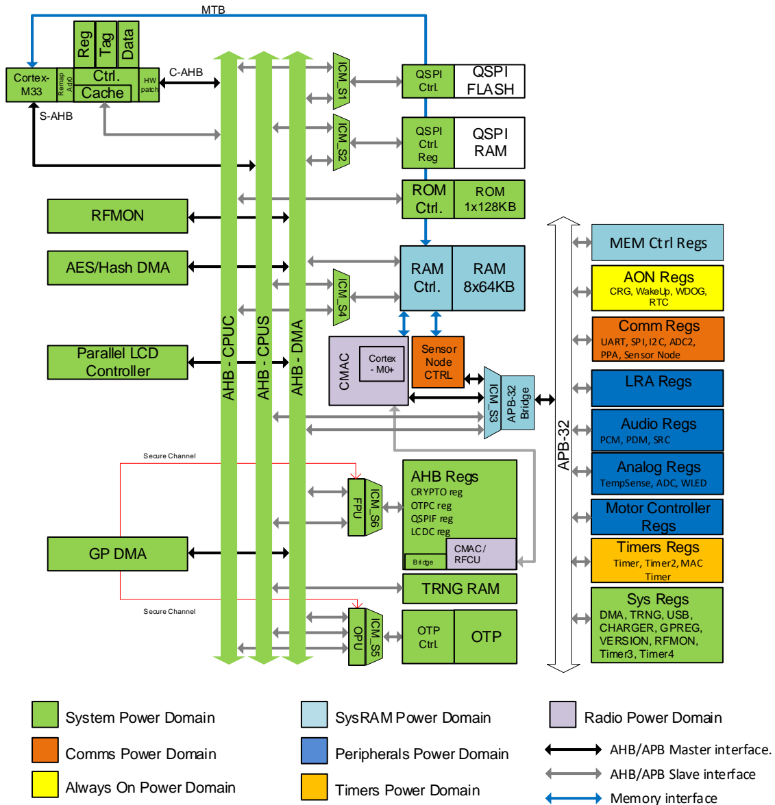
Figure 30. Bus architecture
