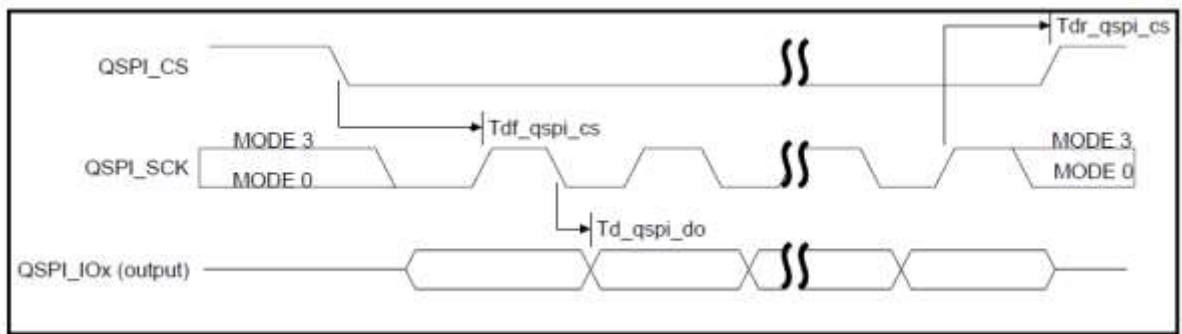
Figure 43: QSPI output timing
