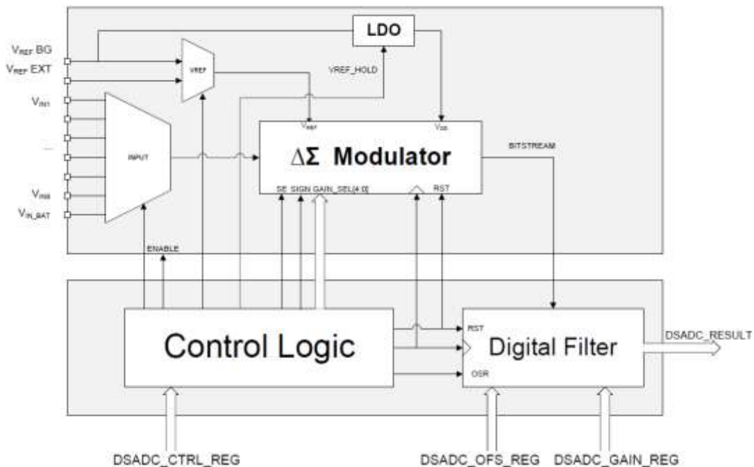
Figure 62. Block diagram of the \Delta\Sigma ADC
