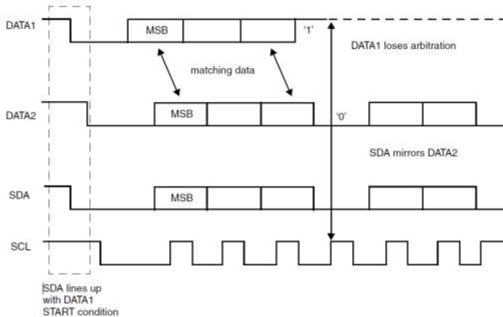
Figure 78. Multiple Master arbitration
