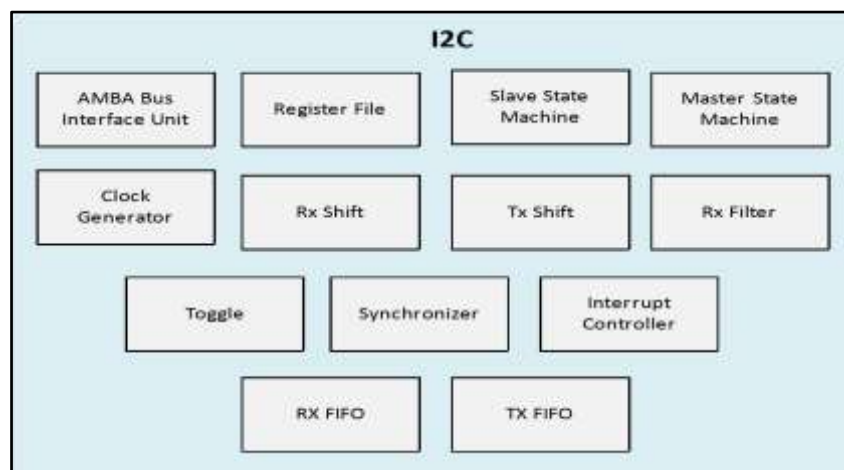
Figure 70. I2C Controller block diagram
