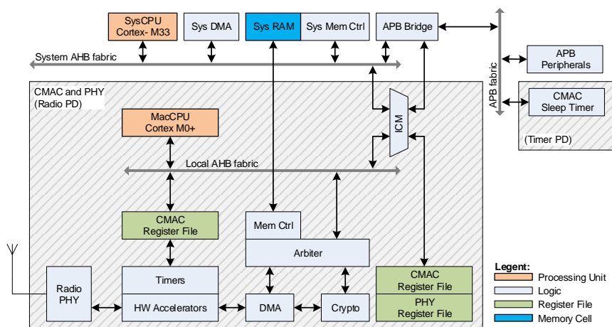
Figure 31. Configurable MAC block diagram
