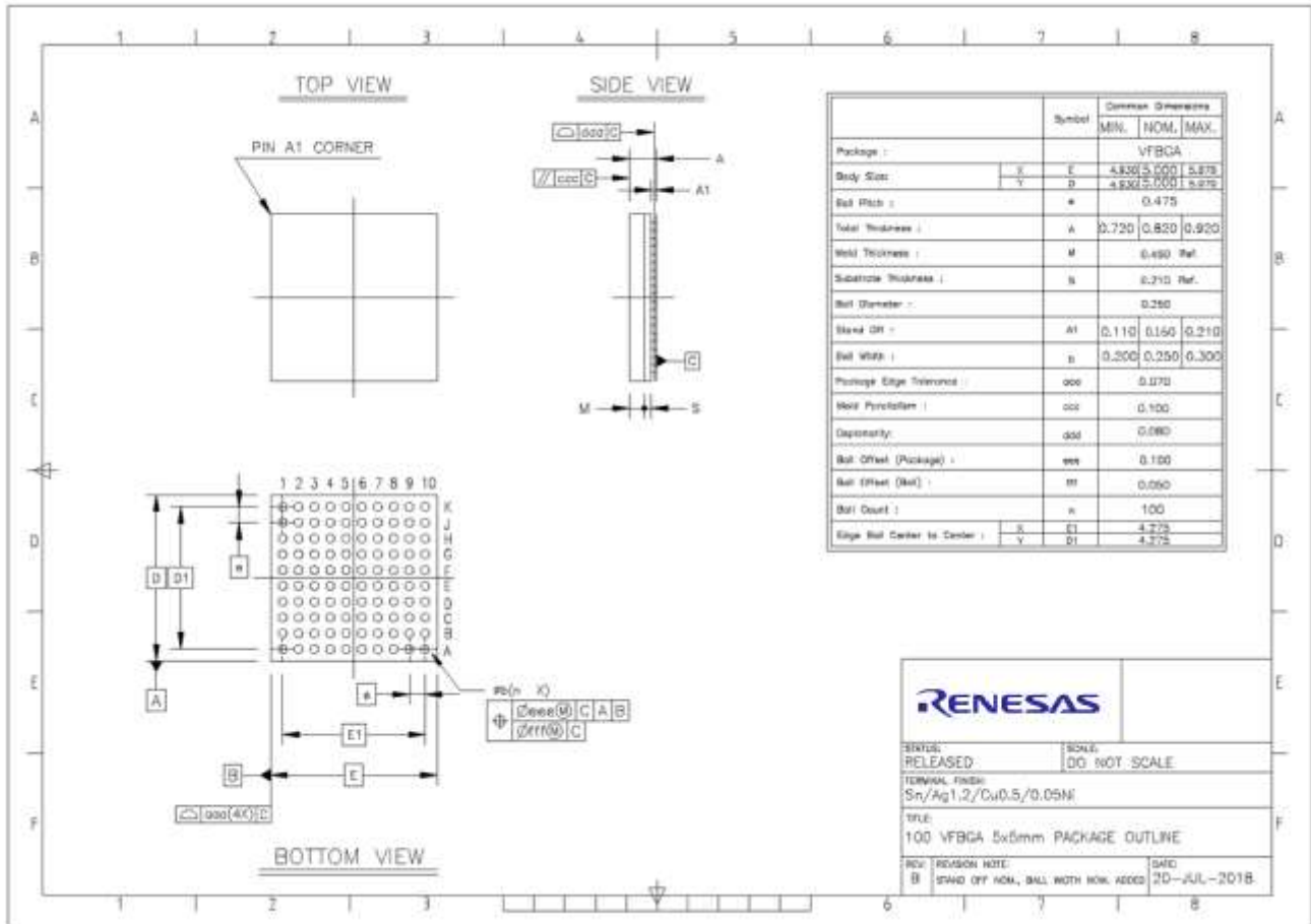
Figure 113. VFPGA100 Package outline drawing
