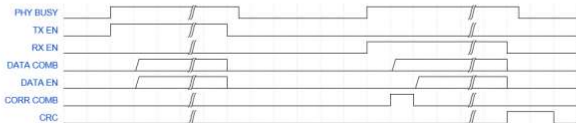
Figure 32. CMAC diagnostics timing diagram
