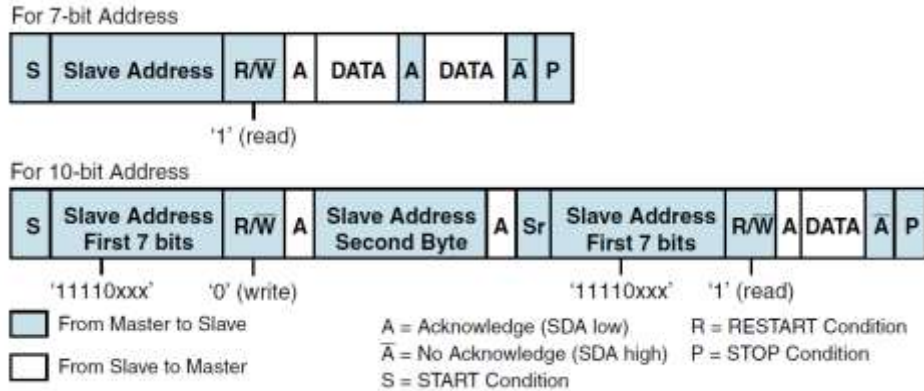
Figure 76. Master-Receiver protocol
