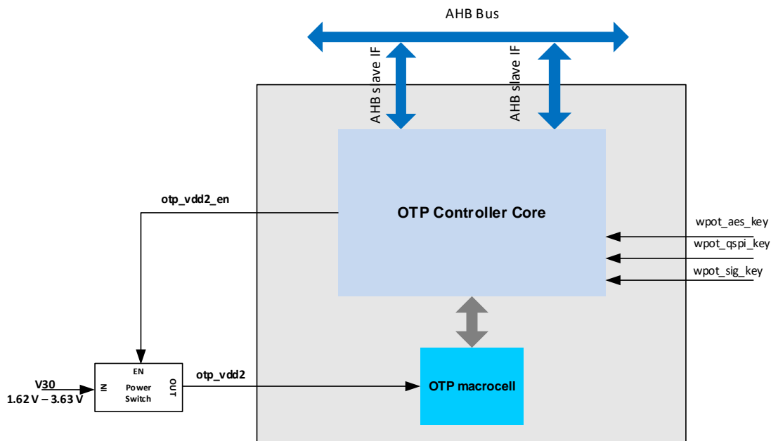
Figure 39. OTP controller block diagram
