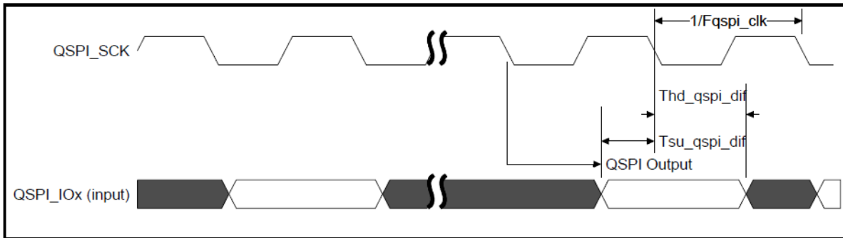
Figure 42. QSPI input timing
