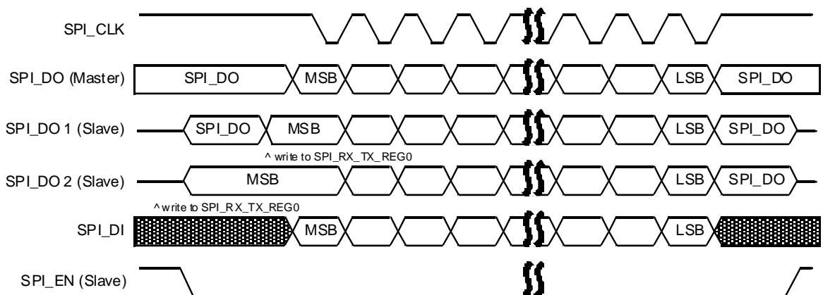
Figure 89. SPI Master/Slave mode 2: SPI_POL=1 and SPI_PHA=0
