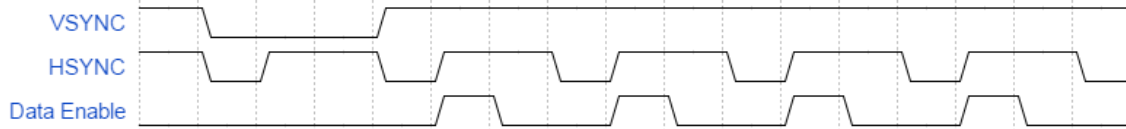
Figure 53: HSYNC/VSYNC Typical Waveform
