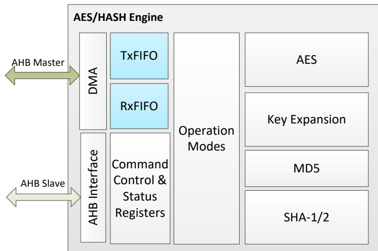
Figure 57. AES/HASH architecture
