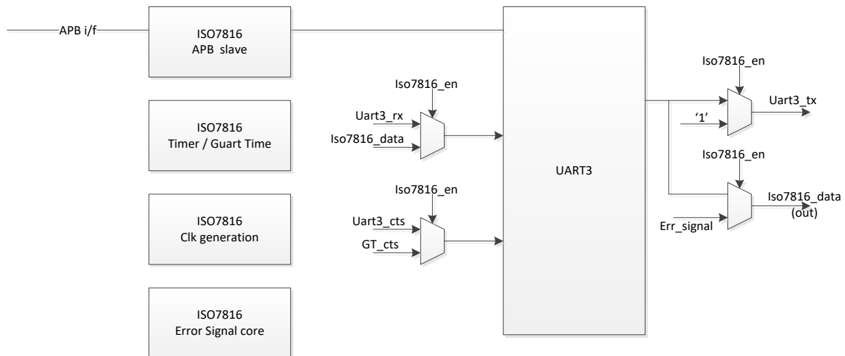
Figure 85. Smart Card (ISO7816-3) block diagram
