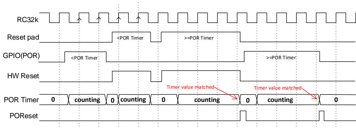
Figure 27. Power-on reset timing diagram
