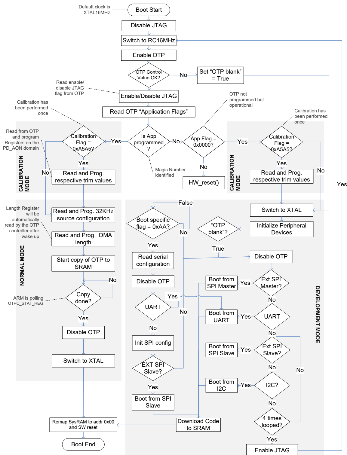
Figure 9: BootROM Sequence
