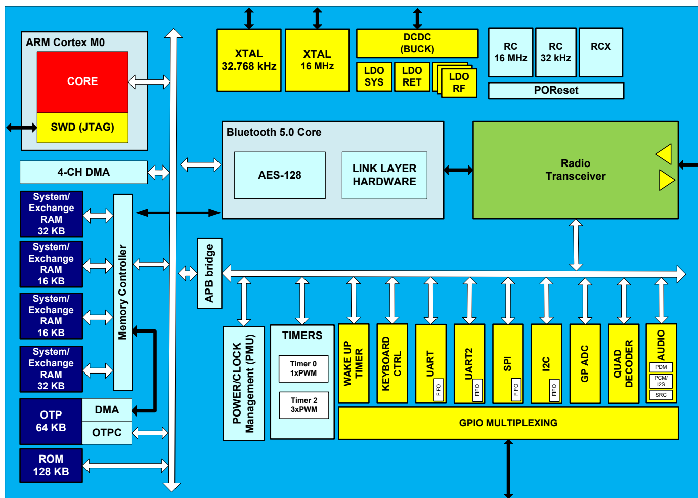
Figure 2: DA14585 High Temperature Block Diagram
