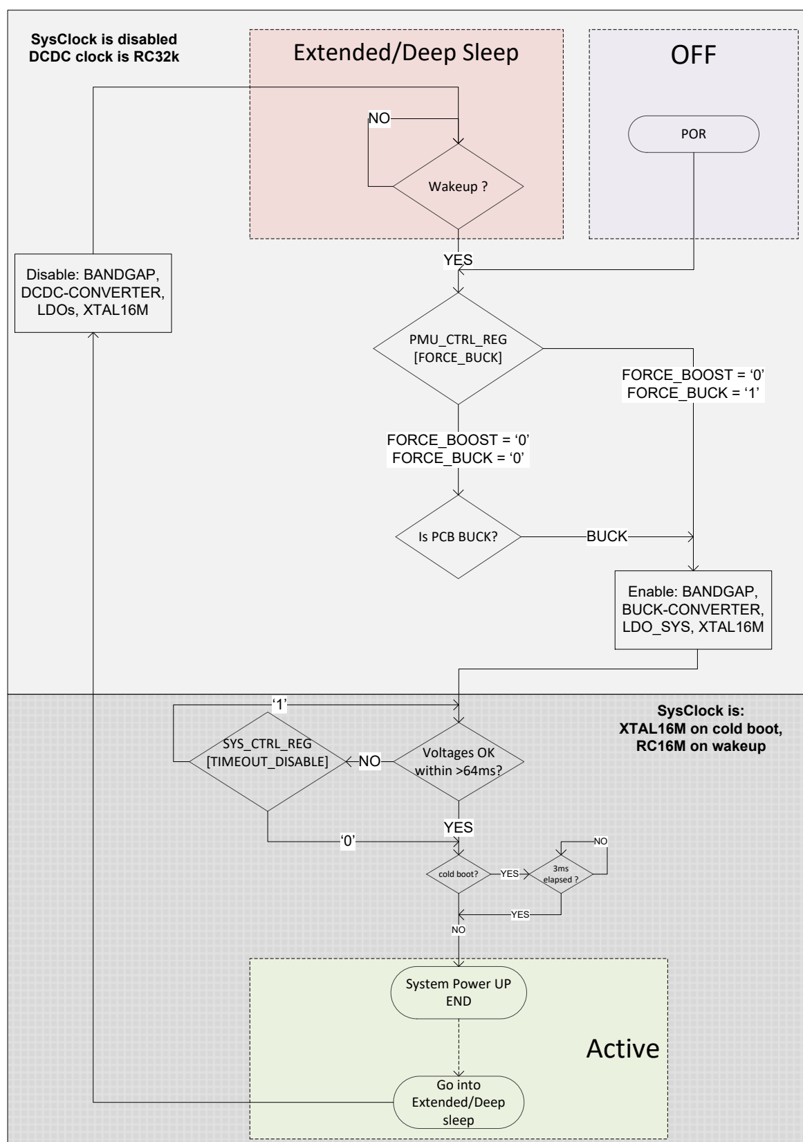
Figure 7: Power/Wake-Up Sequence
