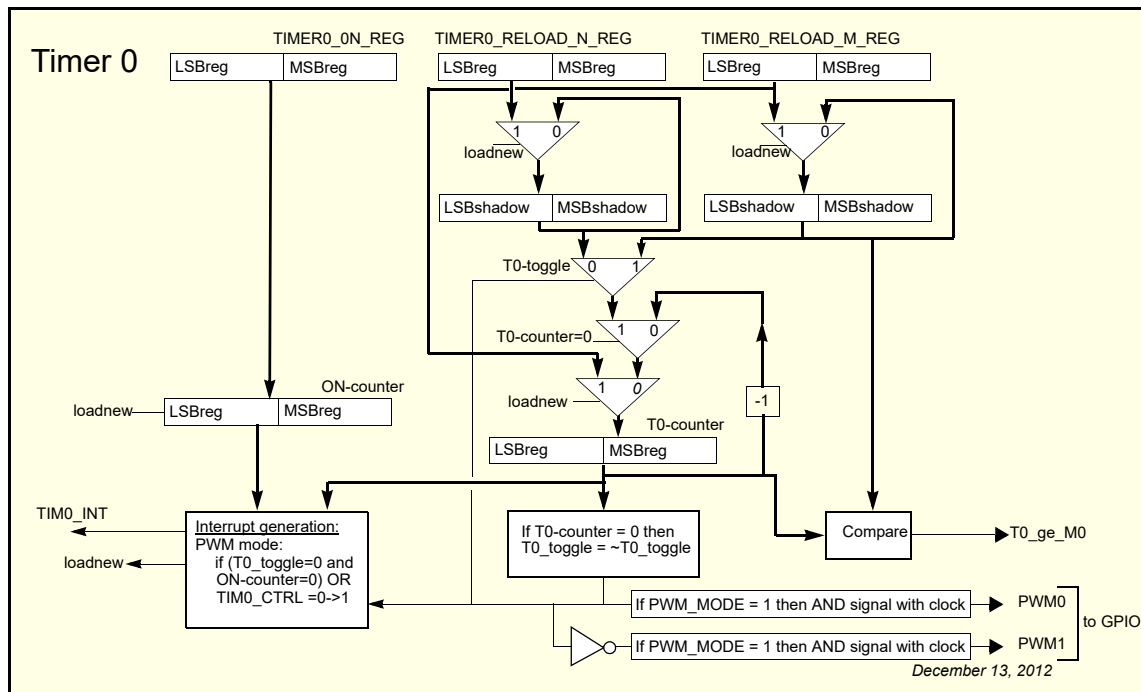
Figure 1: Timer 0 Block Diagram
