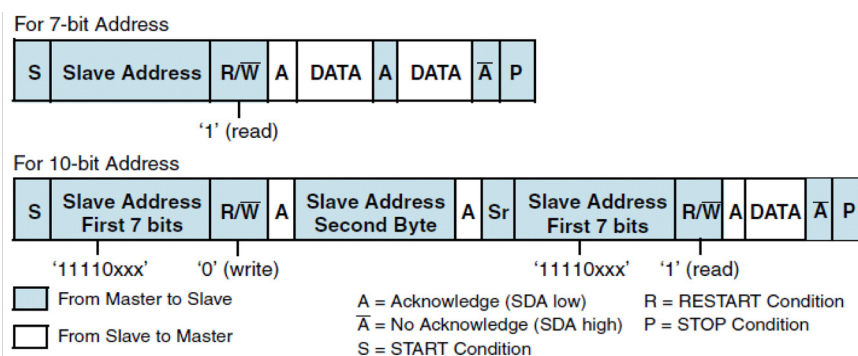
Figure 8: Master-Receiver Protocol
