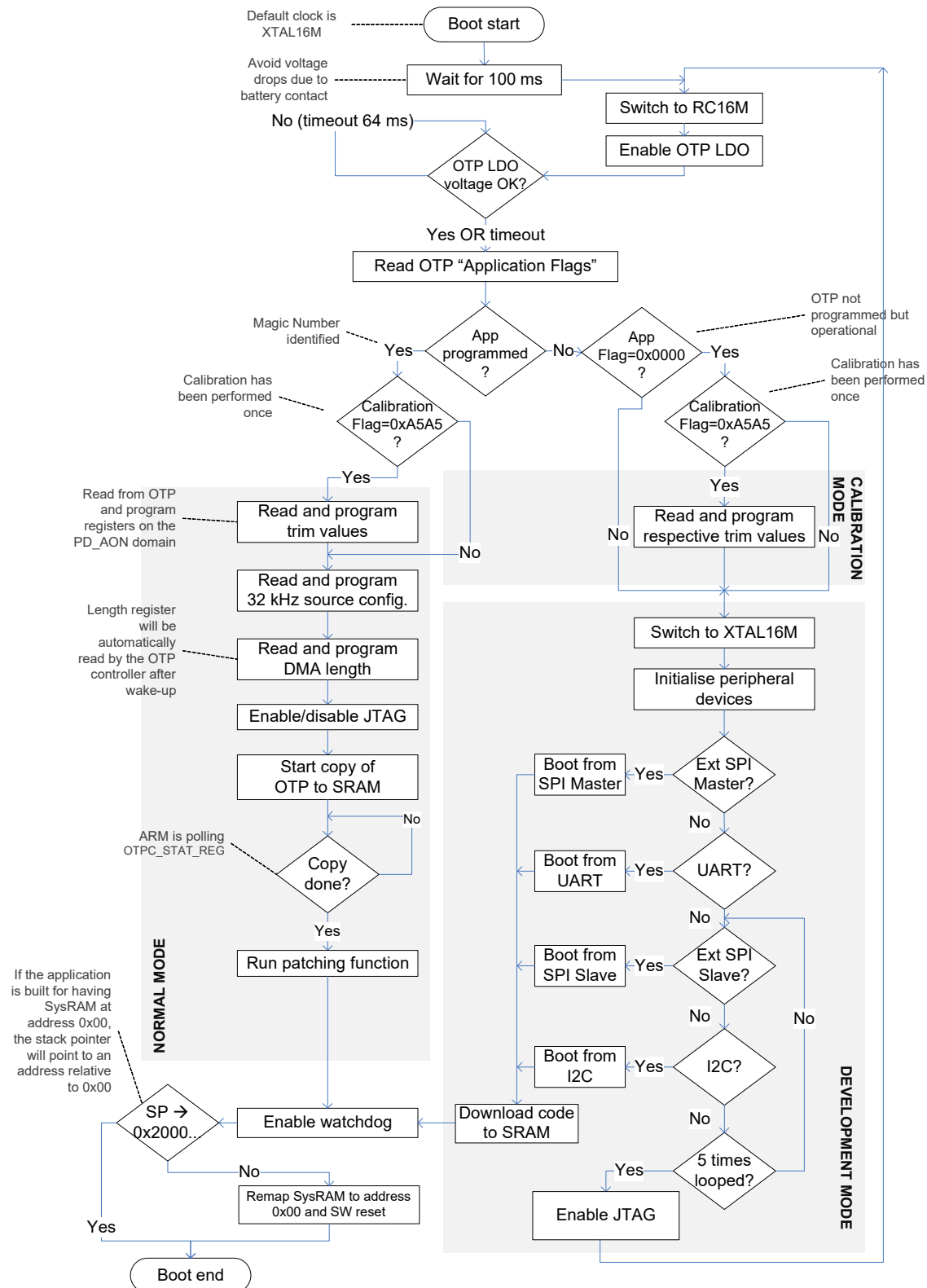
Figure 5: BootROM Sequence
