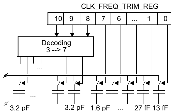
Figure 2: Frequency Trimming
