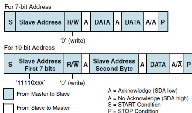
Figure 7: Master-Transmitter Protocol
