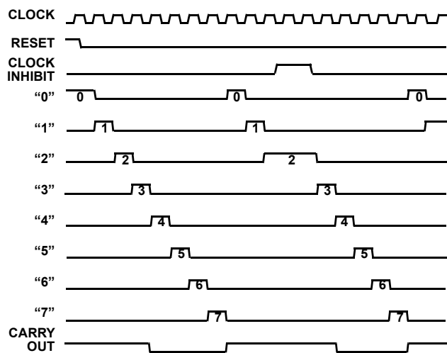
FIGURE 4. CD4022BMS
