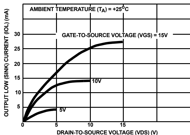
FIGURE 5. TYPICAL OUTPUT LOW (SINK) CURRENT CHARACTERISTICS
