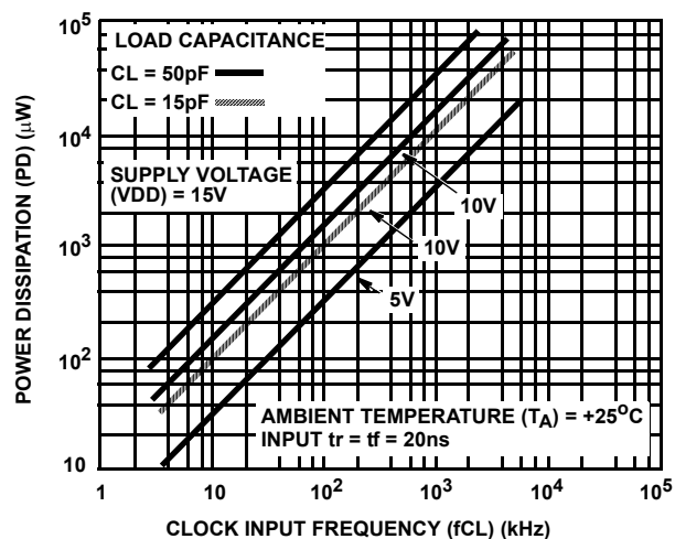
FIGURE 12. TYPICAL DYNAMIC POWER DISSIPATION AS A FUNCTION OF CLOCK INPUT FREQUENCY
