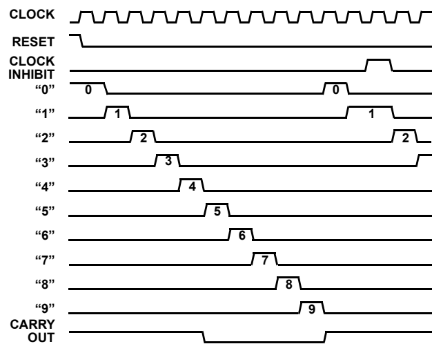
FIGURE 3. CD4017BMS
