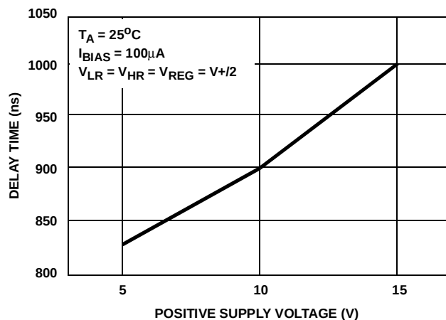
FIGURE 16. DELAY TIME vs SUPPLY VOLTAGE
