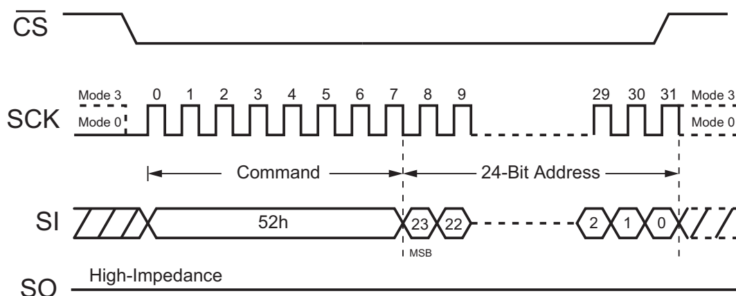
Figure 73. 32 kB Block Erase Command (SPI Mode)
