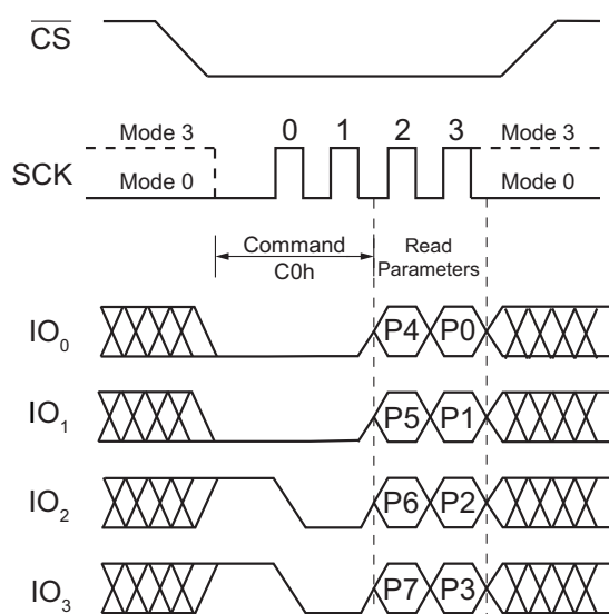
Figure 44. Set Read Parameters Command (QPI Mode)
