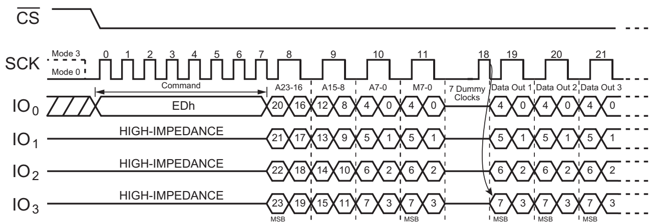
Figure 37. DTR Fast Read Quad I/O (SPI Mode; Initial instruction or previous M5-4 ≠ 1,0)
