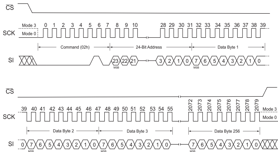
Figure 68. Page Program Command (SPI Mode)
