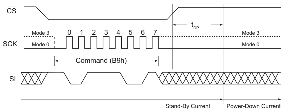
Figure 54. Deep Power-Down Command (SPI Mode)
