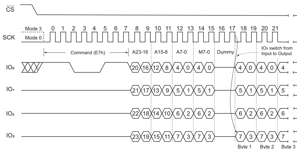
Figure 41. Word Read Quad I/O Command (Initial command or previous set M5-4 ≠ 1,0; SPI Mode)
