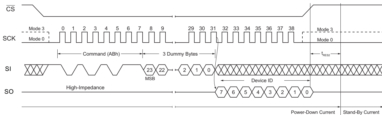
Figure 58. Release Power-Down / Device ID Command (SPI Mode)
