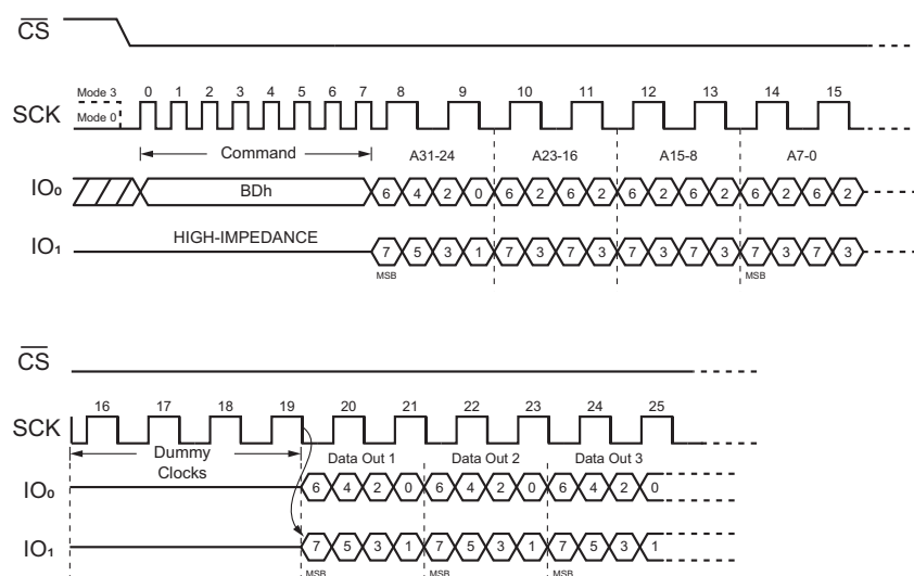
Figure 31. DTR Fast Read Dual I/O (SPI Mode only; Initial instruction or previous M5-4 = 10)
