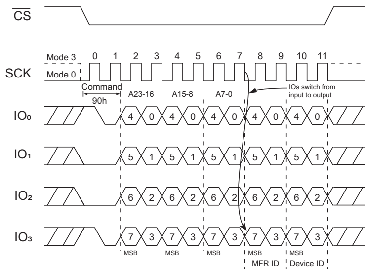
Figure 48. Read Manufacturer/ Device ID Command (QPI Mode)
