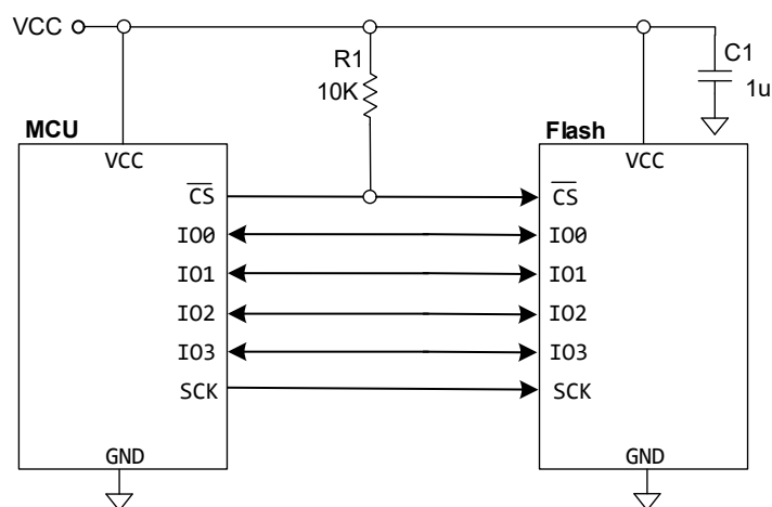
Figure 4. AT25SF0641C / AT25QF0641C Typical Application Block Diagram for QPI/QSPI
