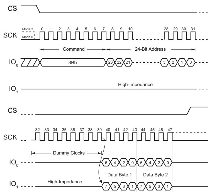
Figure 27. Fast Read Dual Output command (SPI Mode)
