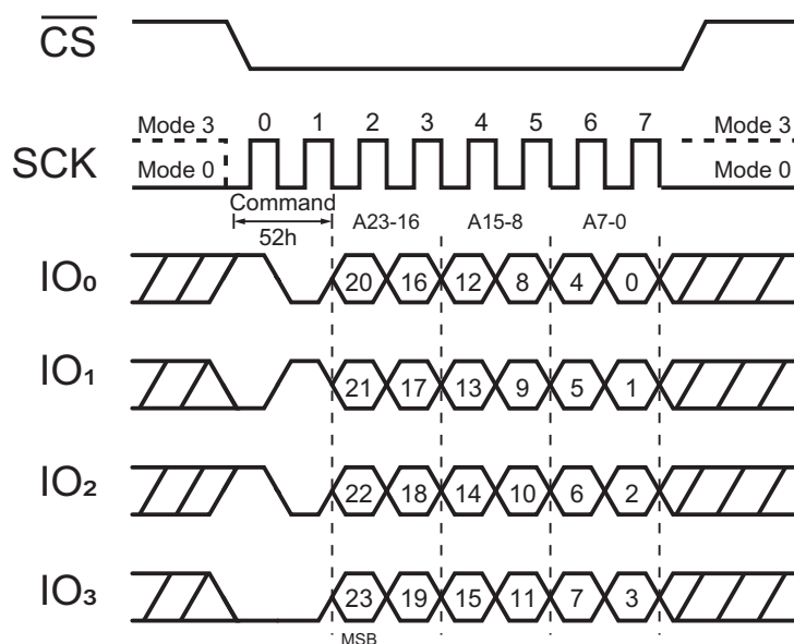
Figure 74. 32 kB Block Erase Command (QPI Mode)
