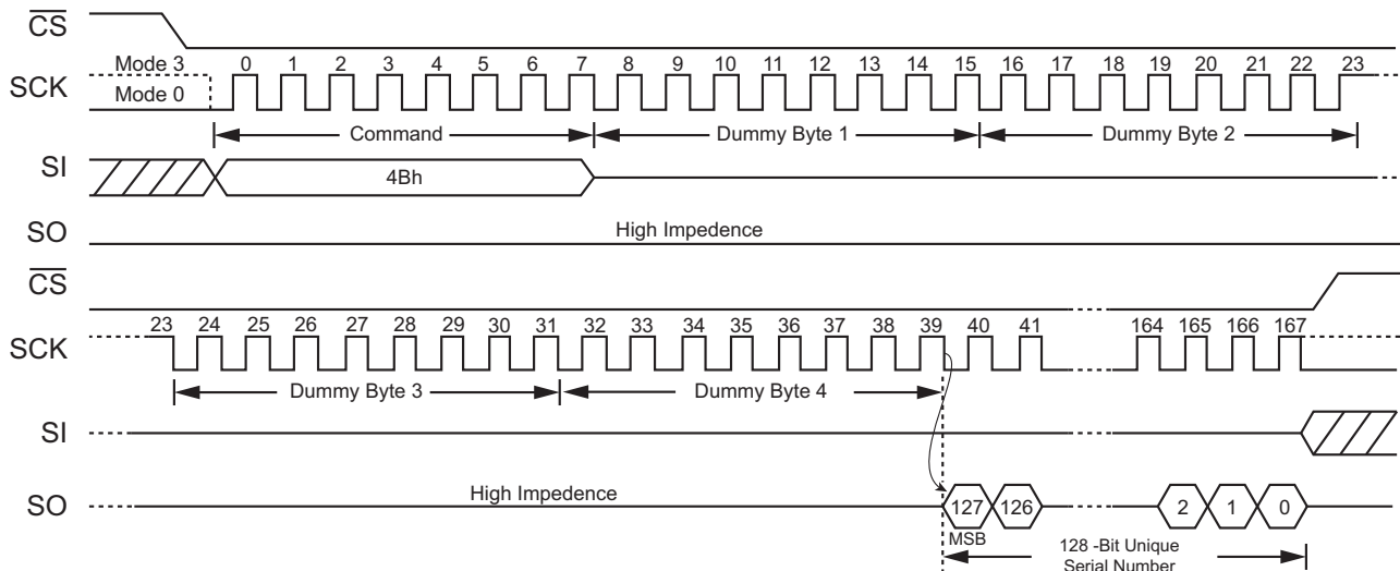
Figure 53. Read Unique ID Sequence (SPI Mode only)
