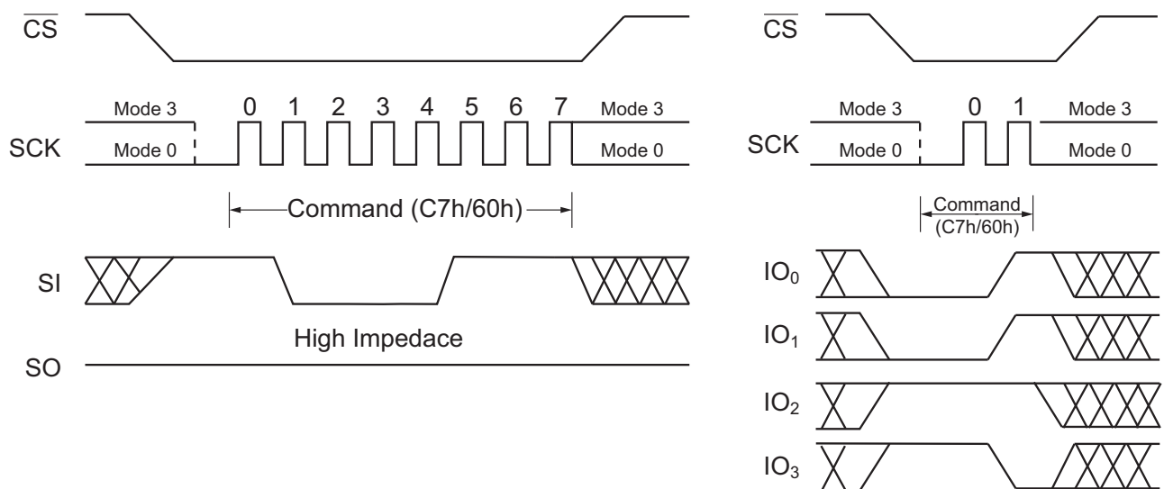
Figure 77. Chip Erase Command for SPI Mode (left) and QPI Mode (right)
