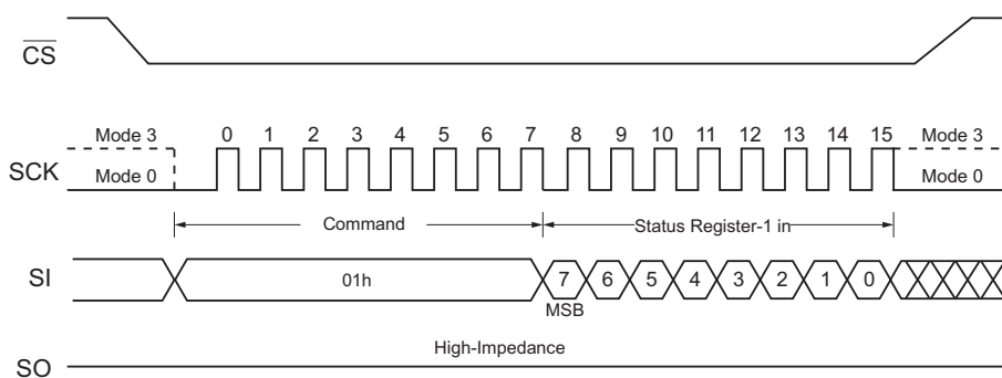
Figure 16. Write Status Register Diagram - 01h/31h/11h 1-byte (SPI Mode)
