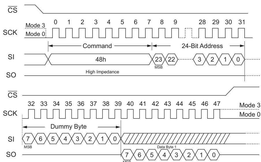
Figure 60. Read Security Register, SPI Mode
