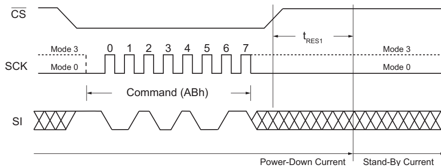
Figure 56. Release Power-Down Command (SPI Mode)
