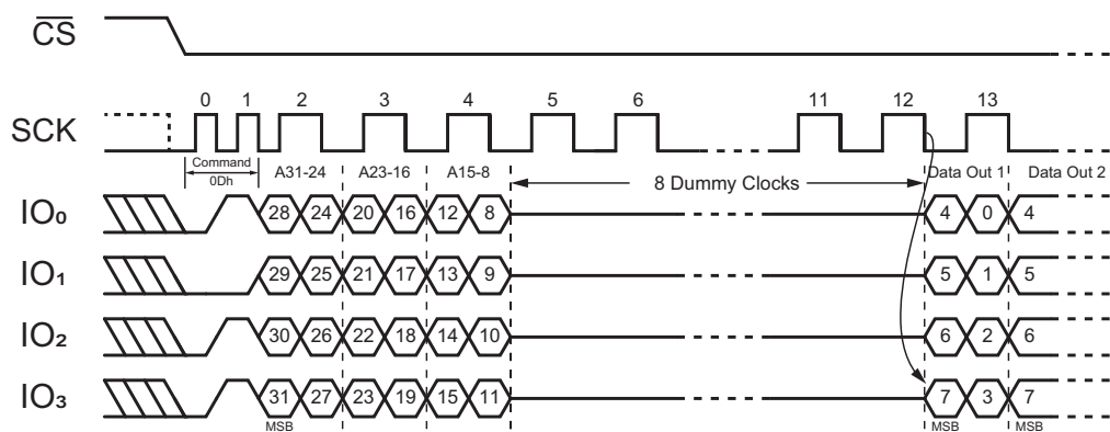
Figure 26. DTR Fast Read (QPI Mode)
