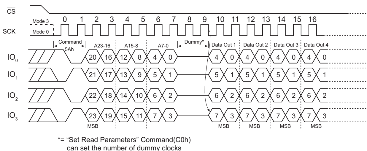
Figure 67. Read SFDP Register Command QPI Mode
