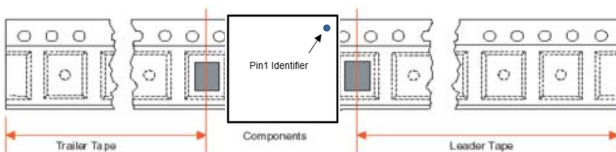
Figure 88. Tape and Reel Example Section
