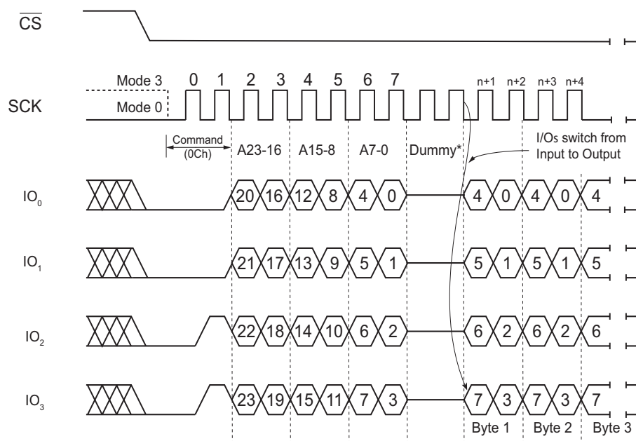
Figure 45. Burst Read with Wrap Command (QPI Mode)
