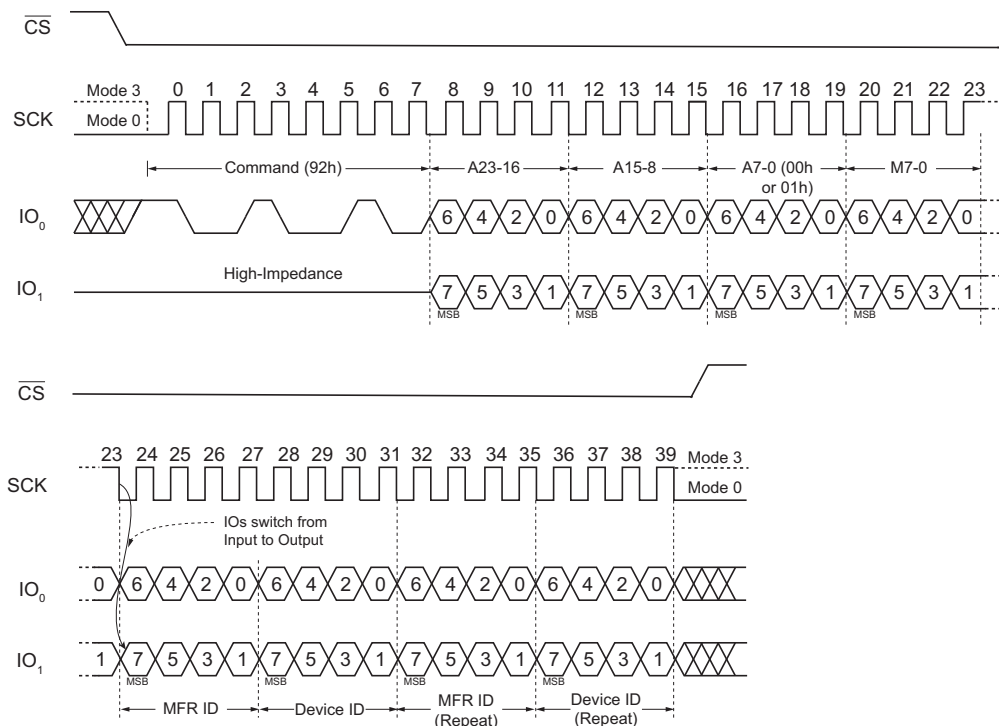
Figure 49. Read Dual Manufacturer/ Device ID Dual I/O Command (SPI Mode)
