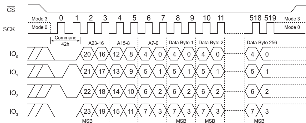
Figure 65. Program Security Register QPI Mode
