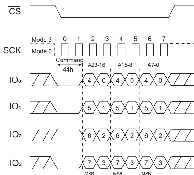
Figure 63. Erase Security Register QPI Mode
