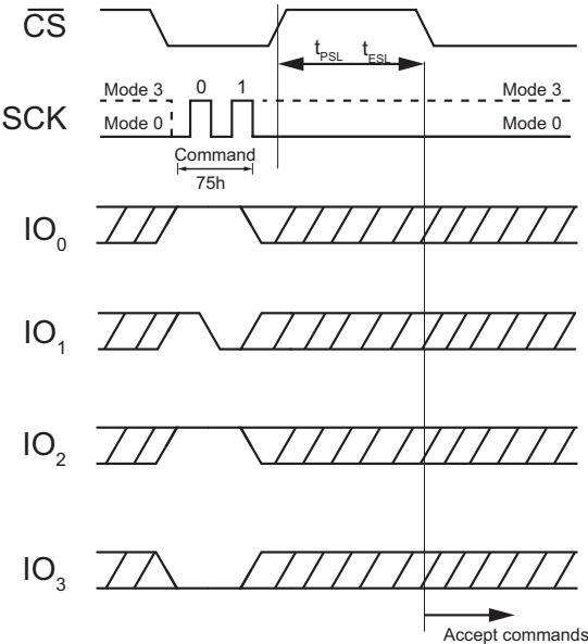
Figure 79. Erase Suspend Command (QPI Mode)
