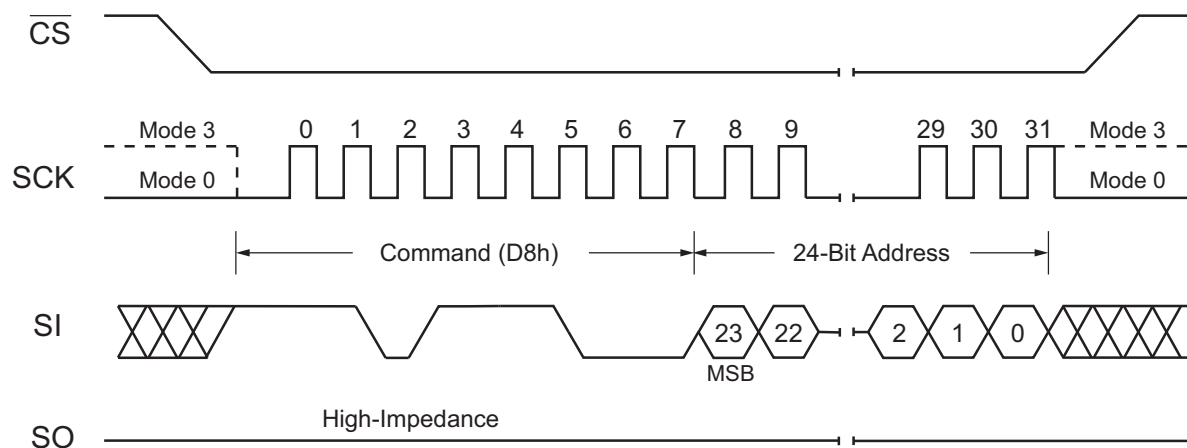
Figure 75. 64 kB Block Erase Command (SPI Mode)
