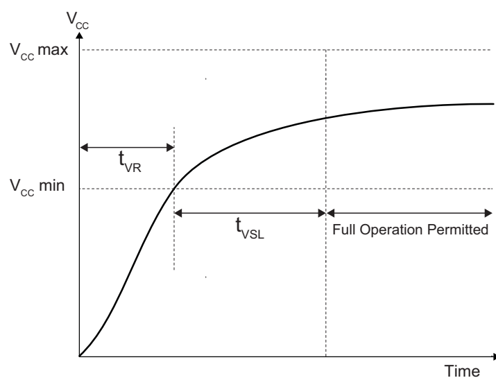
Figure 81. Power-up Timing and Voltage Levels
