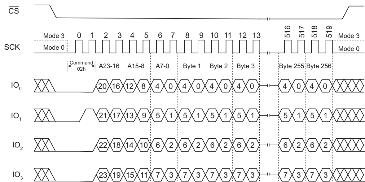
Figure 69. Page Program Command (QPI Mode)
