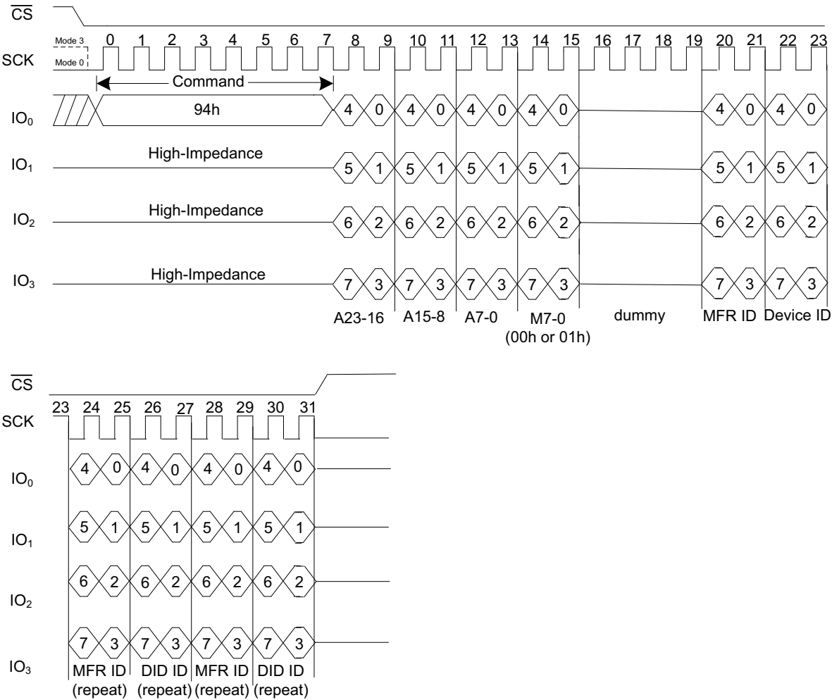
Figure 50. Read Quad Manufacturer/ Device ID Quad I/O Command (SPI Mode)
