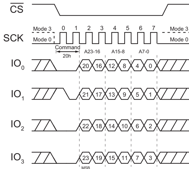
Figure 72. 4 kB Block Erase Command (QPI Mode)
