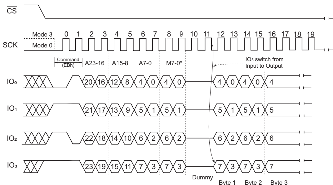
Figure 35. Fast Read Quad I/O Command (first time or after previous command has mode bits M5-4 not equal to 1,0; QPI mode)
