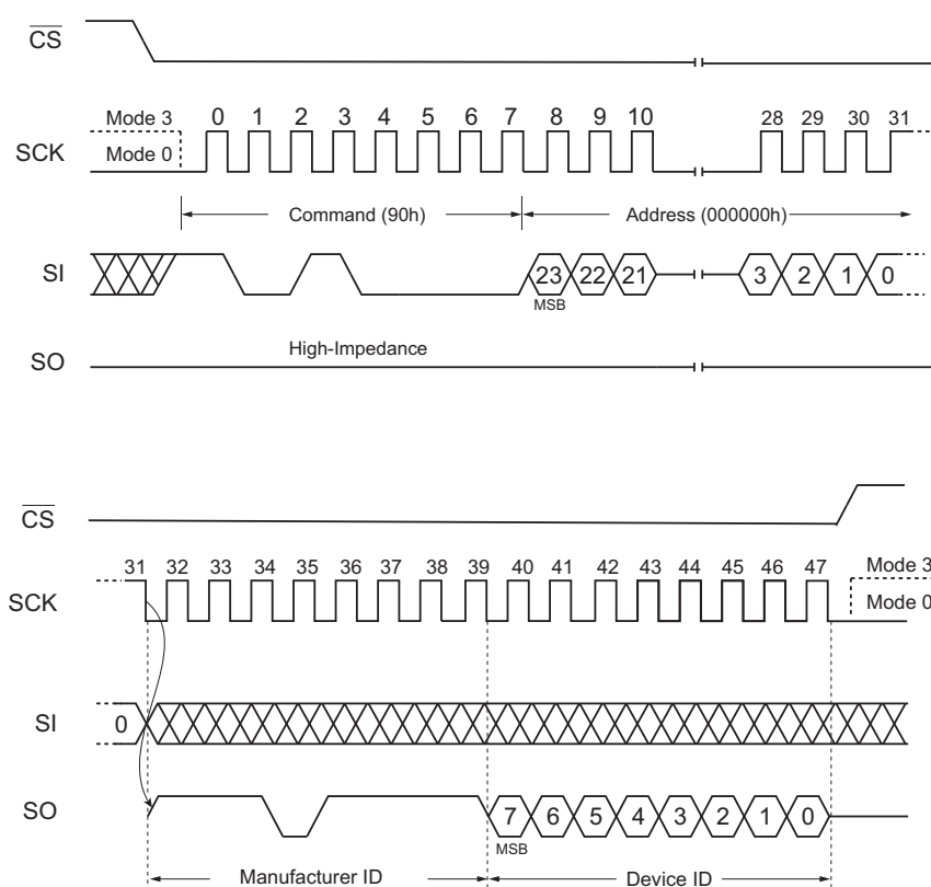
Figure 47. Read Manufacturer/ Device ID Command (SPI Mode)
