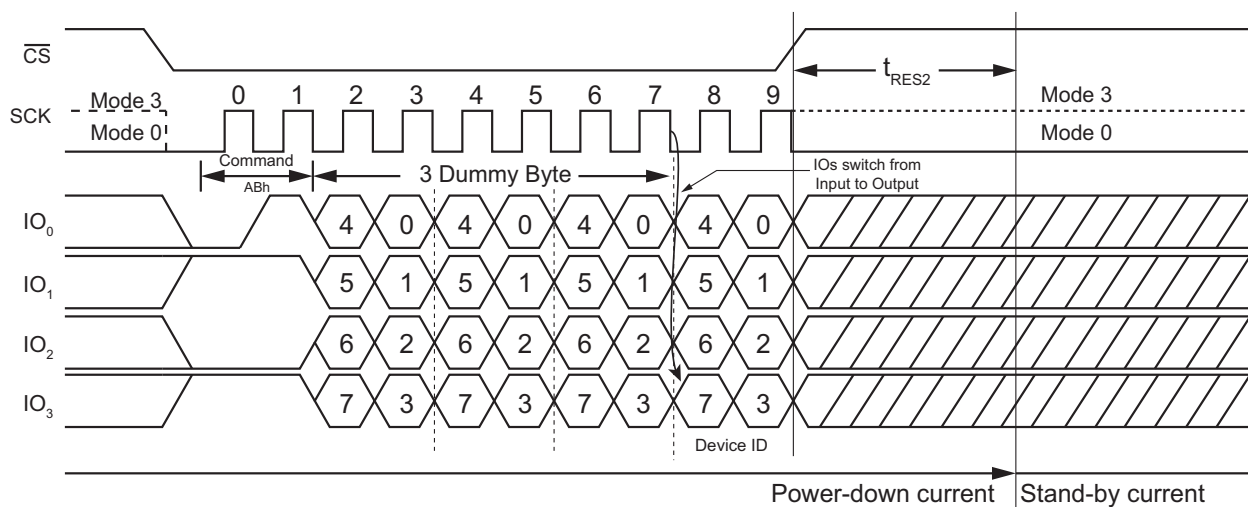
Figure 59. Release Power-Down / Device ID Command (QPI Mode)
