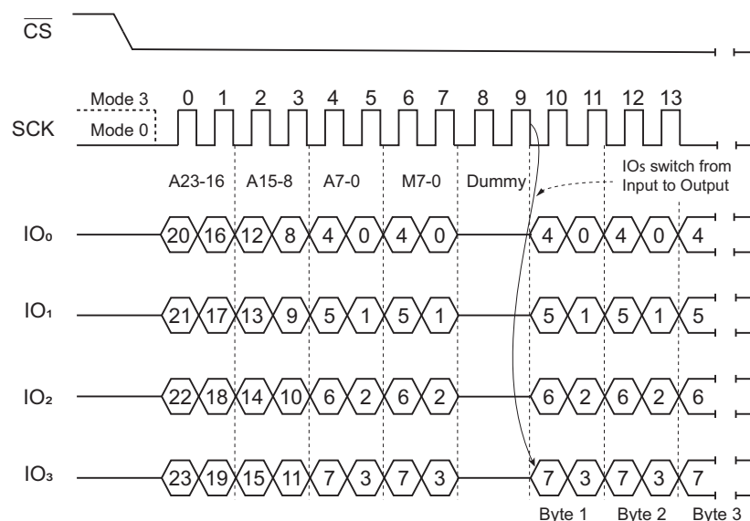
Figure 42. Word Read Quad I/O Command (Previous command set M5-4 = 1,0; SPI Mode)
