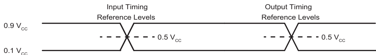
Figure 83. AC Measurement I/O Waveform
