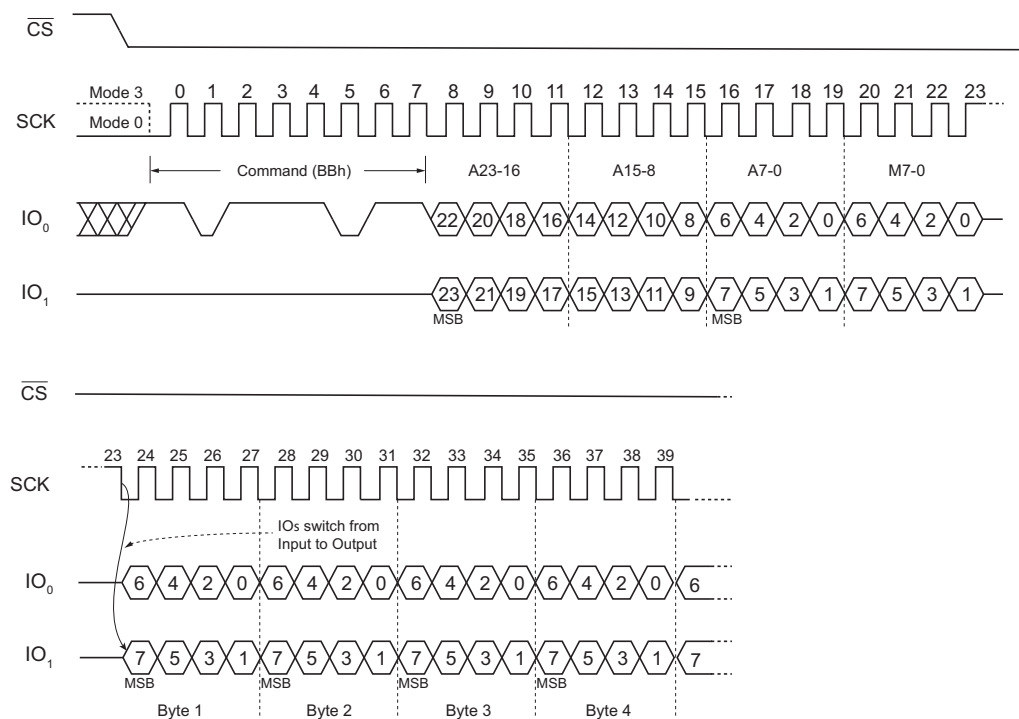
Figure 29. Fast Read Dual I/O Command (first time or after previous command has Mode bits M5-4 not equal to 1,0)
