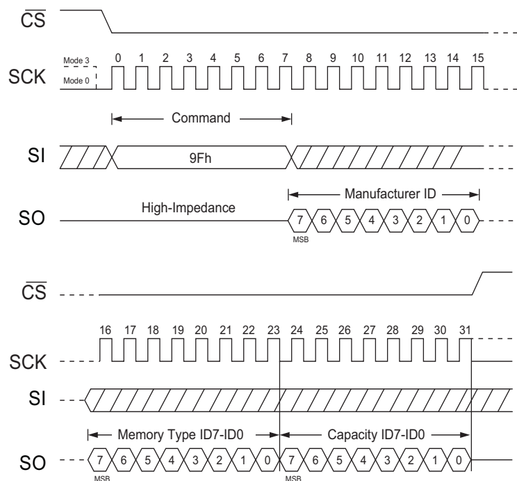
Figure 51. Read JEDEC ID Command (SPI Mode)
