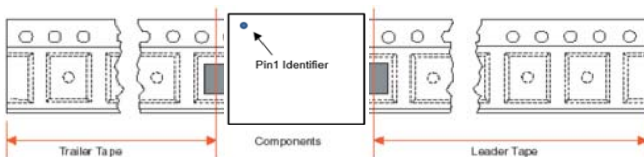
Figure 90. Tape and Reel Example Section
