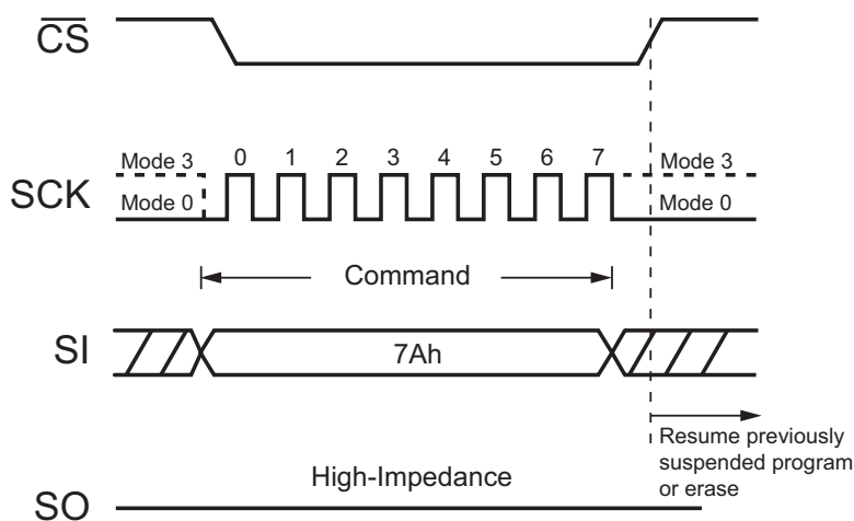
Figure 80. Erase / Program Resume Command (SPI Mode)
