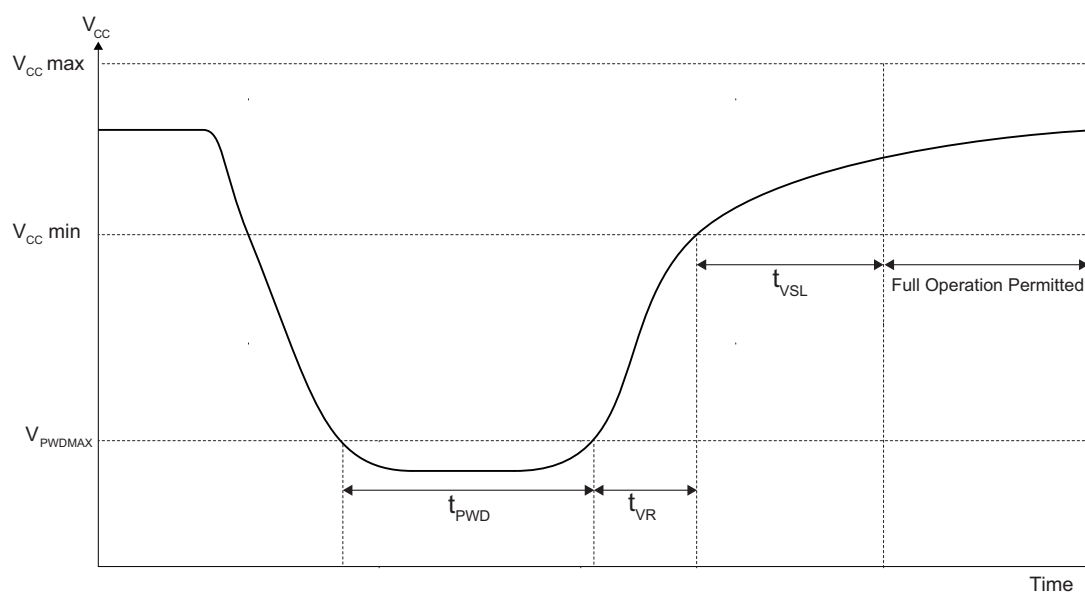
Figure 82. Power-up Timing After Brown-Out
