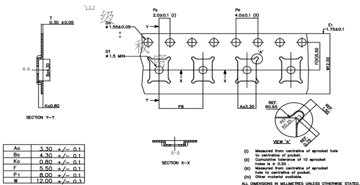
Figure 90. Tape and Reel Example Section
