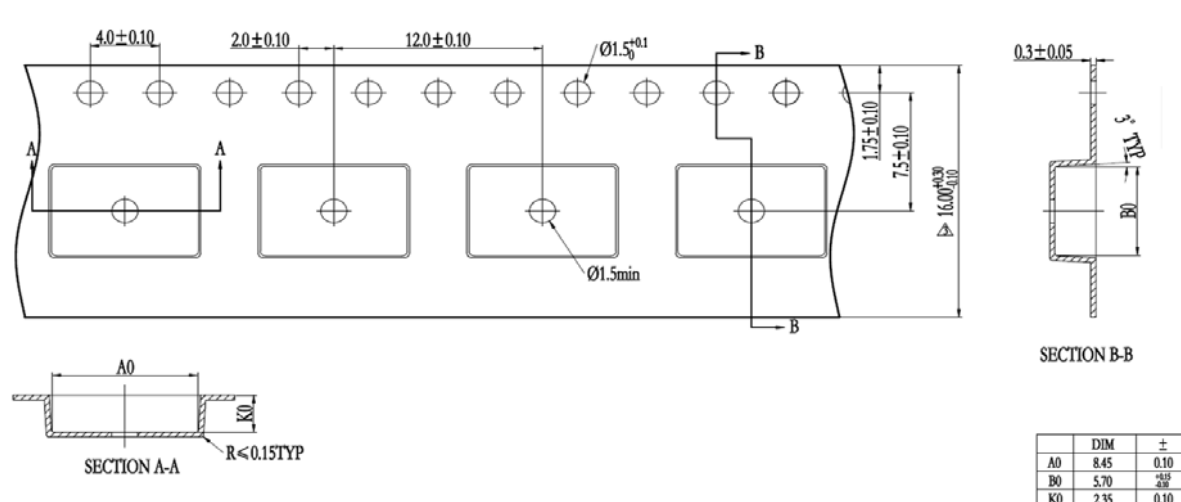
Figure 86. Tape and Reel Example Section
