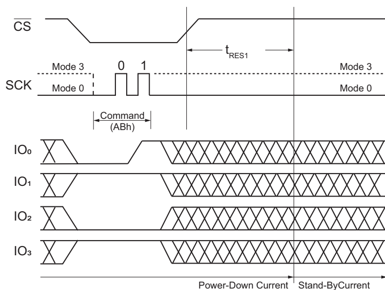
Figure 57. Release Power-Down Command (QPI Mode)
