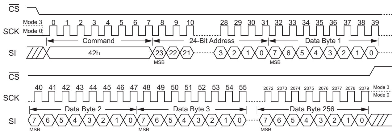
Figure 64. Program Security Register SPI Mode
