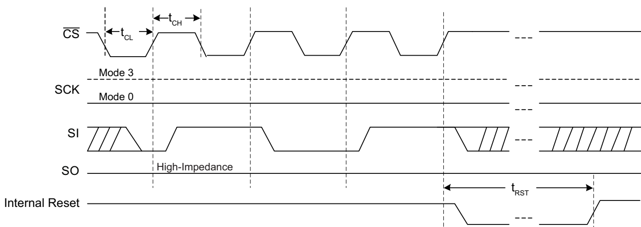
Figure 8. JEDEC Standard Hardware Reset
