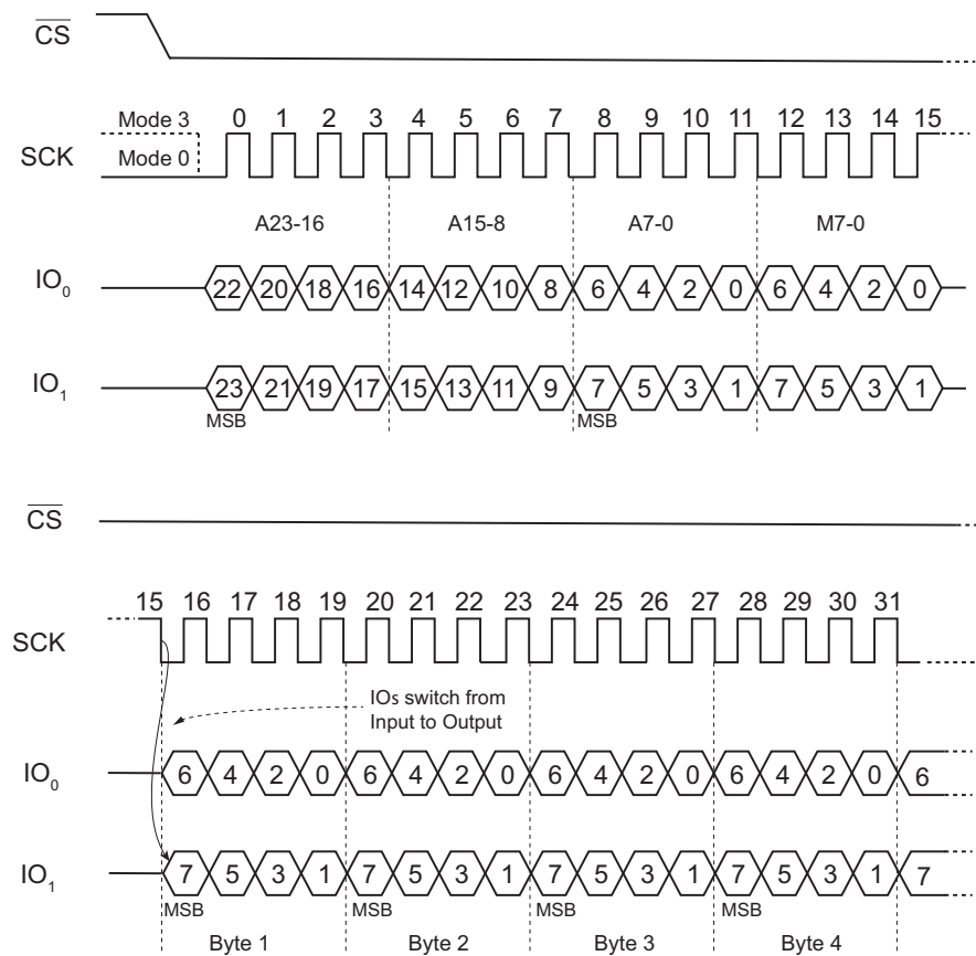
Figure 30. Fast Read Dual I/O Sequence Diagram (previous M5-4 = 1,0) SPI Mode Only
