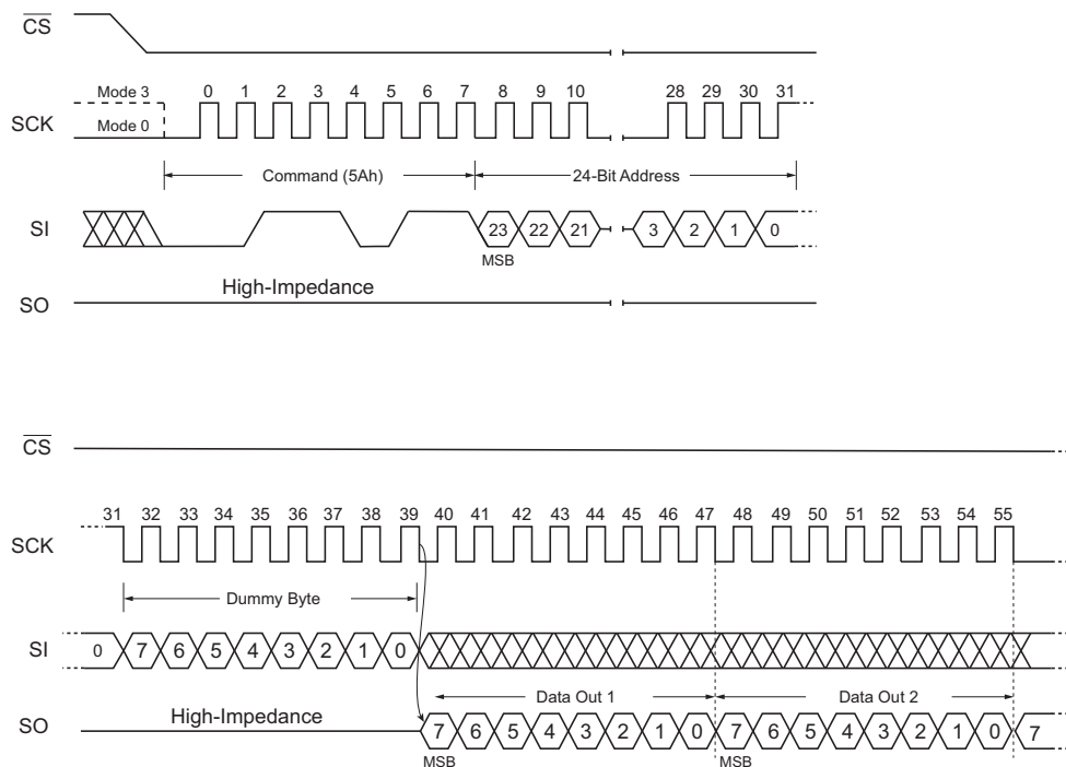
Figure 66. Read SFDP Register Command SPI Mode
