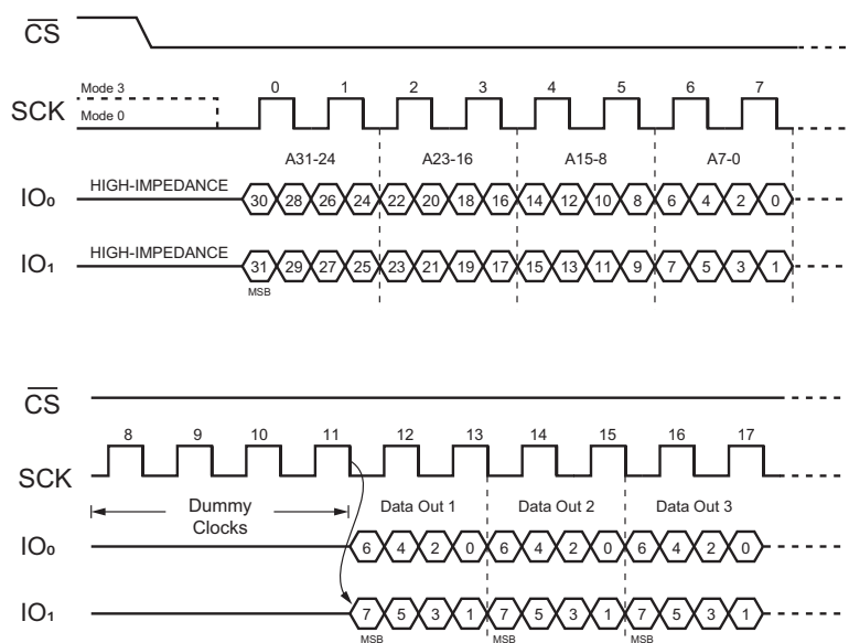
Figure 32. DTR Fast Read Dual I/O (SPI Mode only; Previous instruction set M5-4 = 10)
