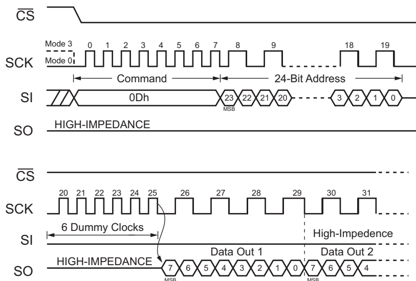
Figure 25. DTR Fast Read (SPI Mode)
