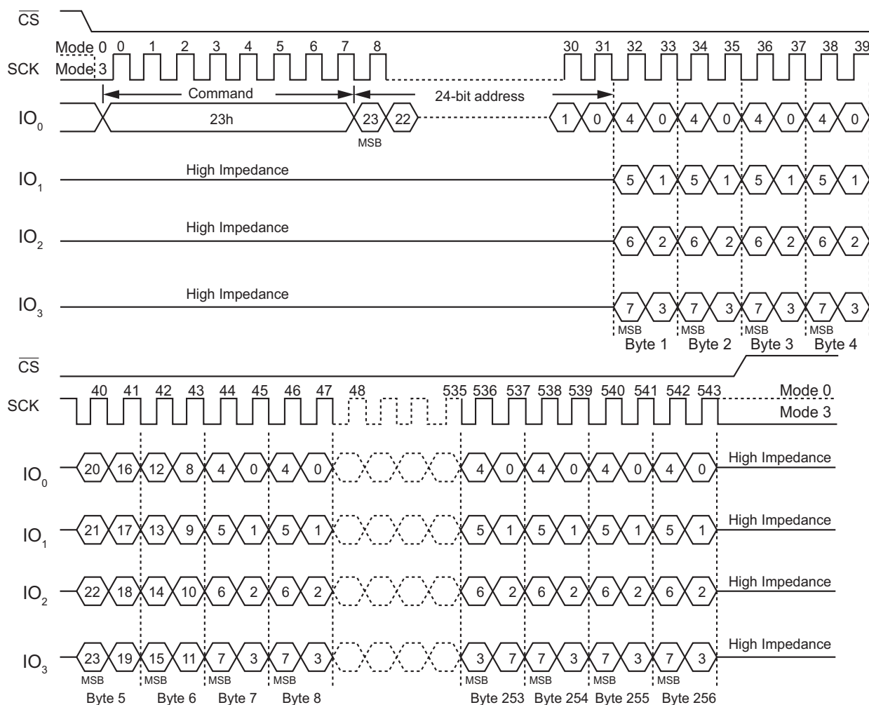
Figure 70. Quad Page Program Command (SPI mode)
