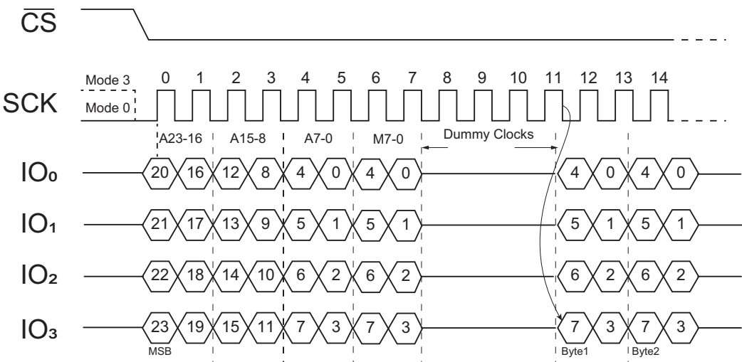
Figure 36. Fast Read Quad I/O Command (Initial command or previous M5-4 = 1,0; QPI mode)
