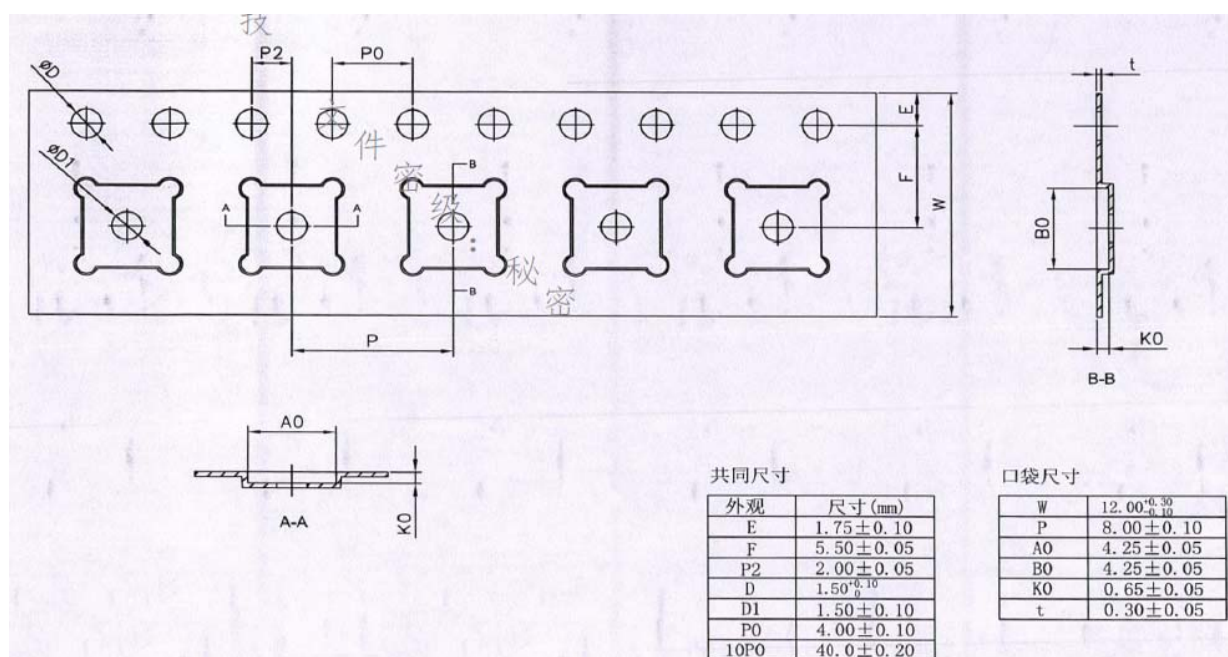
Figure 84. Tape and Reel Example Section
