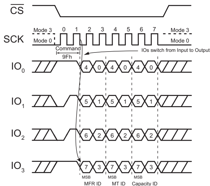
Figure 52. Read JEDEC ID Command (QPI Mode)
