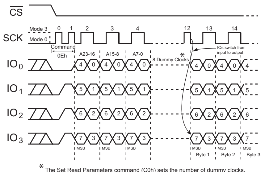
Figure 46. DTR Burst Read with Wrap Command (QPI Mode)
