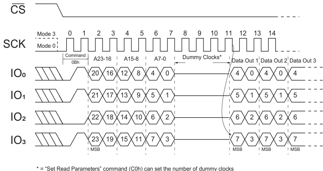
Figure 24. Fast Read Command (QPI Mode)
