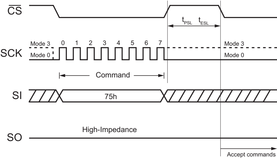
Figure 78. Erase Suspend Command (SPI Mode)
