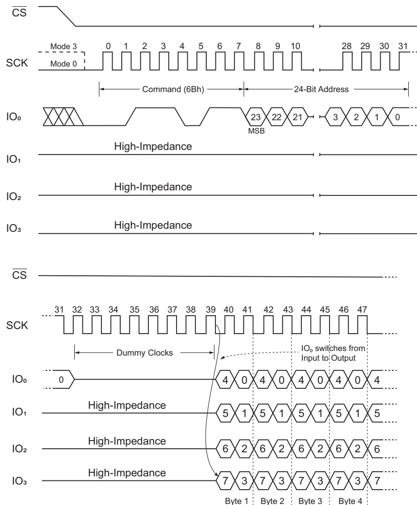
Figure 28. Fast Read Quad Output Command (SPI Mode)
