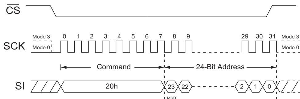
Figure 71. 4 kB Block Erase Command (SPI Mode)
