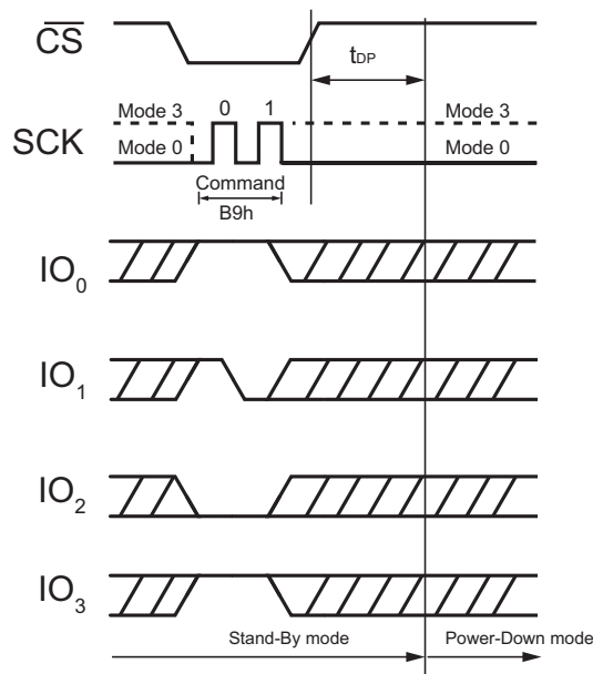
Figure 55. Deep Power-Down Command (QPI Mode)
