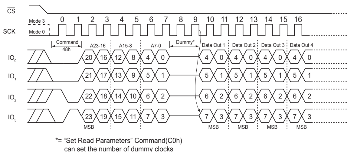
Figure 61. Read Security Register, QPI Mode
