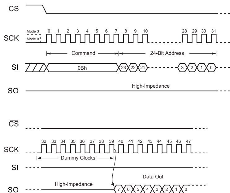
Figure 23. Fast Read Command (SPI Mode)
