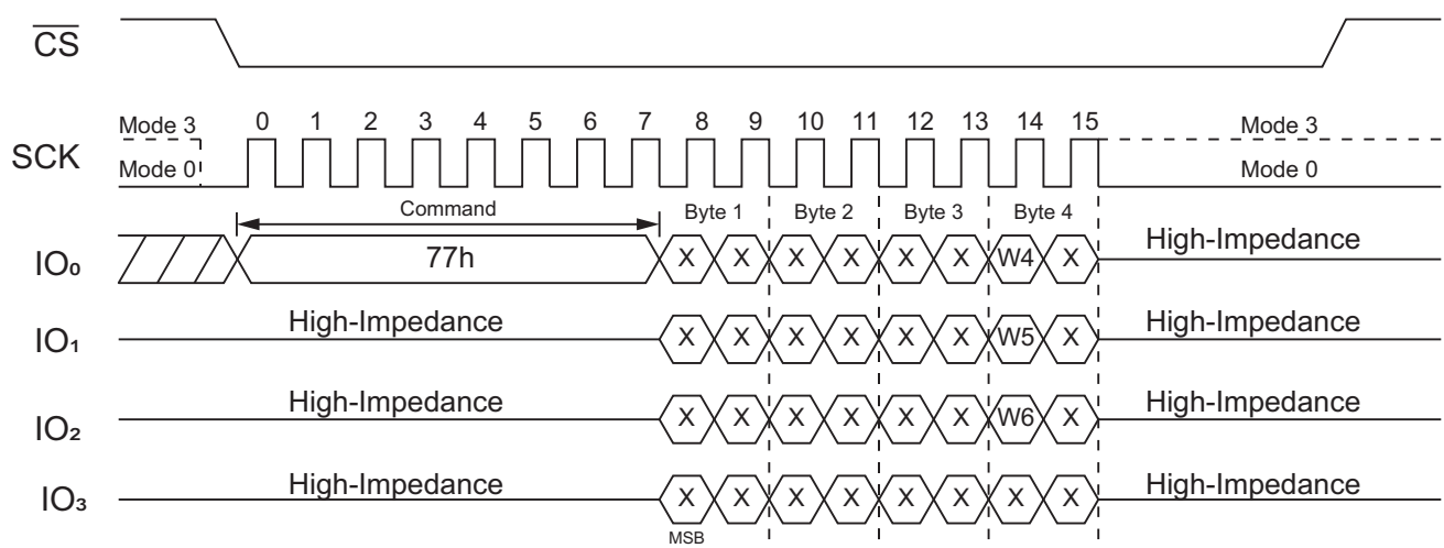
Figure 43. Set Burst with Wrap Command Sequence, SPI Only
