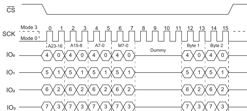
Figure 34. Fast Read Quad I/O Command (initial command or previous M5-4 = 1,0; SPI mode)
