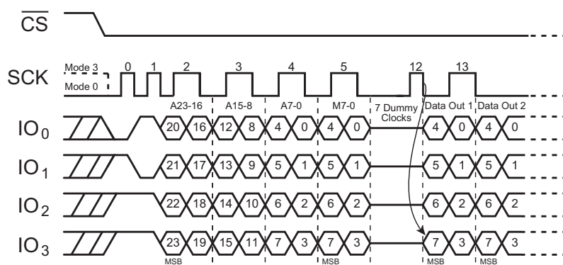
Figure 39. DTR Fast Read Quad I/O (QPI Mode; Initial instruction or previous M5-4 ≠ 1,0)
