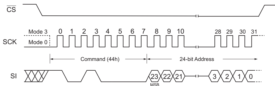
Figure 62. Erase Security Register SPI Mode
