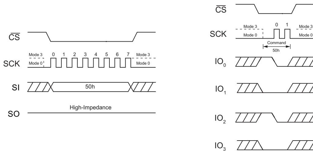
Figure 10. Write Enable for Volatile Status Register Command for SPI Mode (left) and QPI Mode (right)
