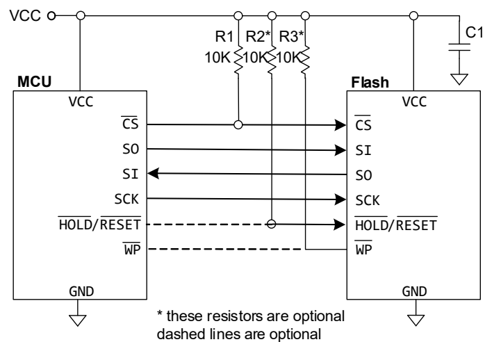
Figure 3. AT25SF0641C / AT25QF0641C Typical Application Block Diagram for SPI
