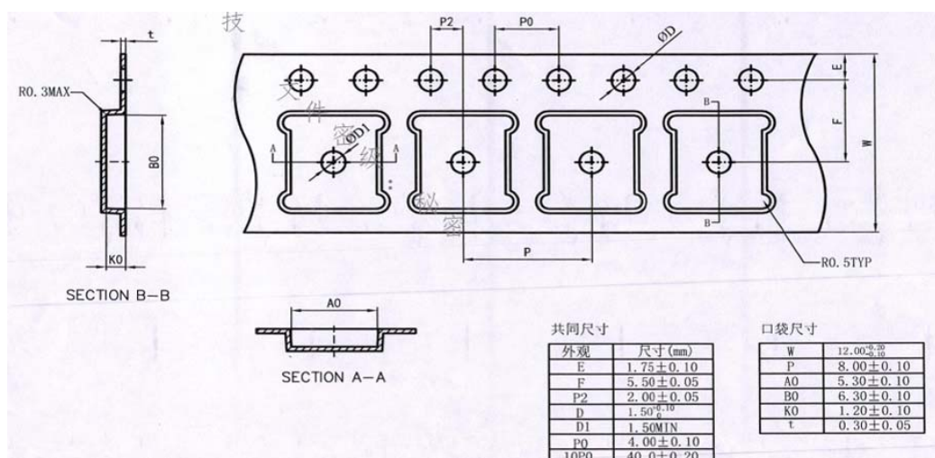
Figure 88. Tape and Reel Example Section
