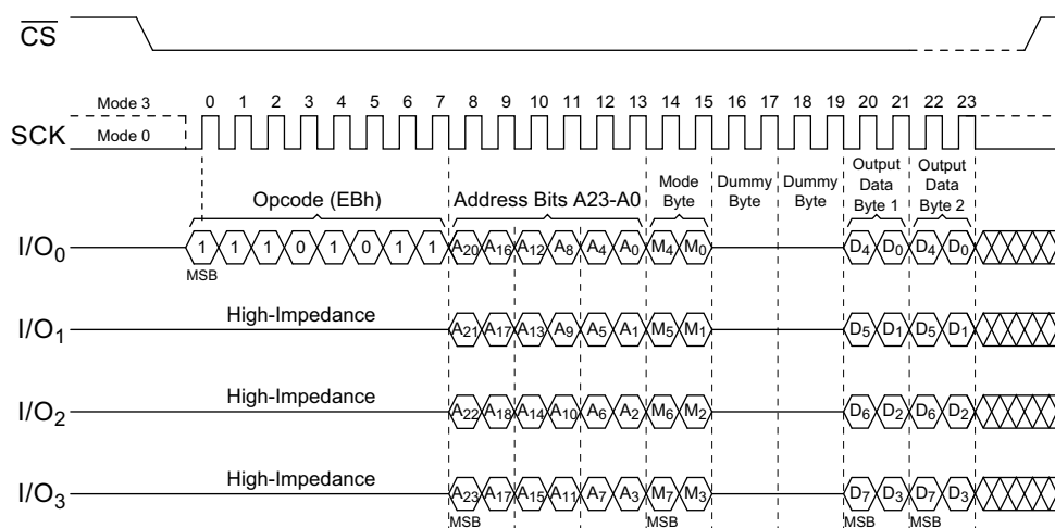
Figure 33. Fast Read Quad I/O Command (first time or after previous command has mode bits M5-4 not equal to 1,0; SPI Mode)
