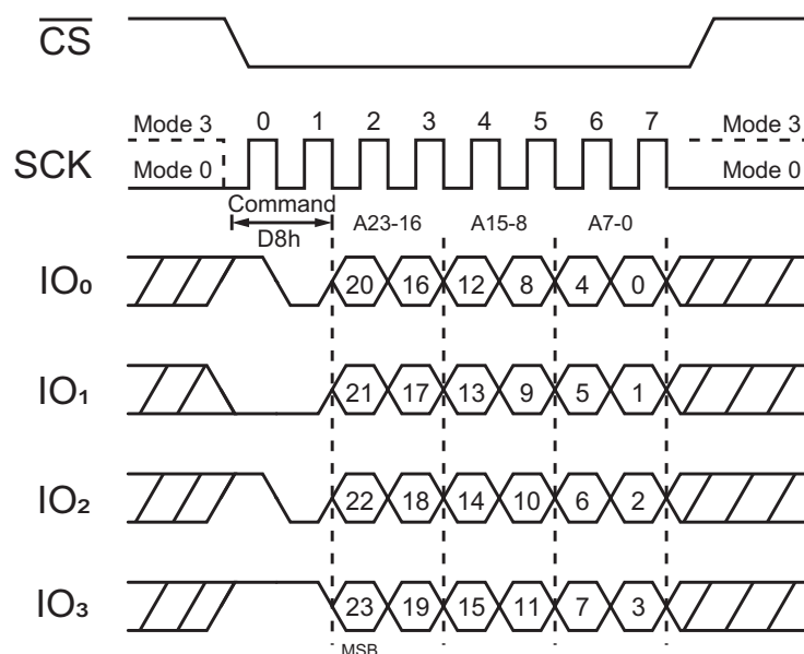
Figure 76. 64 kB Block Erase Command (QPI Mode)
