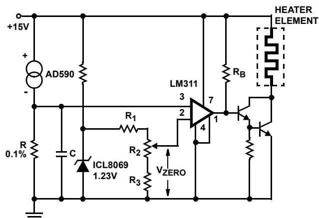
FIGURE 9. SINGLE SETPOINT TEMPERATURE CONTROLLER
