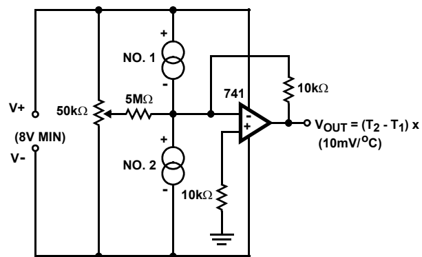
FIGURE 15. DIFFERENTIAL THERMOMETER
