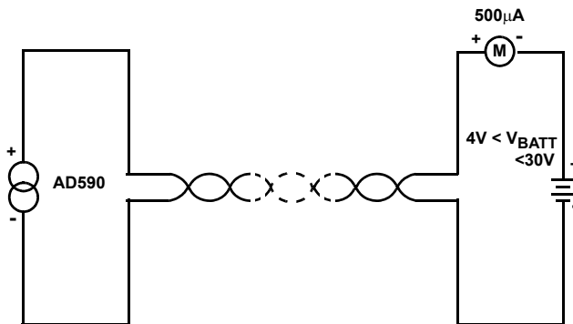
FIGURE 10. SIMPLEST THERMOMETER
