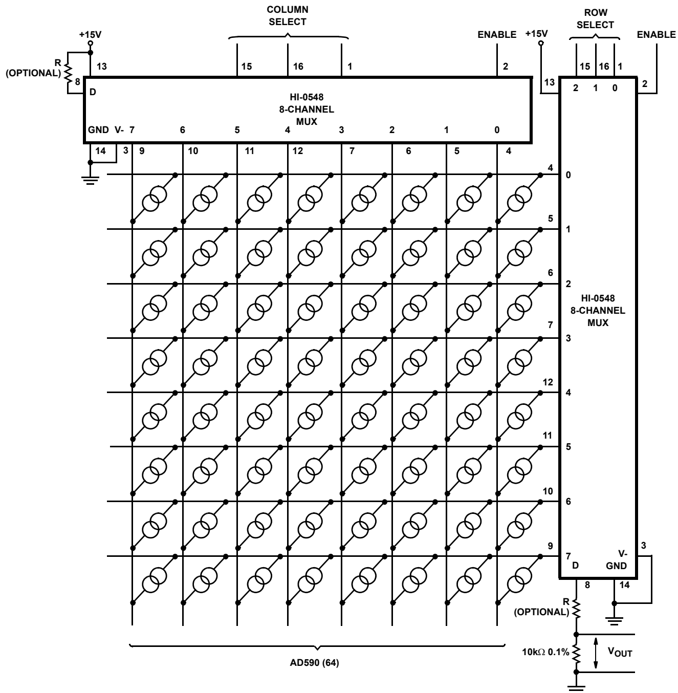
FIGURE 17. MULTIPLEXING SENSORS
