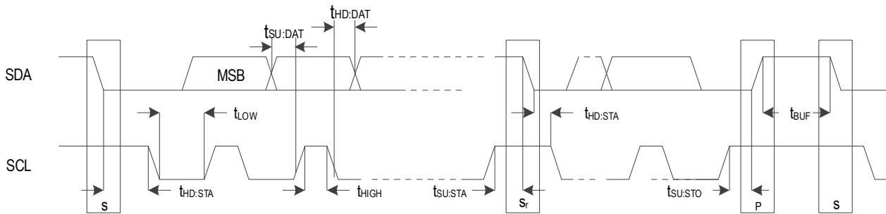
Figure 6. SMBus Slave Timing Diagram
