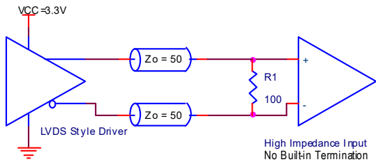
Figure 17. LVDS Termination
