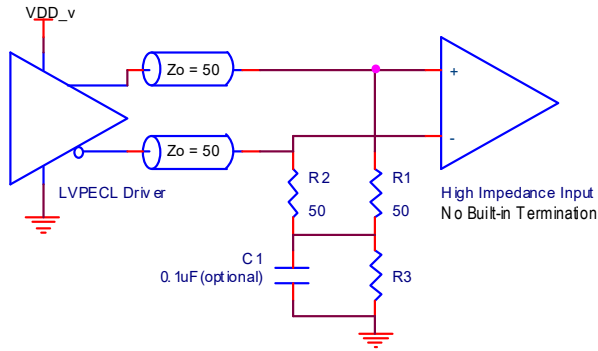
Figure 15. LVPECL Y-Termination
