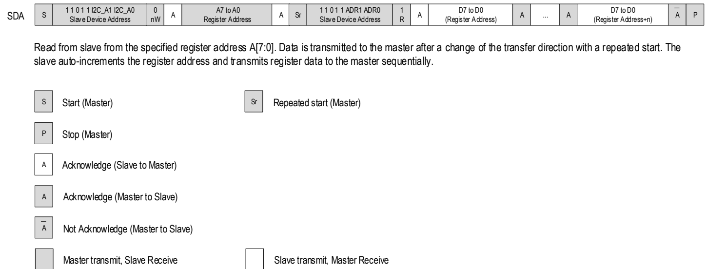
Figure 4. I 2 C Read Data (Slave Transmit, Master Receive) From Any Register Address
