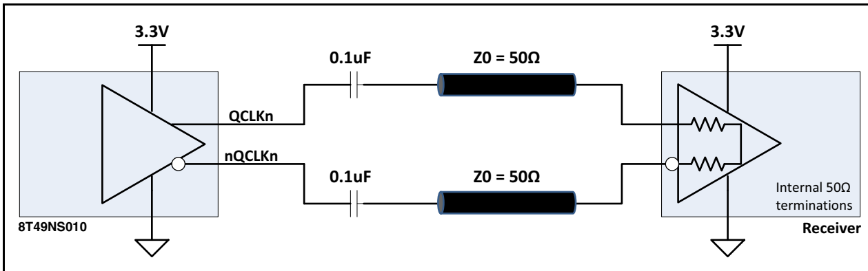
Figure 3F. AC Termination for FORMAT #2 used with an Input Clock Receiver with Internal 50\Omega Terminations.
