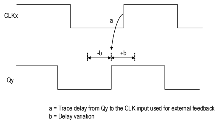
Figure 39. Input-Output Delay with External Feedback
