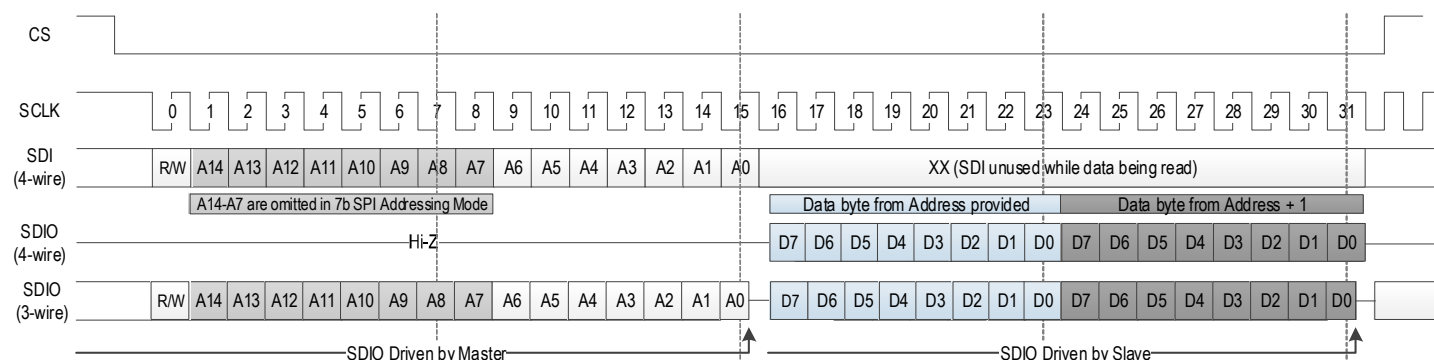
Figure 20. SPI Sequencing
