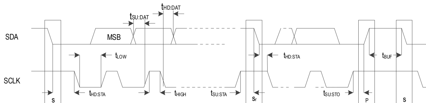
Figure 18. I 2 C Slave Timing Diagram
