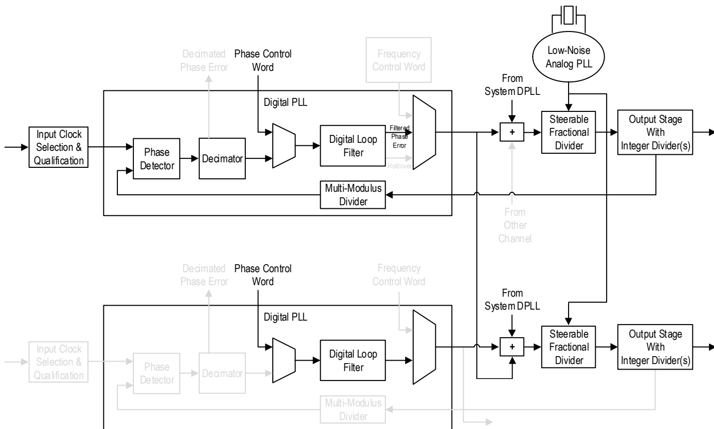
Figure 32. Combo Mode
