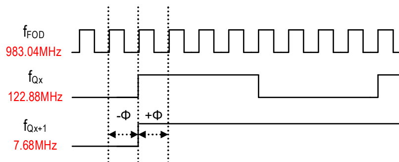
Figure 36. SYSREF Coarse Phase Adjustment
