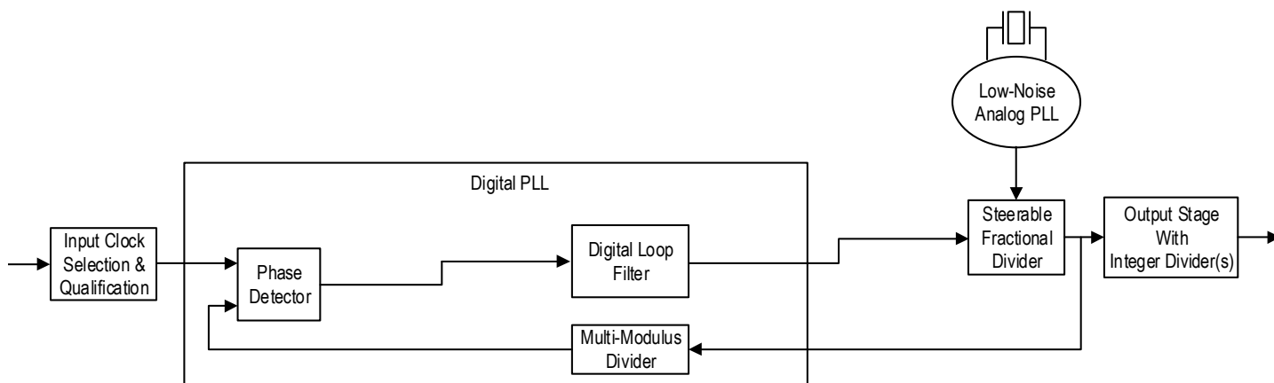
Figure 10. DPLL Channel
