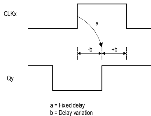
Figure 38. Input-Output Delay
