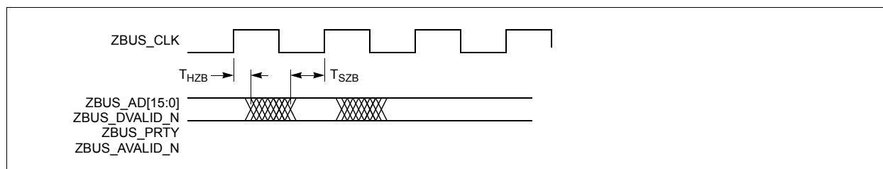
Figure 2 89TSF552 ZBus Interface Input Timing
