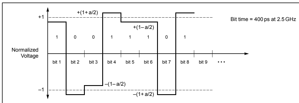
Figure 5 Output with Pre-Emphasis
