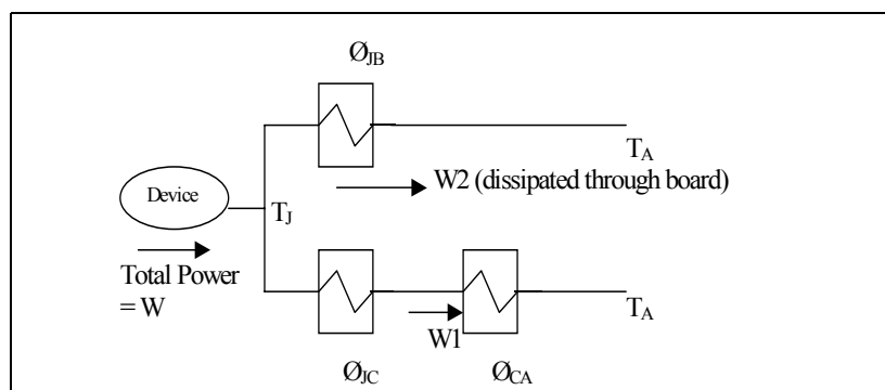
Figure 7 89TSF552 Thermal Circuit
