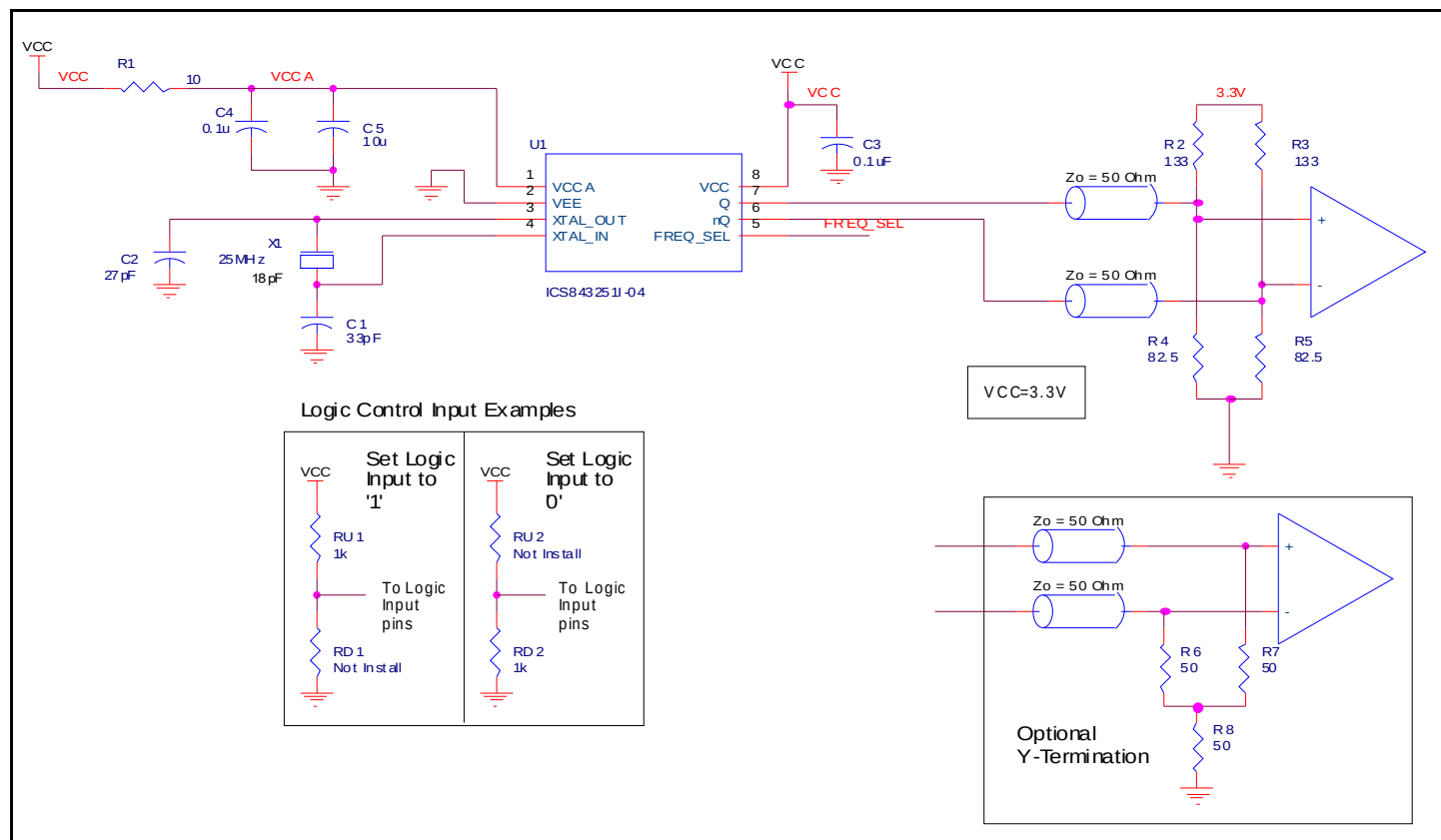
Figure 5. 843251-04 Schematic Example
