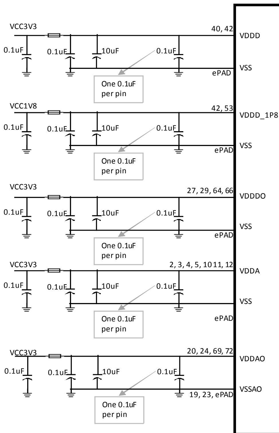
Figure 24. 82P33813 Power Decoupling Scheme
