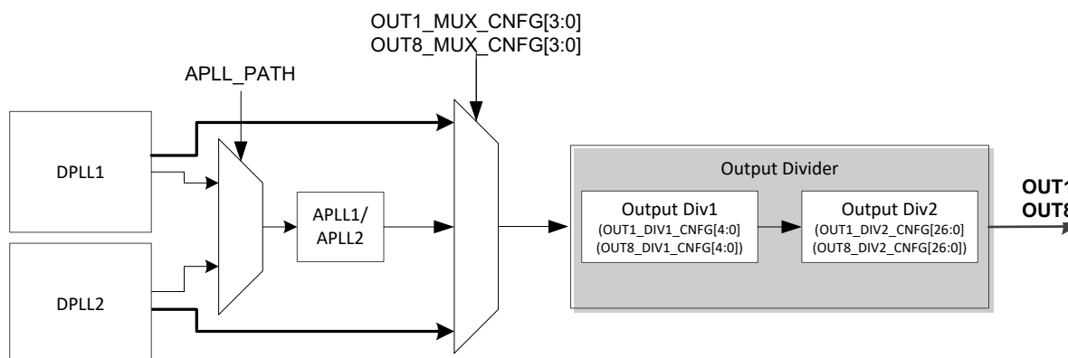
Figure 13. OUT1 and OUT8 output dividers
