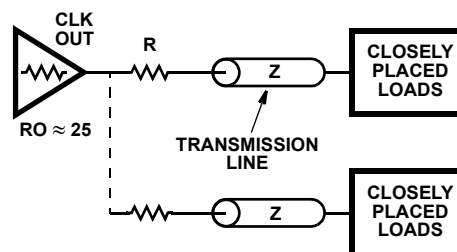
FIGURE 2. SERIES TERMINATION
