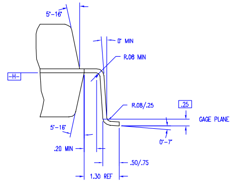
DETAIL B
