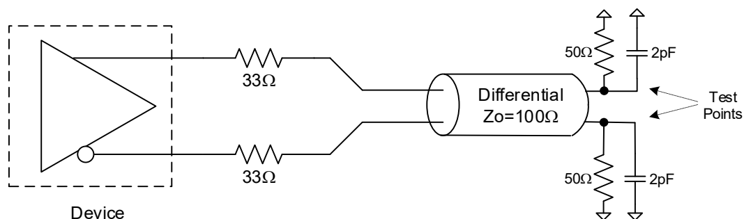
Figure 3. HCSL/LPHCSL Test Load
