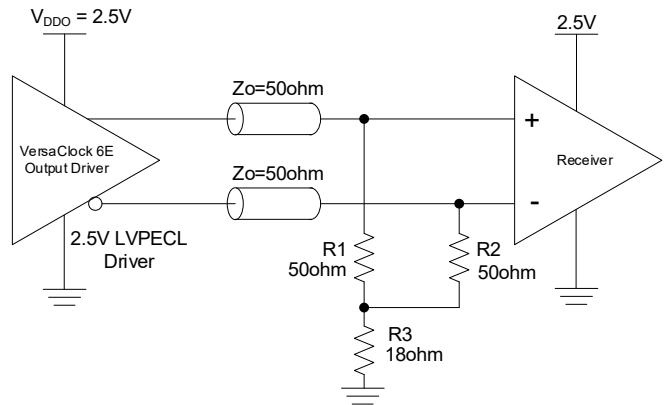
Figure 14. 2.5V LVPECL Output Termination
