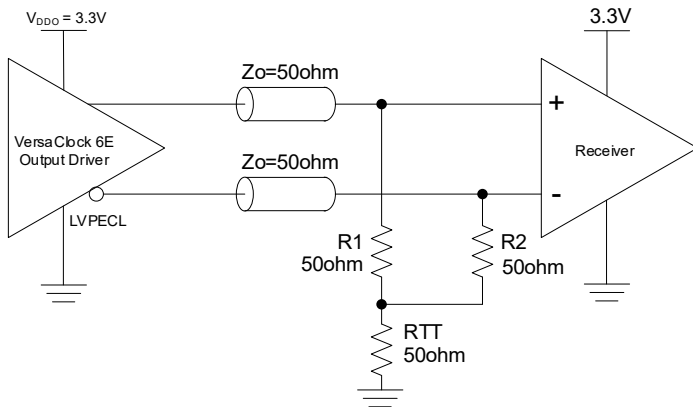
Figure 12. 3.3V LVPECL Output Termination
