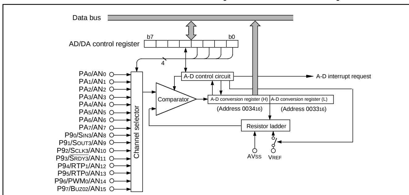
Fig. 61 Block diagram of A-D converter
