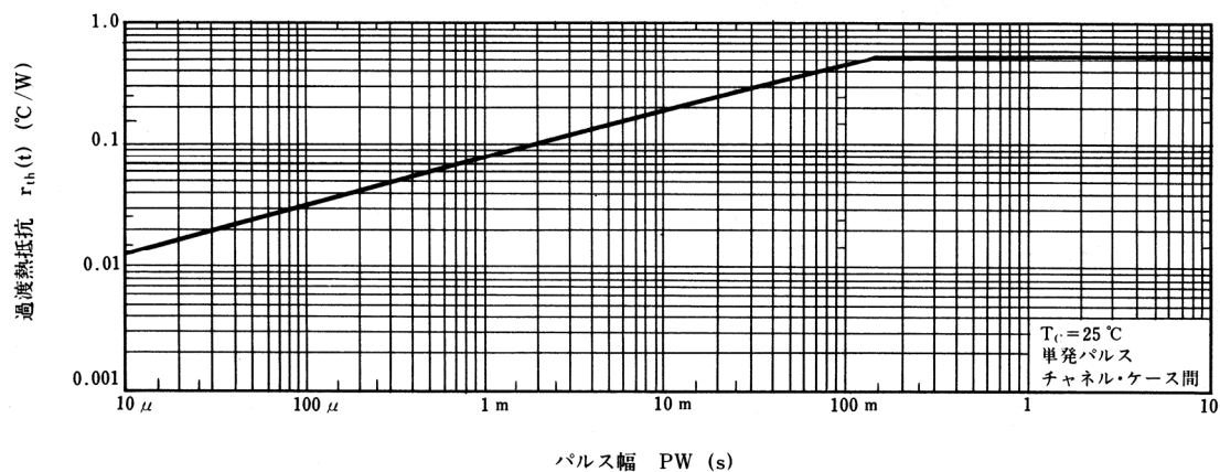
TRANSIENT THERMAL RESISTANCE vs. PULSE WIDTH
