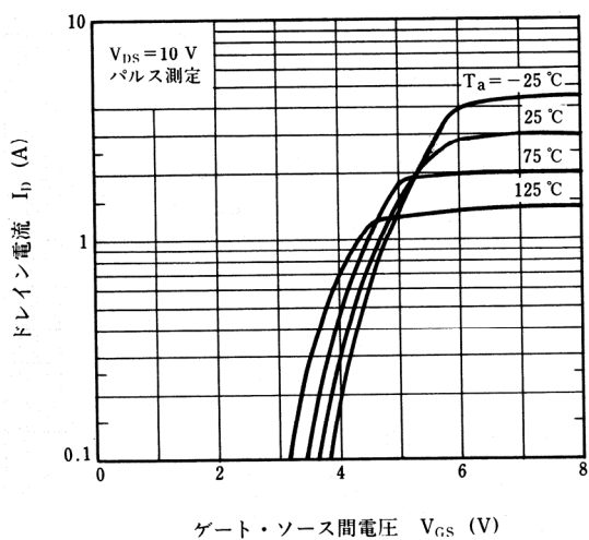
TRANSFER CHARACTERISTICS
