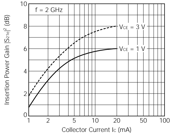
INSERTION GAIN vs. COLLECTOR CURRENT
