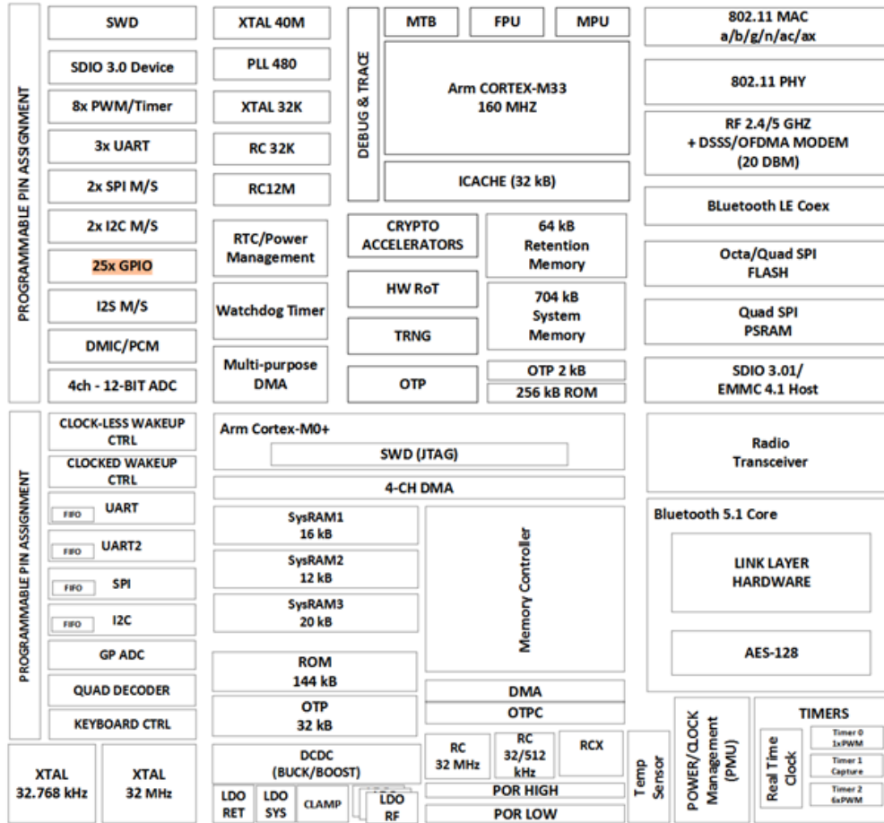
Figure 1. RA6W2 block diagram
