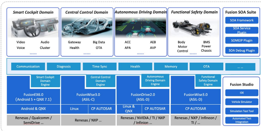
Create Digital Soft Chassis for Smart Car
