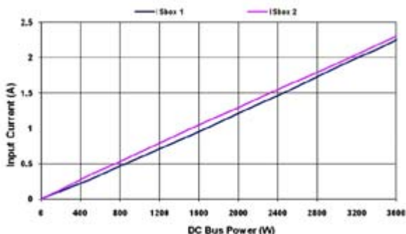
Figure 3: Current sharing <4% across the load range
