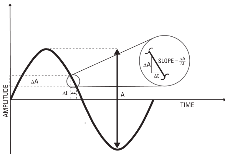
Figure 3: Aperture jitter in an ADC
