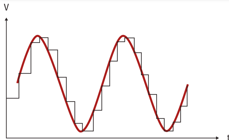
Figure 4: DAC output compared to ideal output (prior to reconstruction filter)
