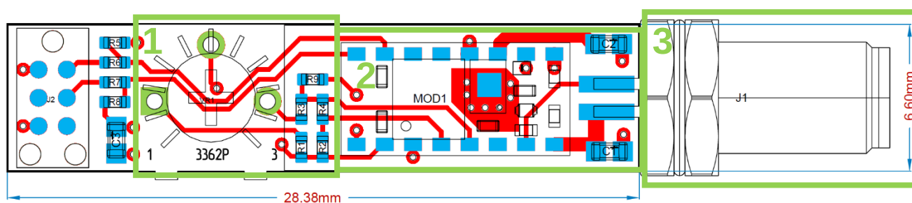
Figure 15. Reference Design 2: Base Board - Assembly View TOP
