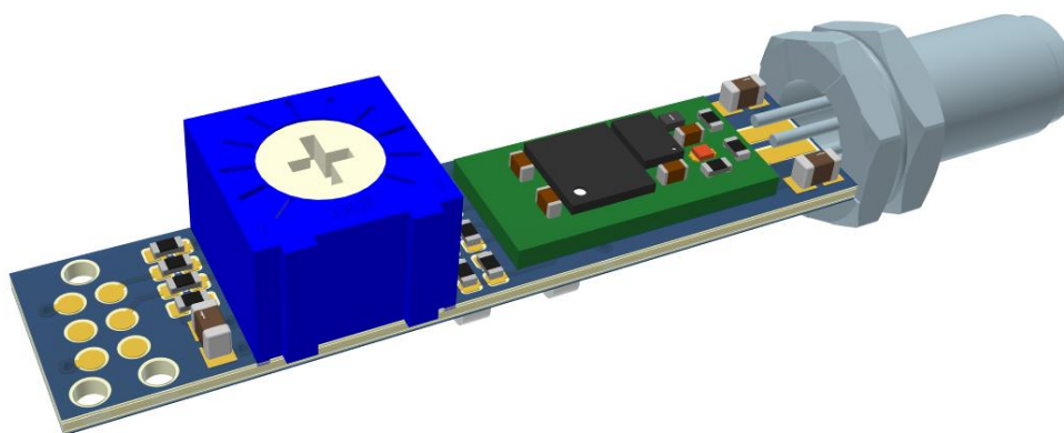
Figure 17. Reference Design 2: Base Board - 3D View
