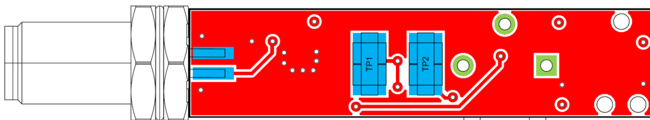
Figure 16. Reference Design 2: Base Board - Assembly View BOT
