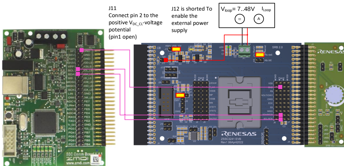
Figure 3. Current Loop HW Calibration Setup
