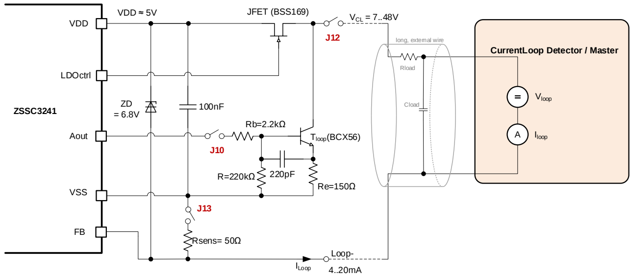
Figure 1. Current Loop Configuration
