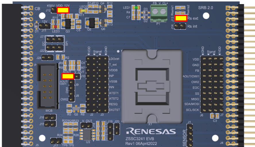
Figure 2. Evaluation Board Jumper Settings
