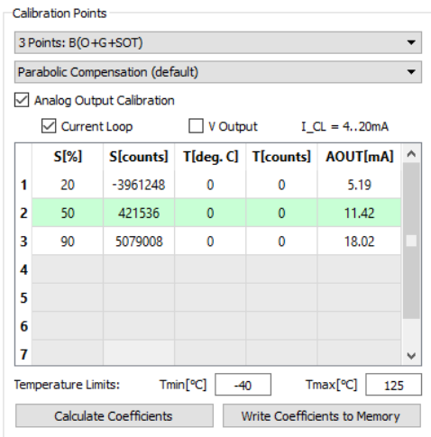
Figure 13. Current Loop 3-point Calibration Data
