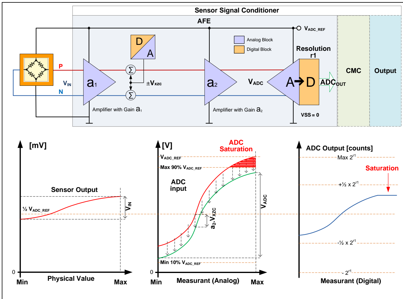
Figure 2.1 Analog Offset Compensation
