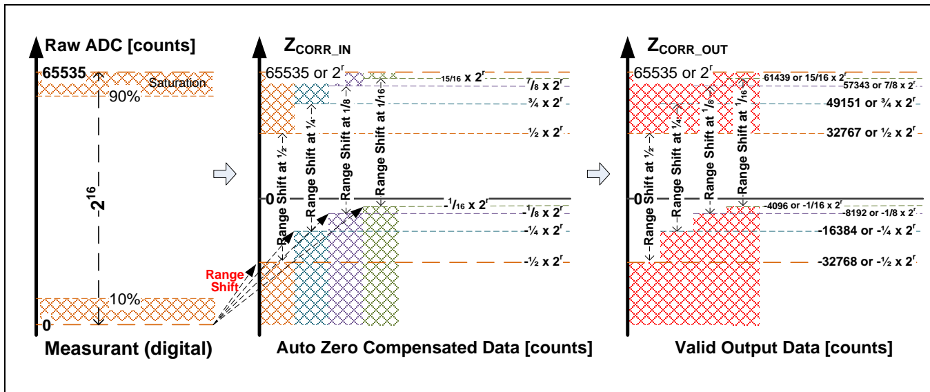
Figure 4.1 ADC Ranges
