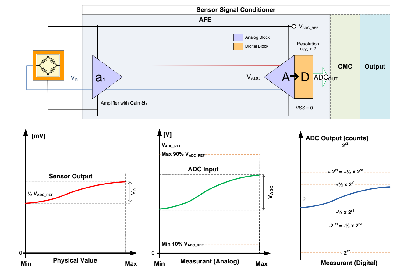
Figure 2.2 Range Zooming
