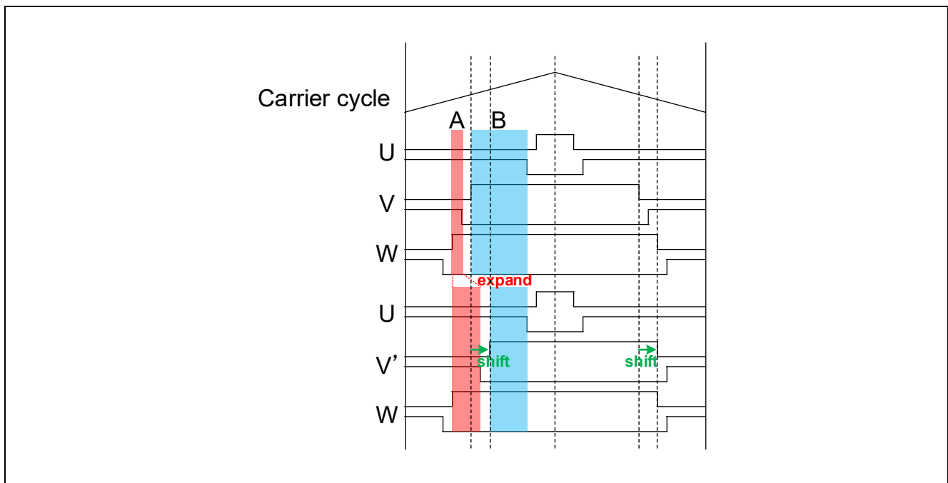
Figure 3-8 Duty adjustment
