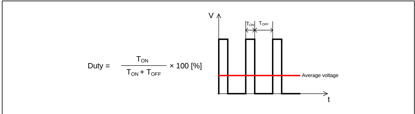
Figure 3-2 PWM control
