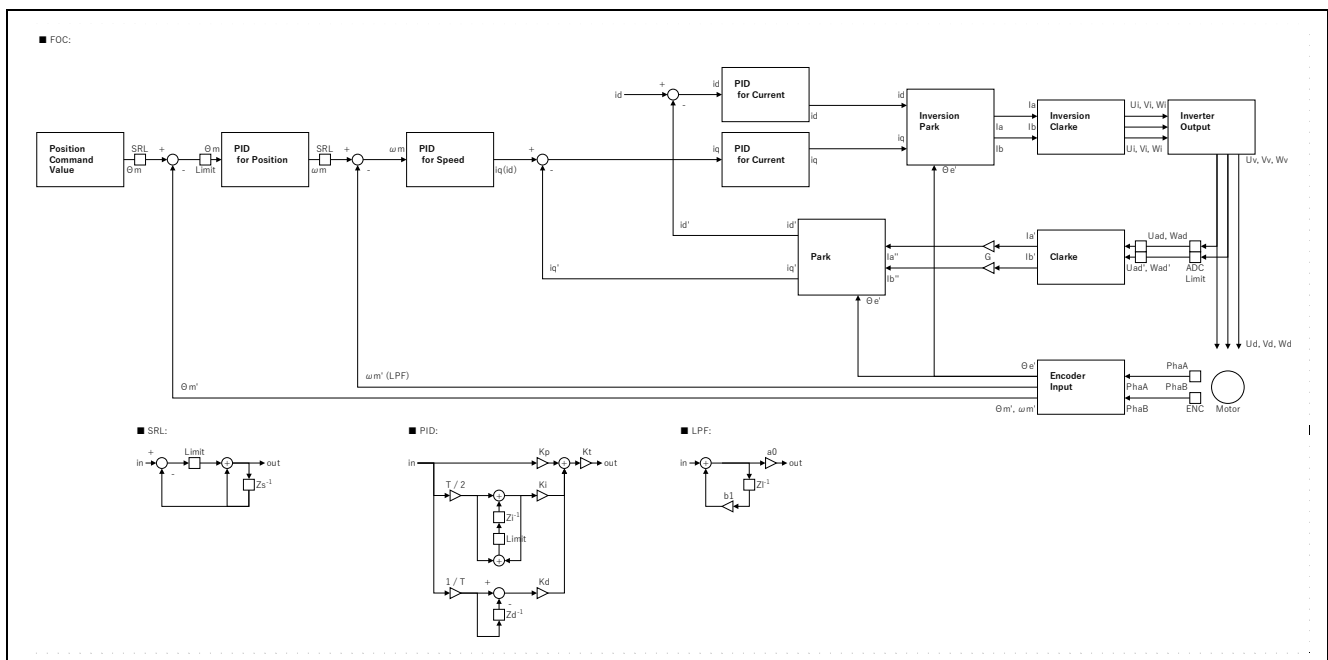
Figure 3-1 Vector control
