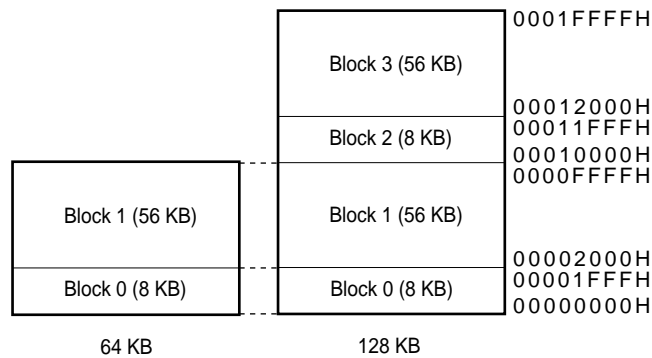
Figure 1-4. Flash Memory Configuration
