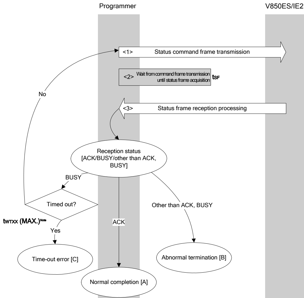
Status command processing sequence
