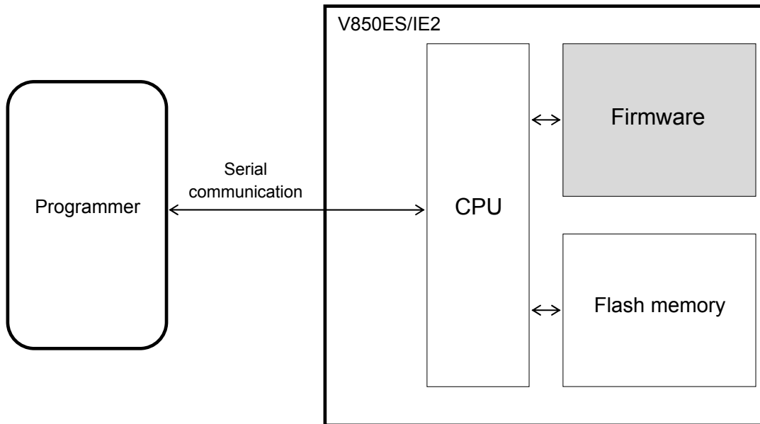
Figure 1-1. System Outline of Flash Memory Programming in V850ES/IE2
