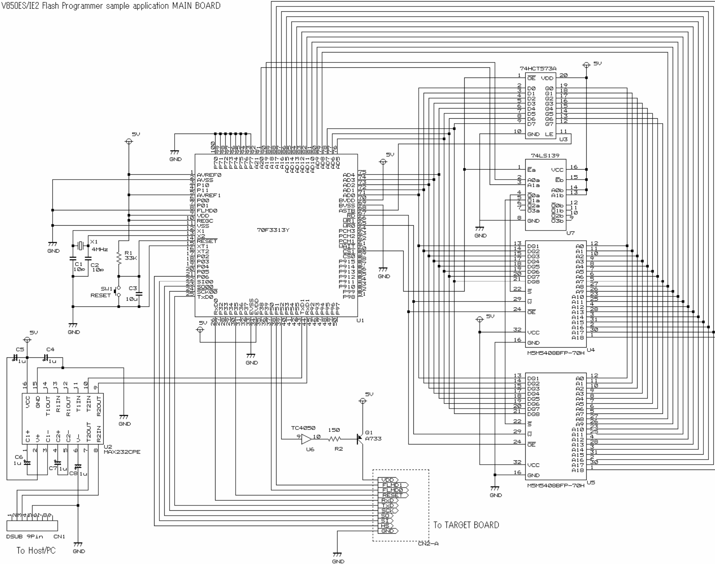
Figure A-1. Reference Circuit Diagram of Programmer and V850ES/IE2 (Main board)
