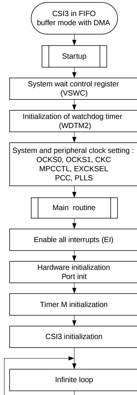
Figure 3-20: FIFO Buffer Transfer Flowchart with DMA
