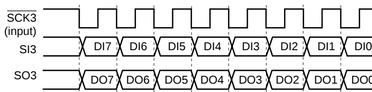
Figure 2-18: Slave Mode
