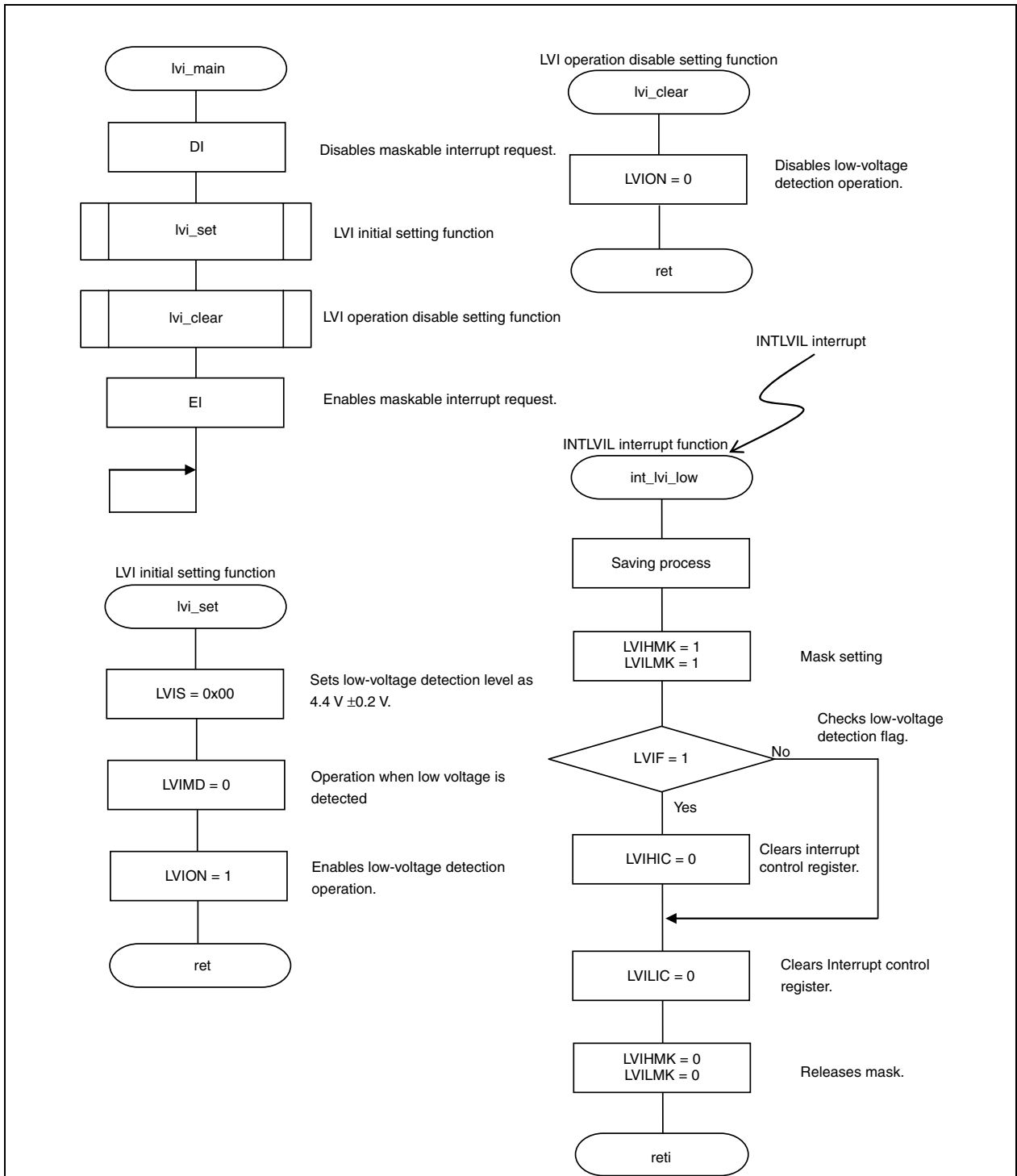
Figure 1-1. Low-Voltage Detection Interrupt Request Signal (1/2)
