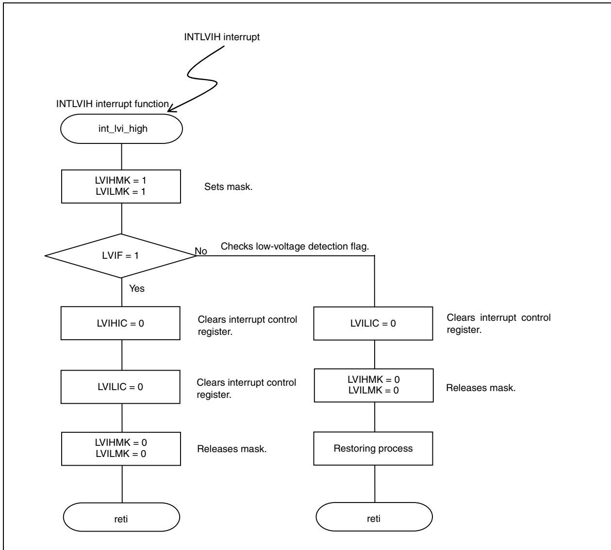
Figure 1-1. Low-Voltage Detection Interrupt Request Signal (2/2)
