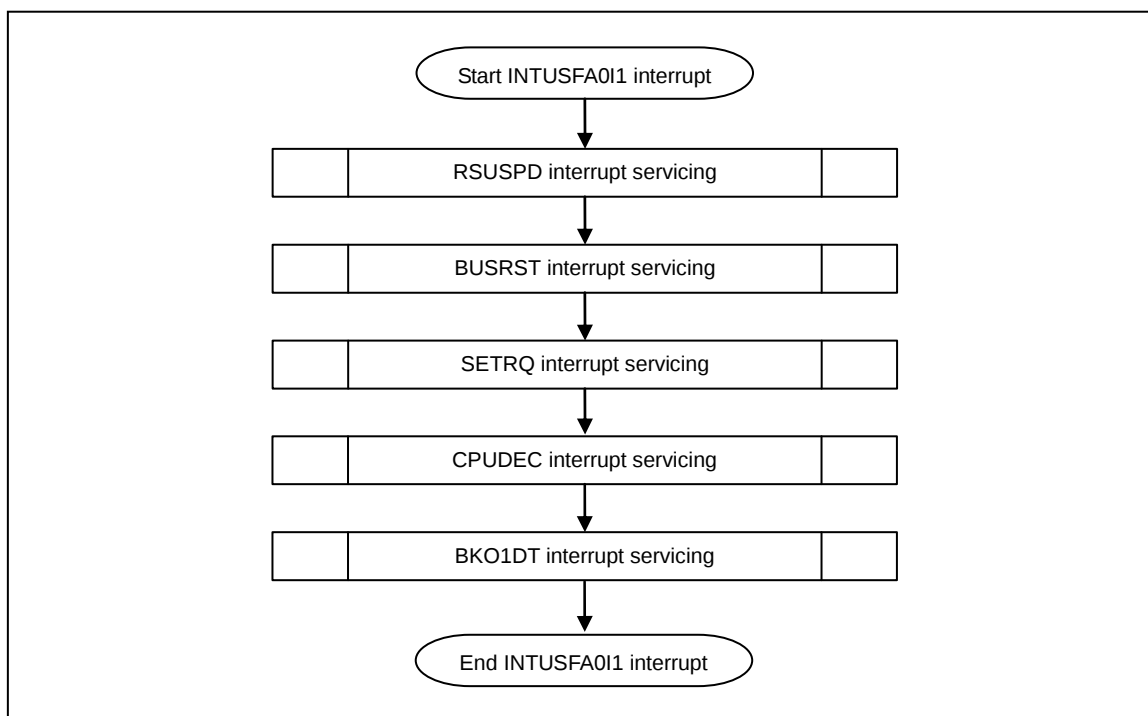
Figure 4-12. INTUSFA0I1 Interrupt Handler Processing Flowchart
