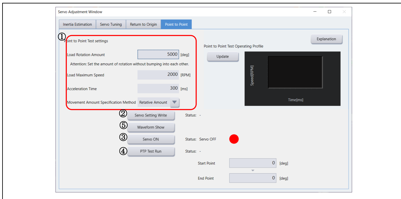
Figure 4-7 Operation window or “Point to point”
