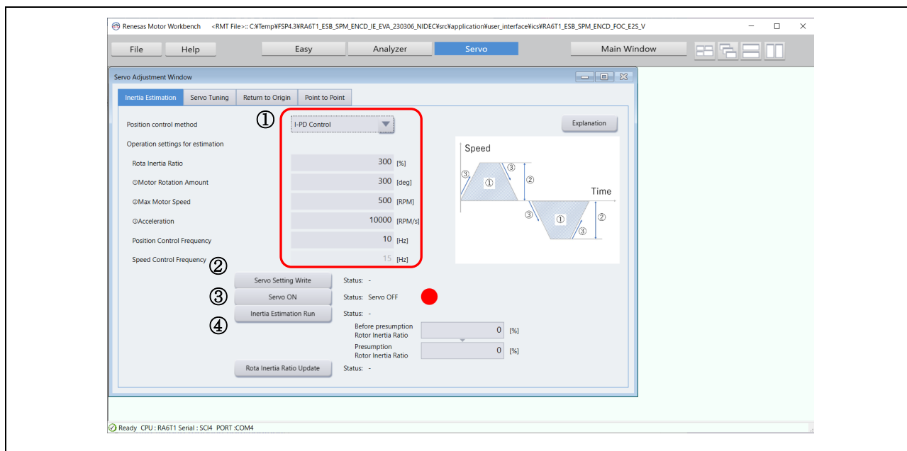
Figure 4-4 Operation window of “Inertia Estimation”
