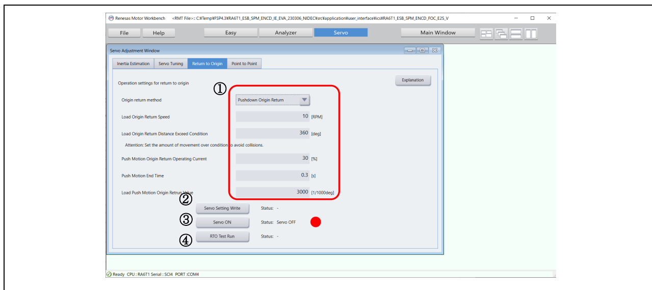
Figure 4-5 Operation window of “Return Origin”
