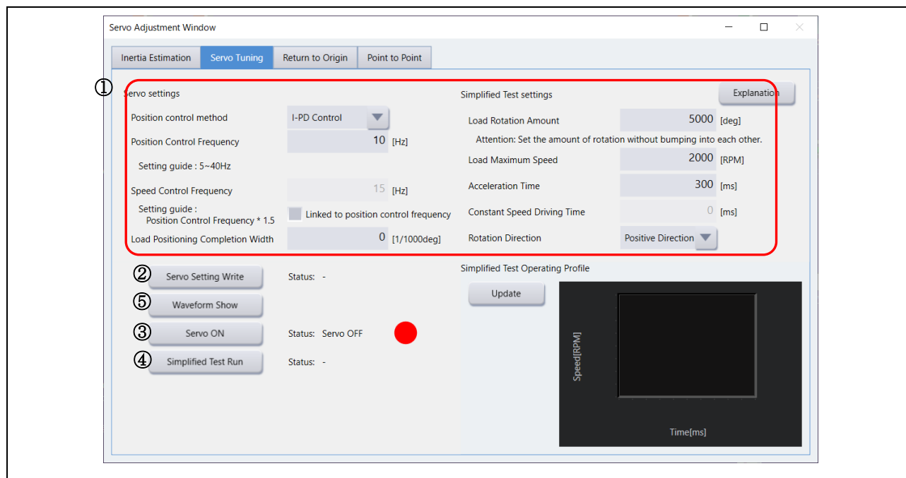
Figure 4-6 Operation window of “Servo Tuning”
