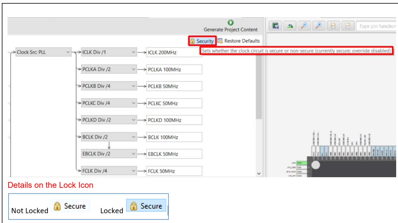
Figure 25. Secure Project Sets Clock as Secure
