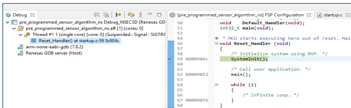
Figure 63. Running the Non-secure Project
