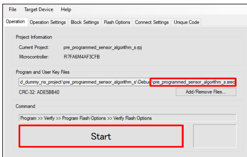
Figure 91. Select the Secure Binary to Program into the MCU
