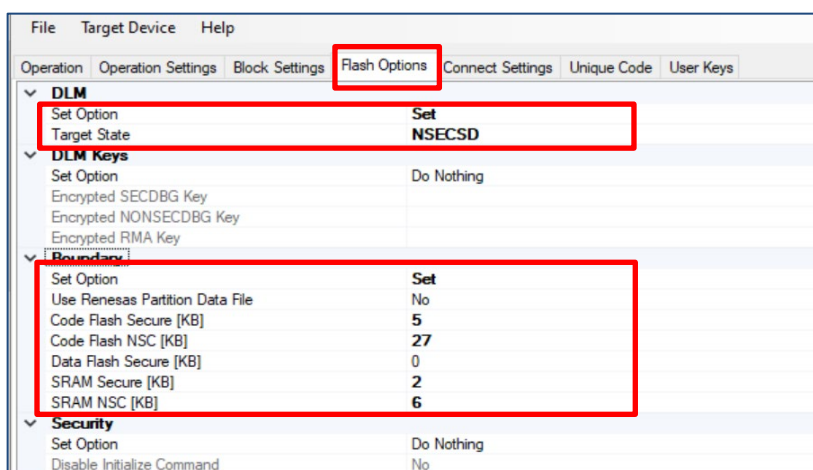
Figure 89. Setup for the IDAU Region
