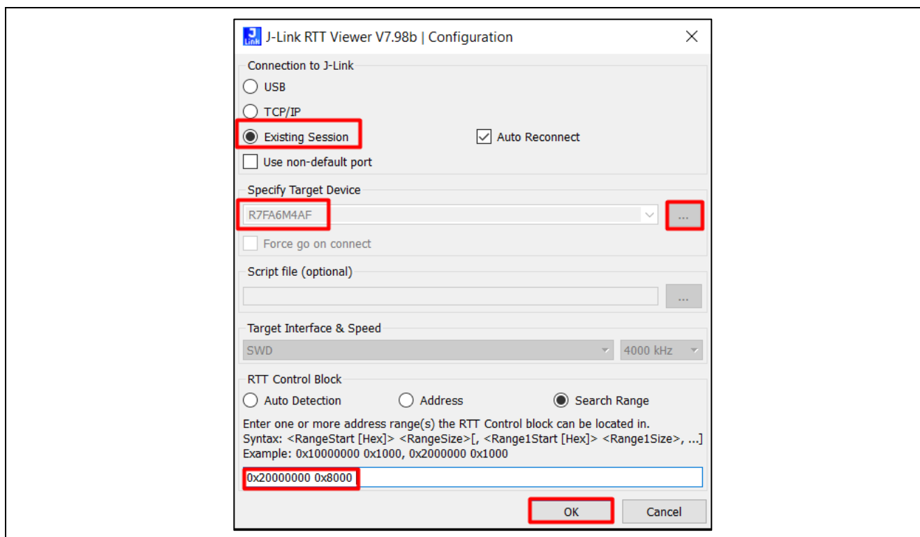
Figure 64. Start the RTT Viewer
