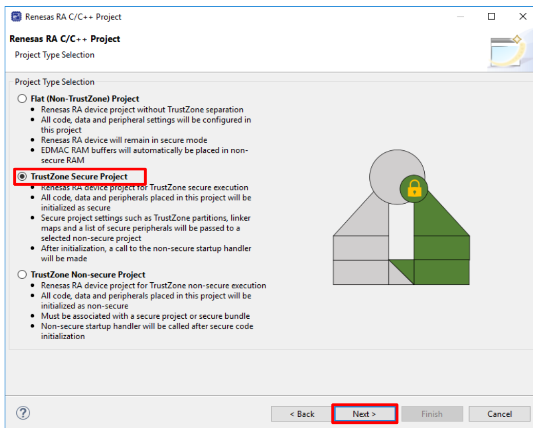
Figure 22. Choose the Secure Project Type
