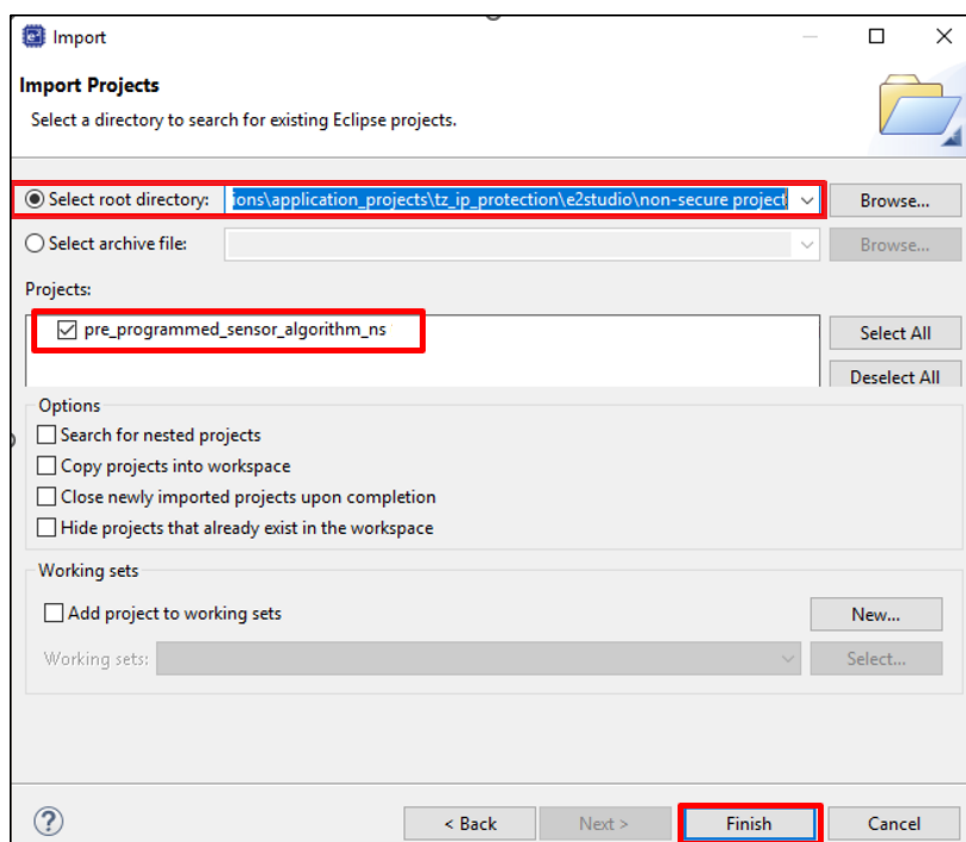
Figure 60. Import the Non-secure Project
