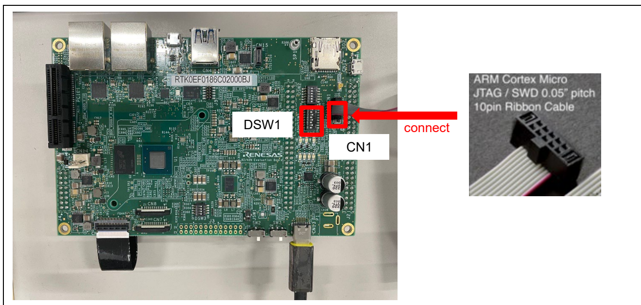
Figure 45: JTAG connection
