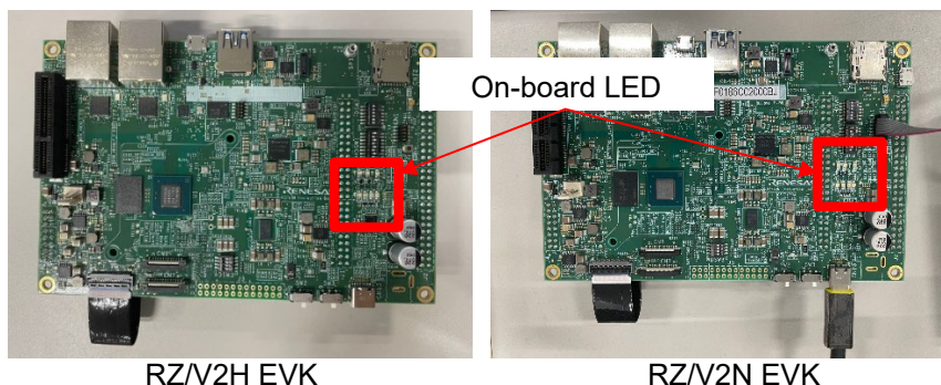
Figure 50: On-board LED of RZ/V2H EVK and RZ/V2N EVK
