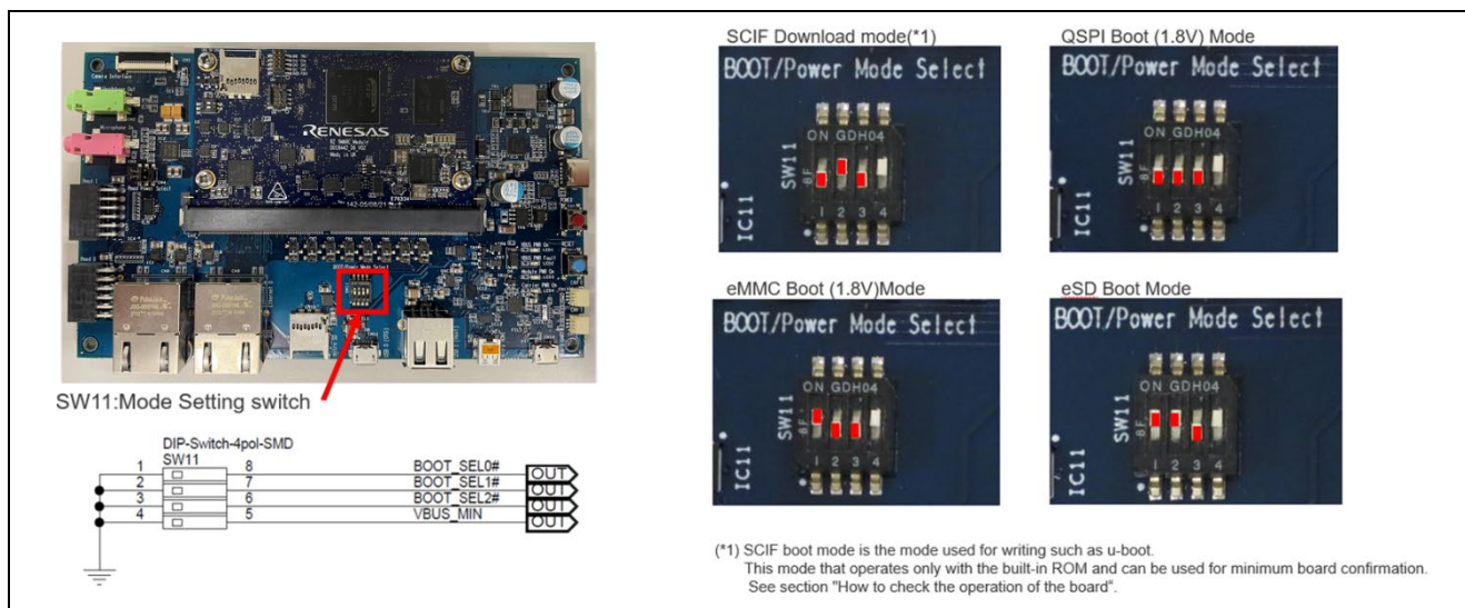
Figure 32: Boot MODE
