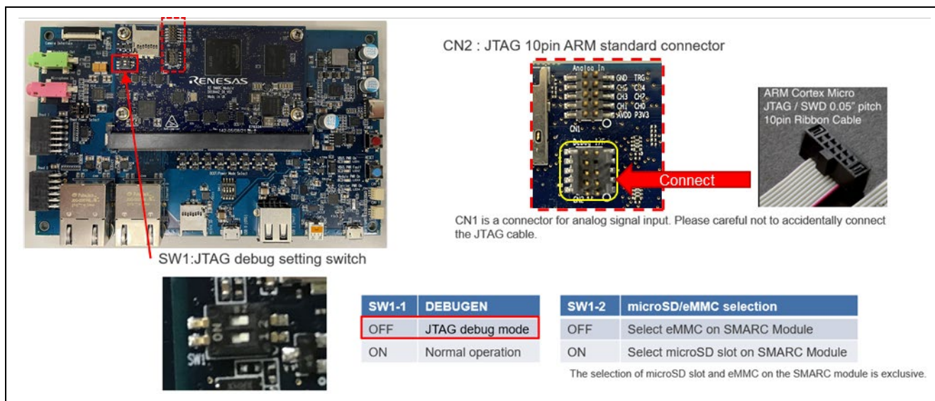
Figure 33: JTAG connection
