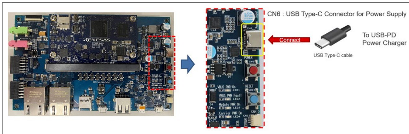
Figure 35: Power Supply
