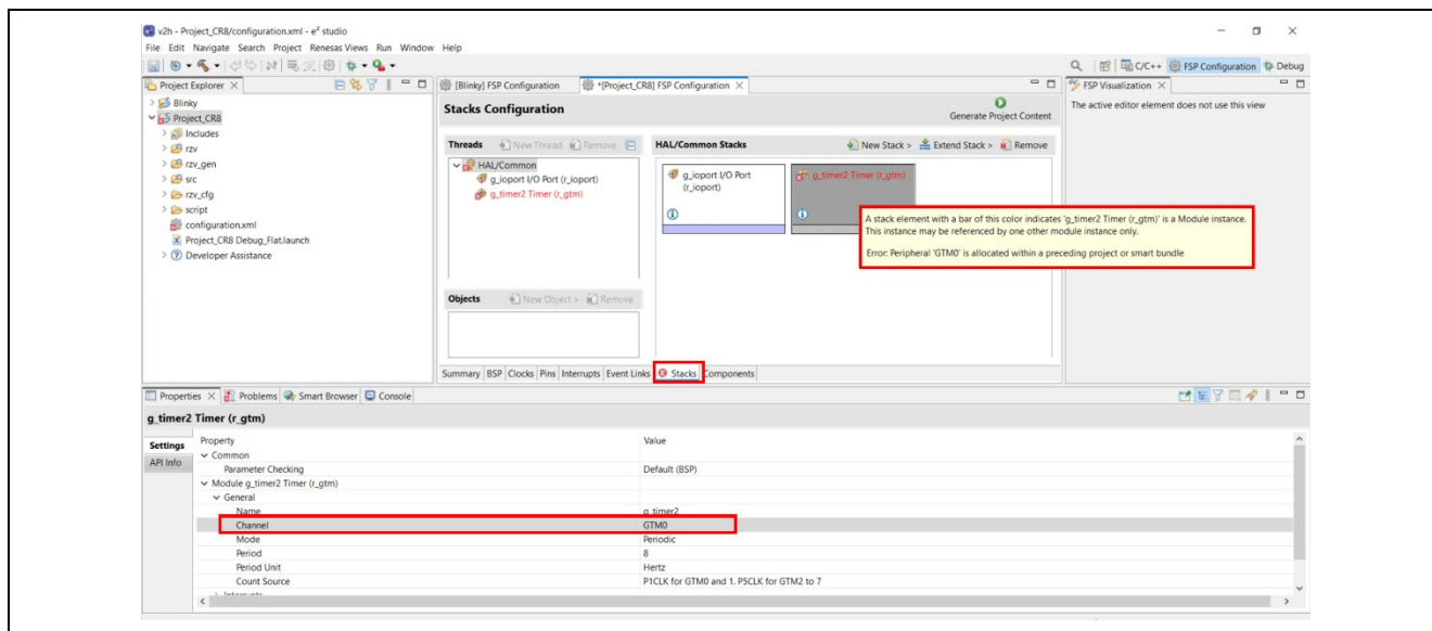
Figure 77 : Duplication of resource between Core 6(CM33_0) and Core 4(CR8_0) projects
