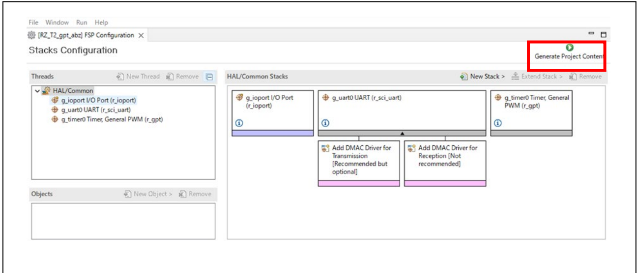
Figure 6-3 Code generator
