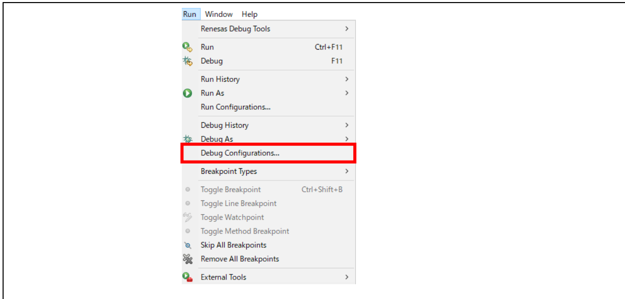
Figure 6-11 Debug Configurations
