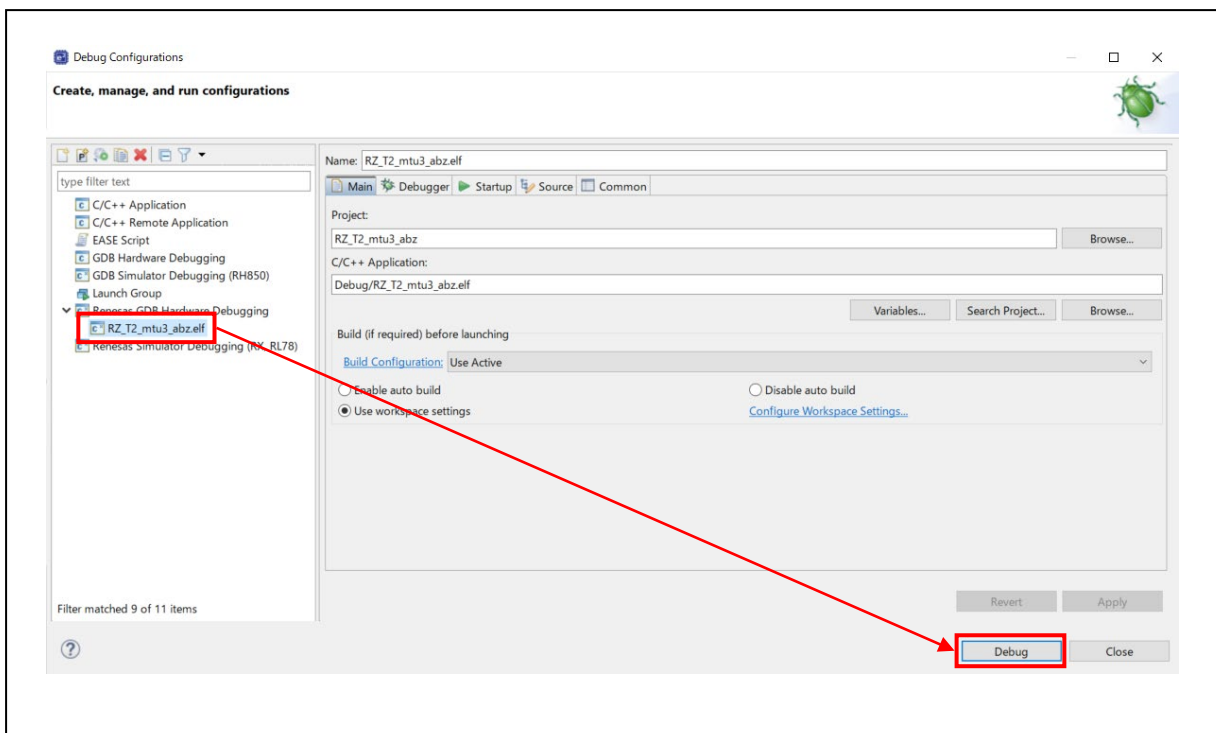
Figure 6-12 Run debug
