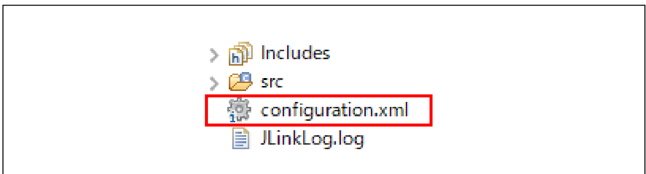
Figure 6-8 Configuration.xml
