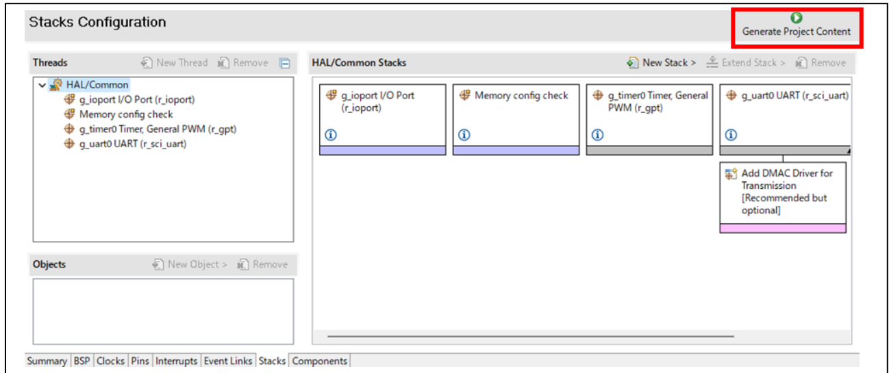
Figure 6-9 Code Generation
