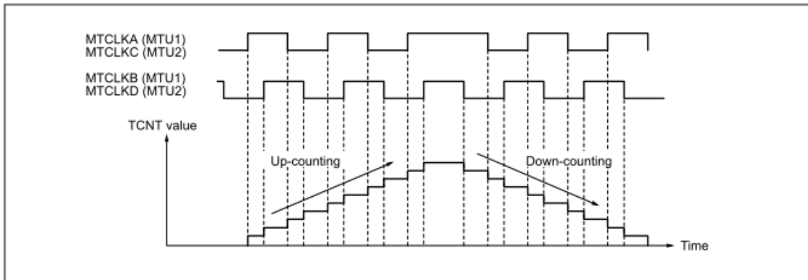
Figure 17.31 Example of operation in phase counting mode 1
