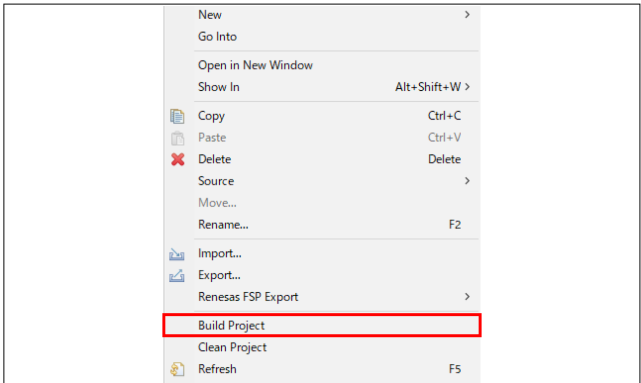
Figure 6-10 Run build
