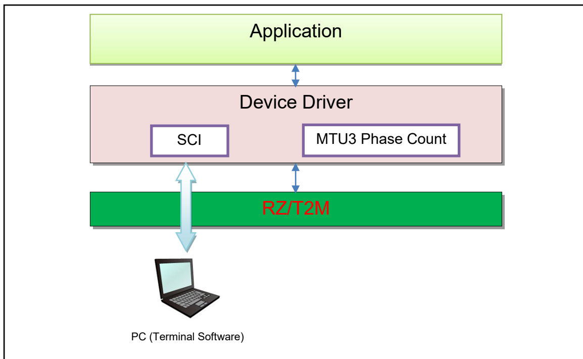
Figure 5-1 Software Configuration
