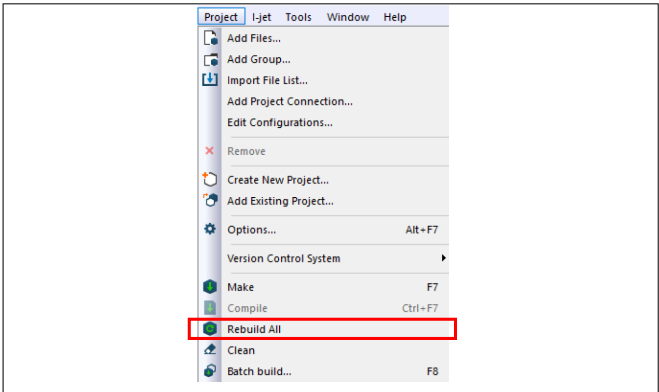
Figure 6-4 Rebuild All
