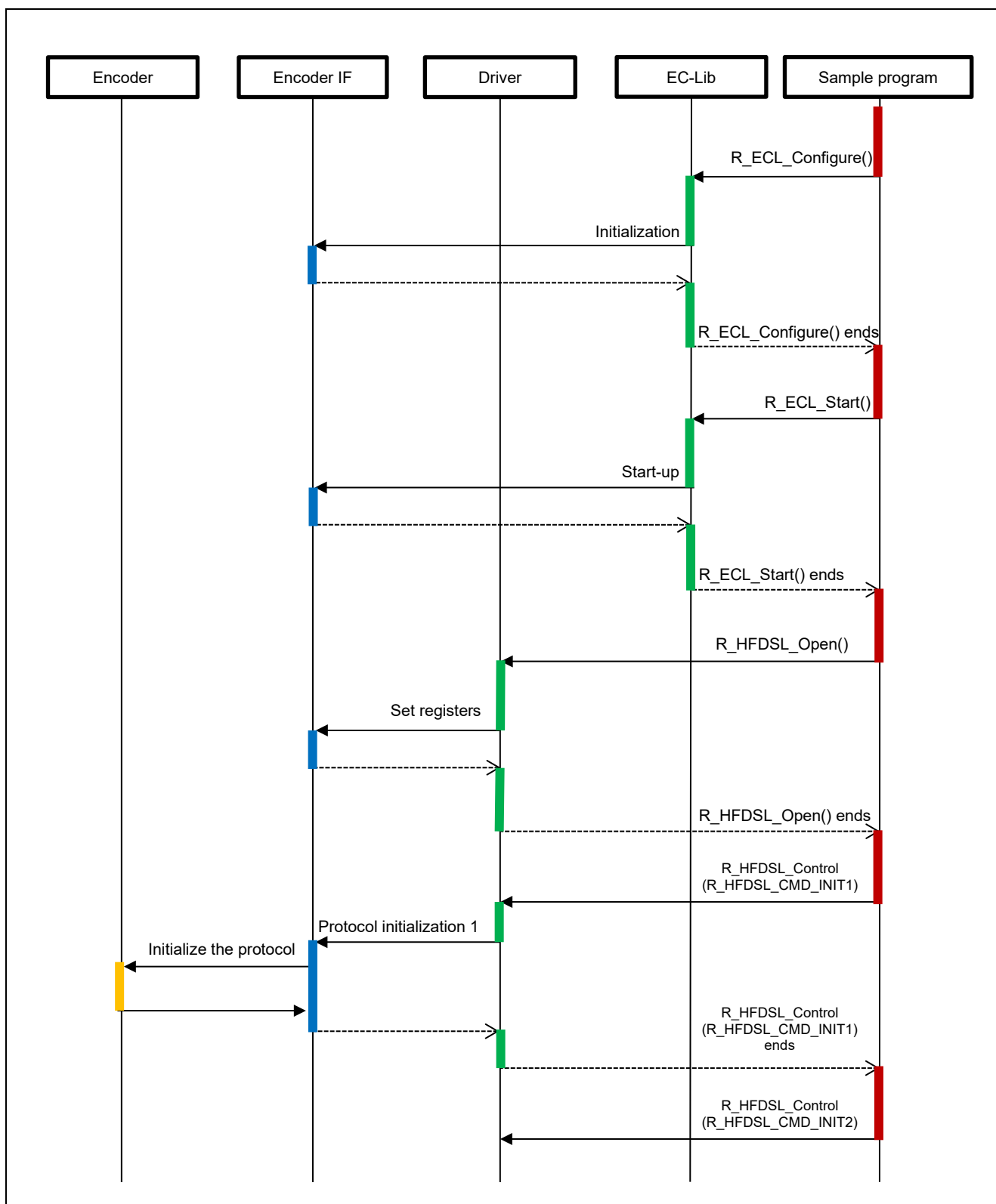
Figure 4.14 Startup Sequence Diagram (1/3)
