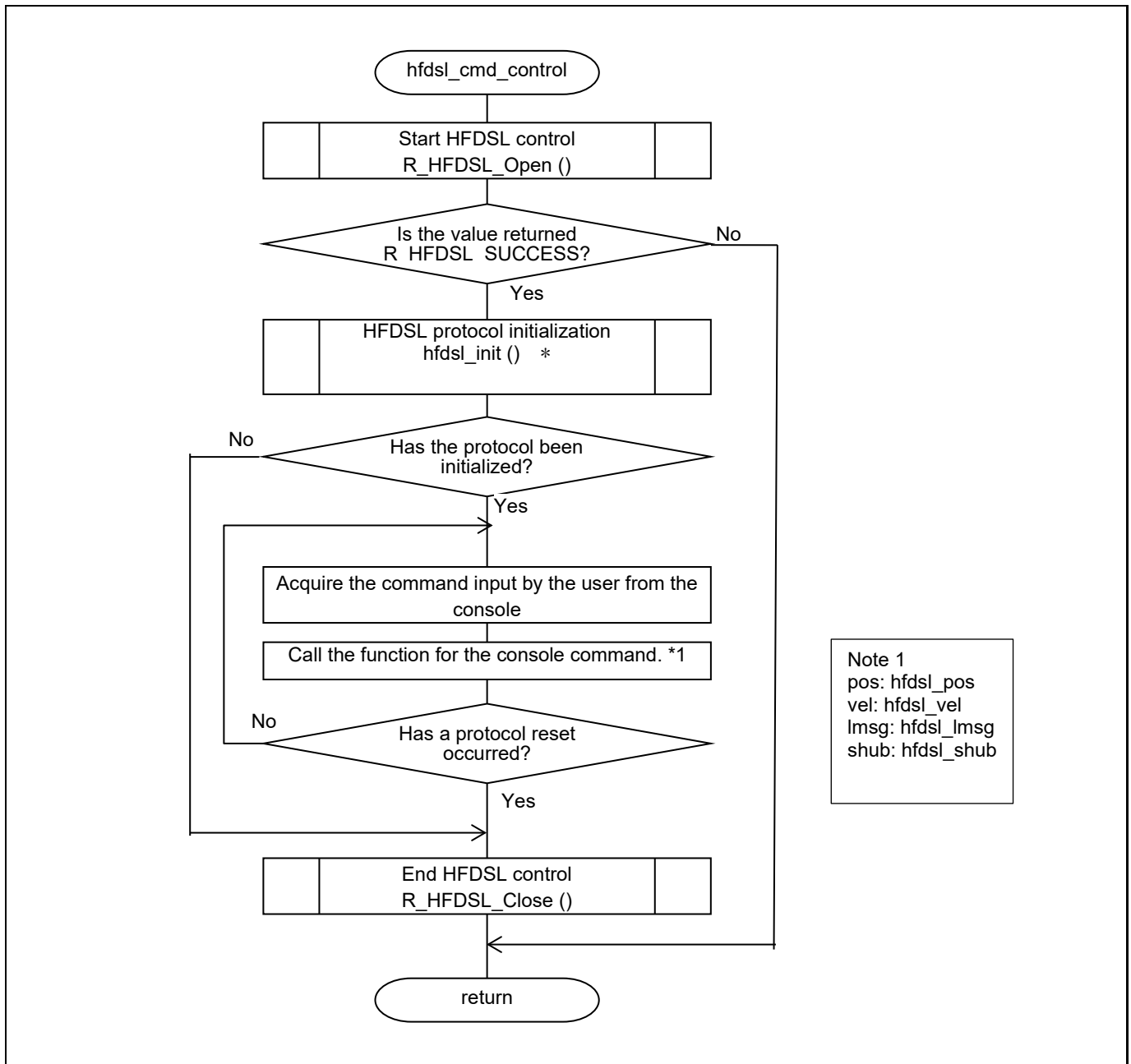
Figure 4.5 Flowchart of hfdsl_cmd_control function
