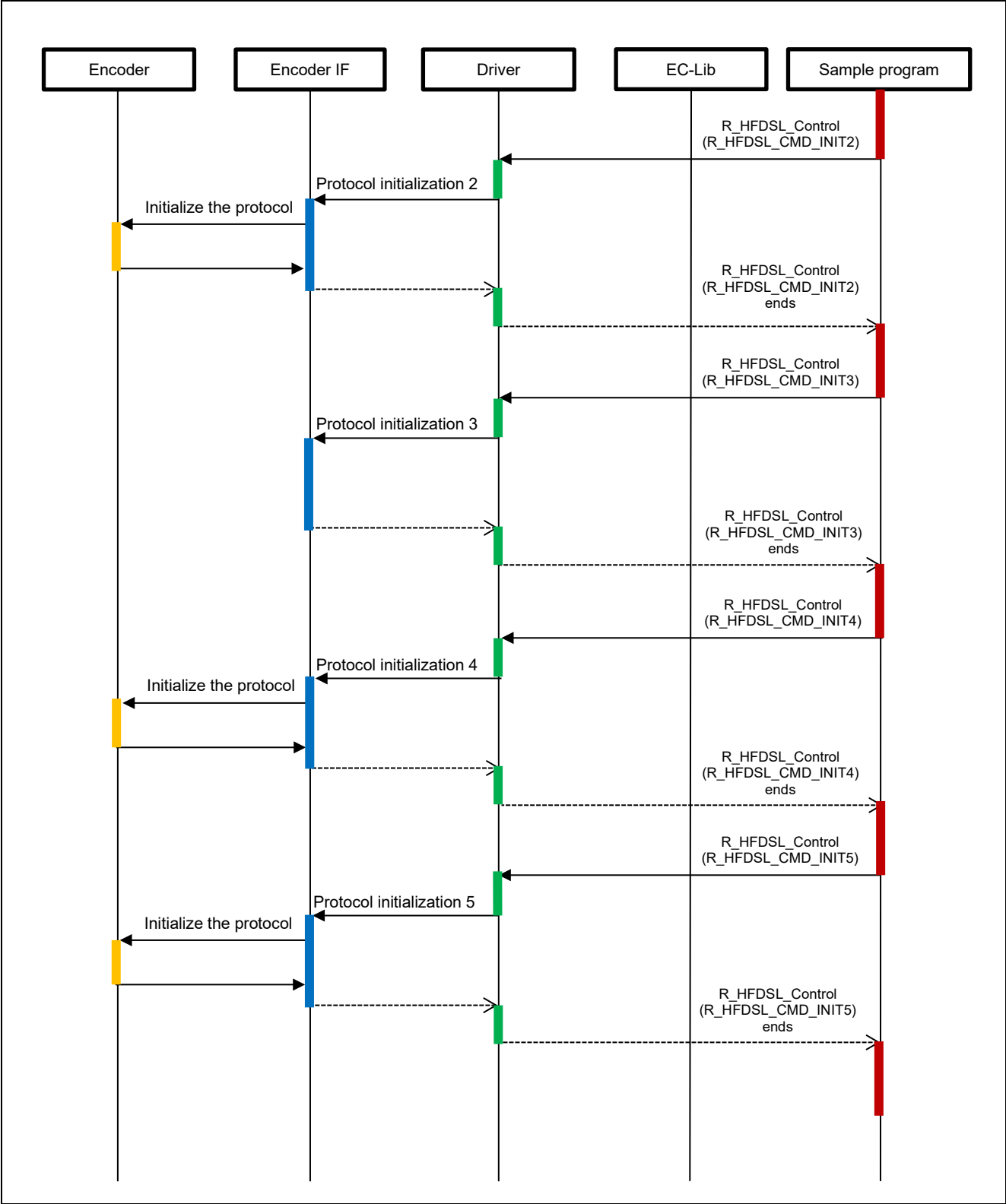
Figure 4.15 Startup Sequence Diagram (2/3)
