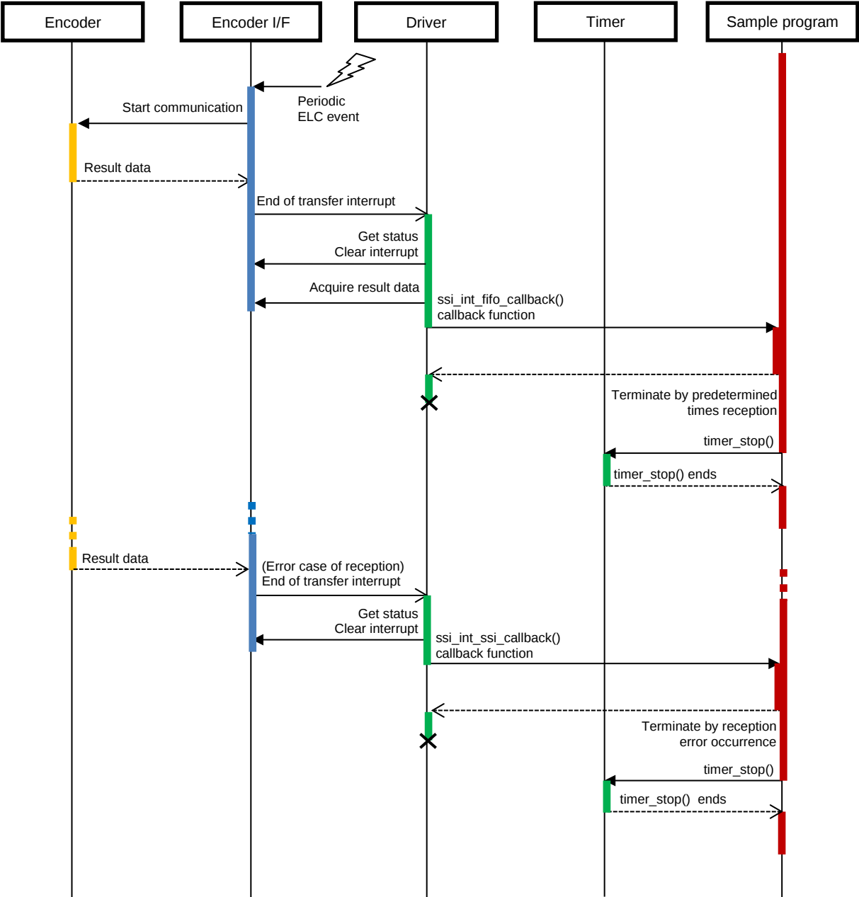
Figure 4.21 Request Data Reception (ELC Operation) Sequence Diagram
