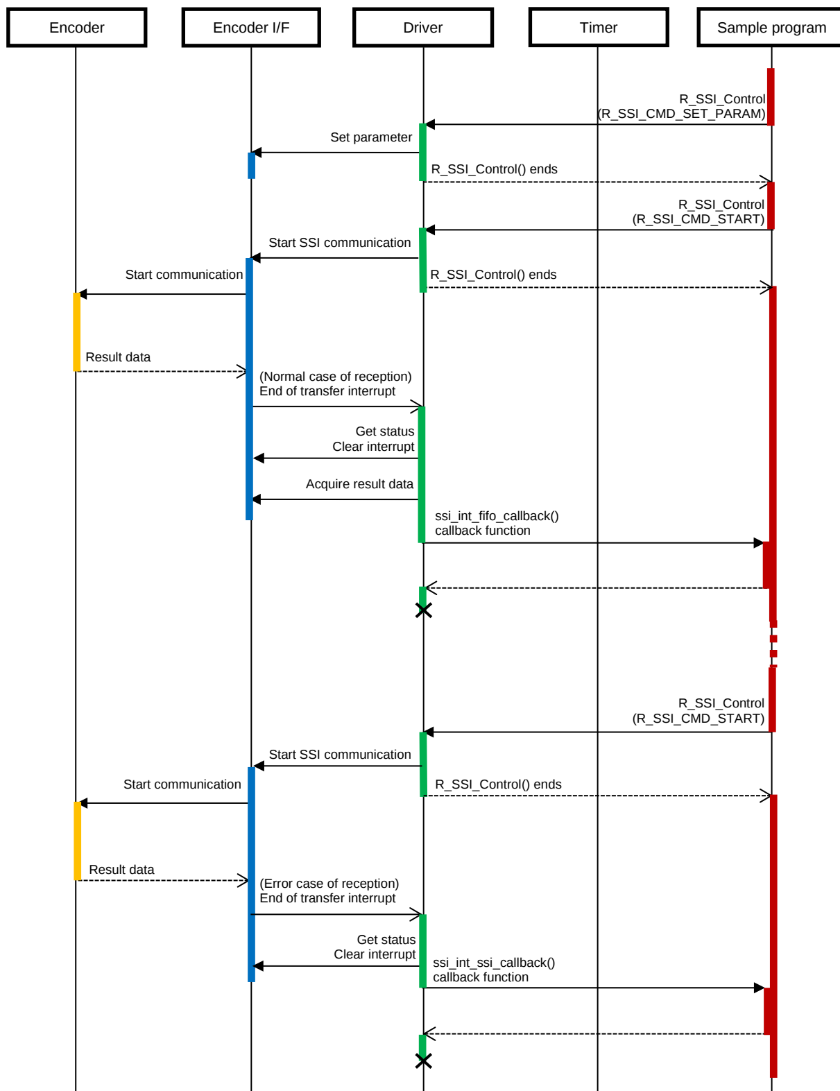
Figure 4.19 Request Data Reception Sequence Diagram
