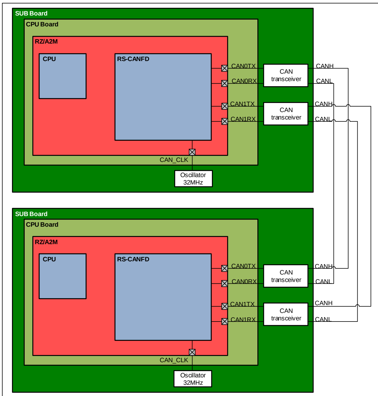
Figure 2-1 Hardware configuration
