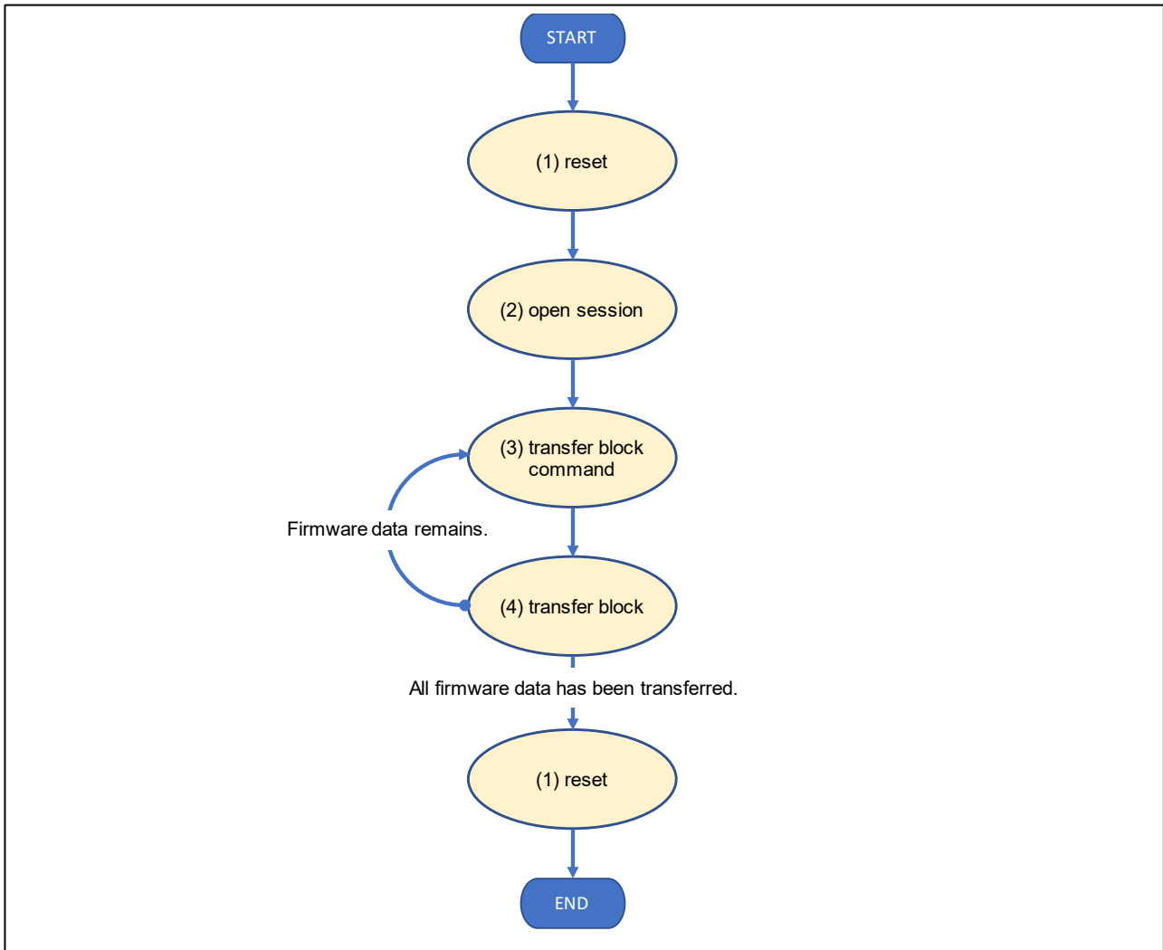
Figure 4-5 Operation flowchart
