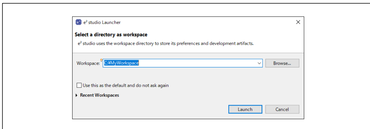
Figure 3-1 Workspace selection
