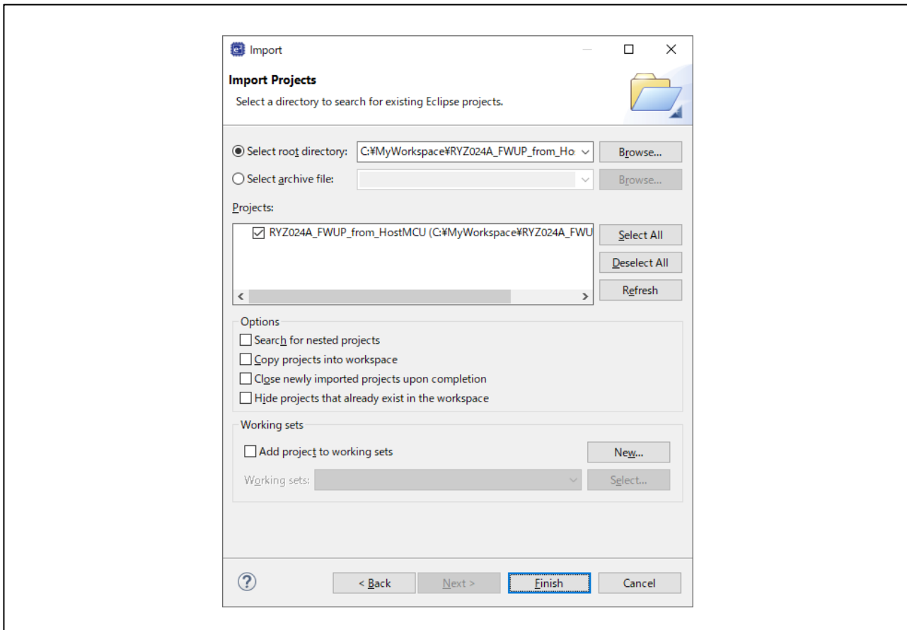
Figure 3-4 Import project
