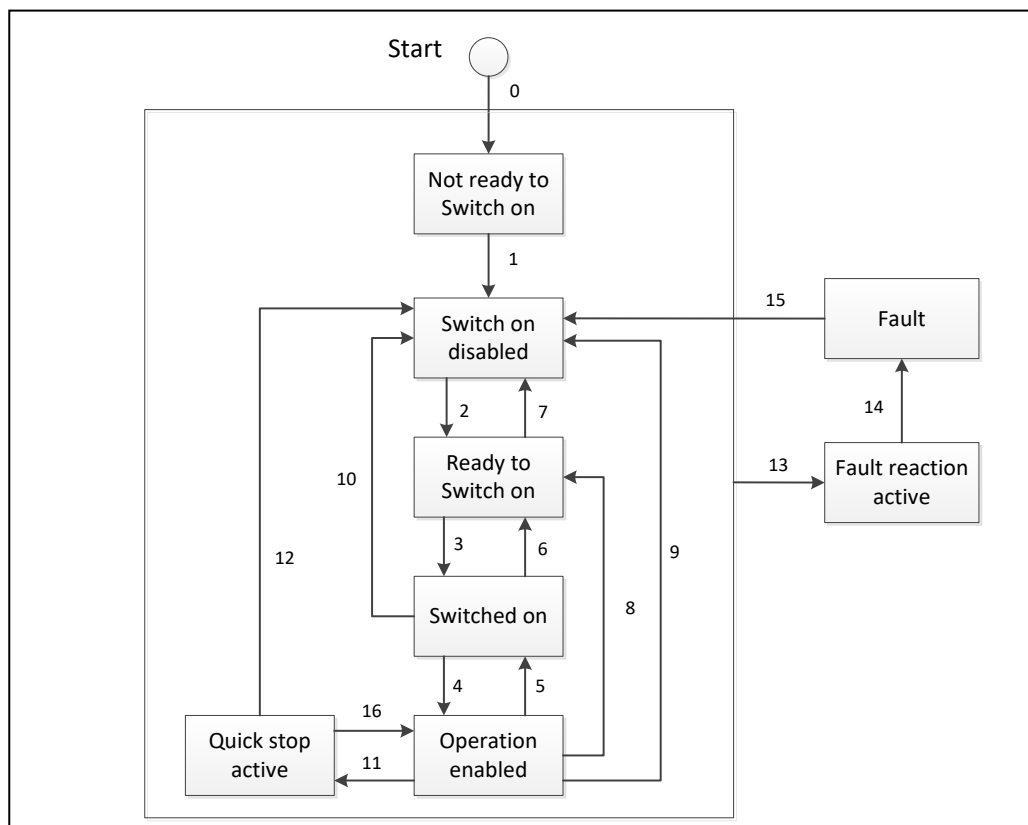
Figure 6-2 CiA402 State Transition Diagram
