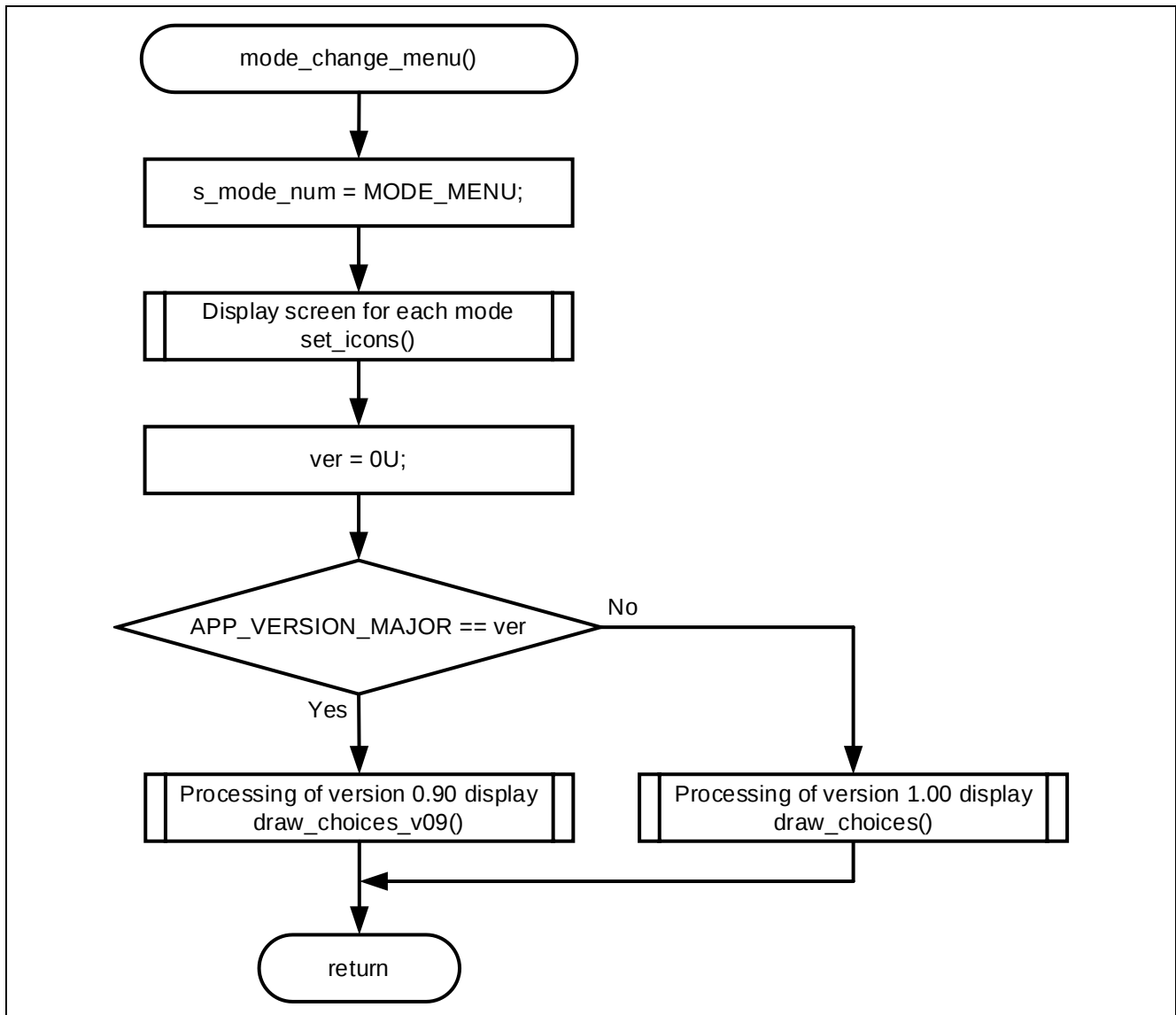
Figure 4-6 Flowchart for moving to the menu screen
