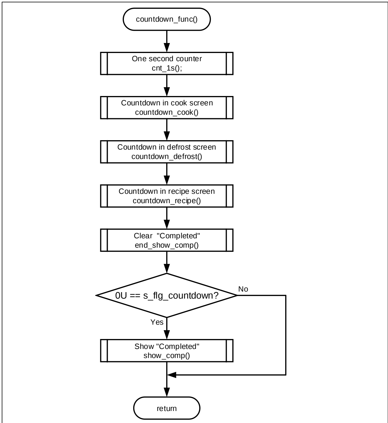
Figure 4-12 Flowchart during cooking
