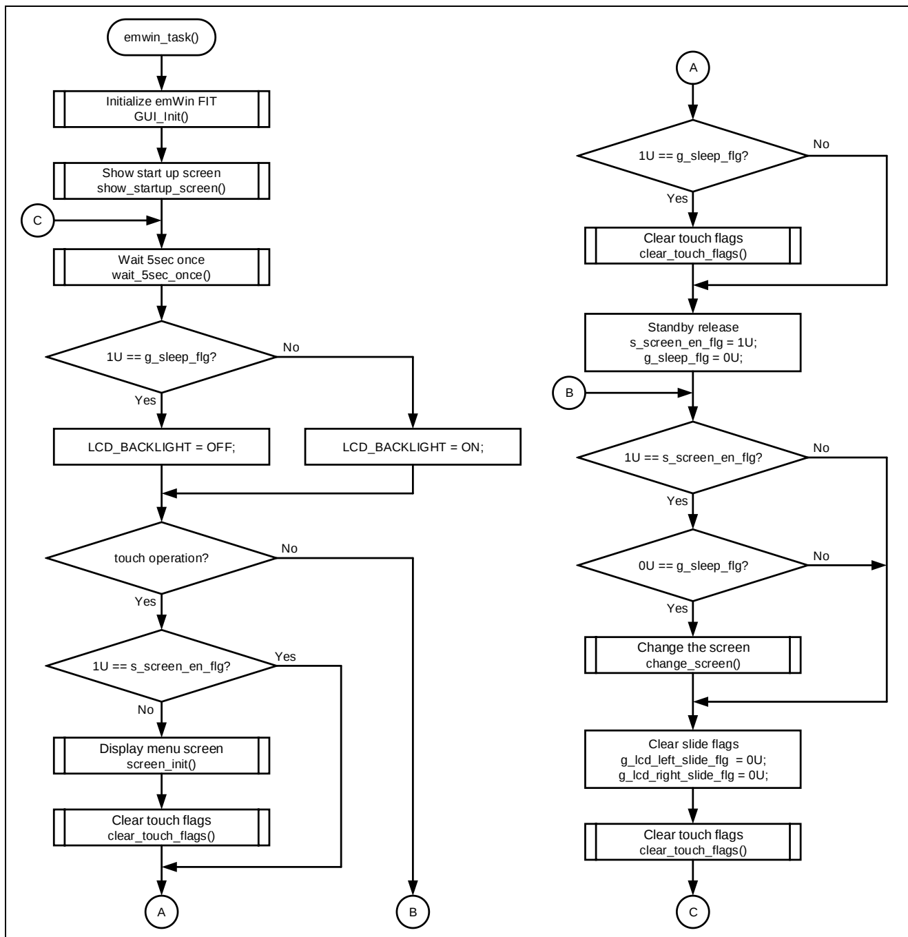
Figure 4-4 Overall flowchart of LCD control
