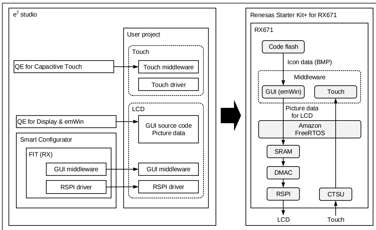
Figure 1-2 Software configuration
