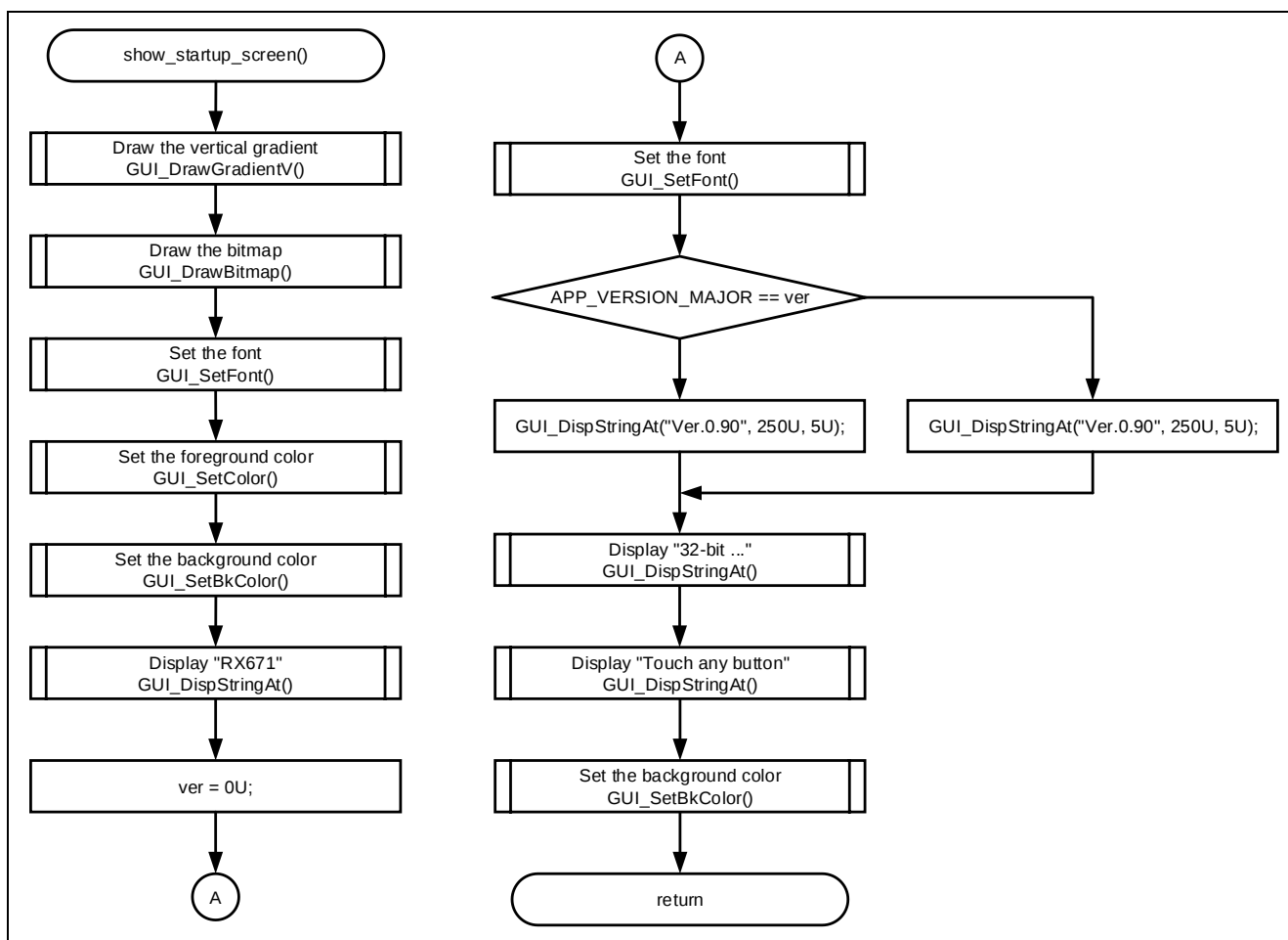
Figure 4-15 Flowchart of startup screen display
