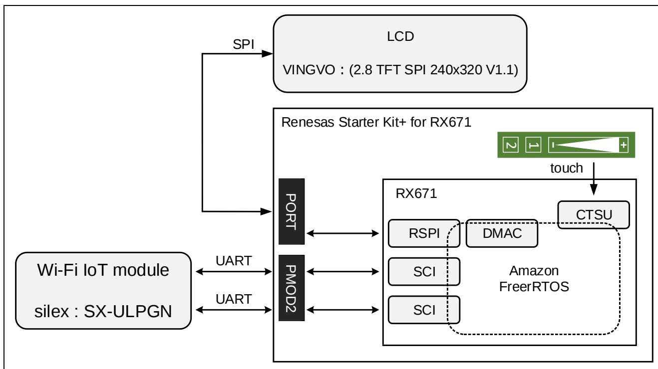
Figure 1-1 System configuration
