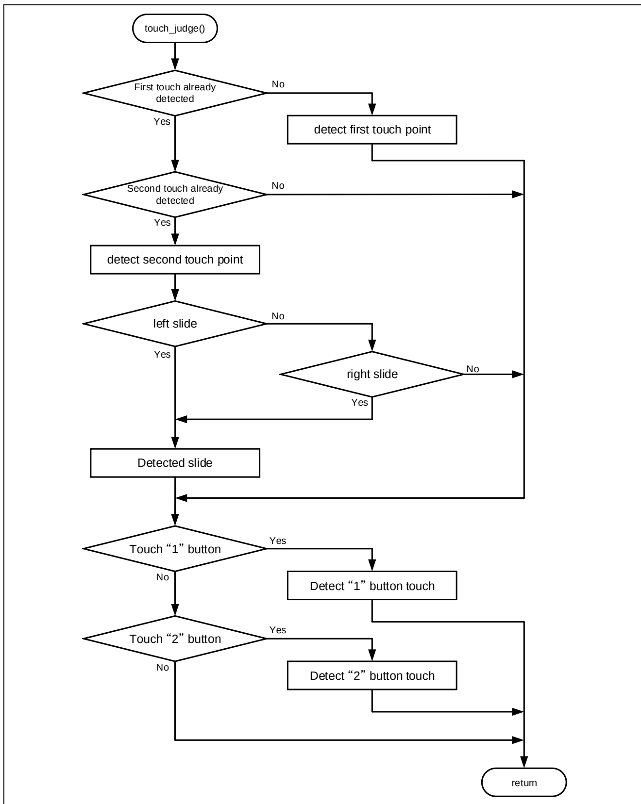
Figure 4-14 Flowchart of touch judgement
