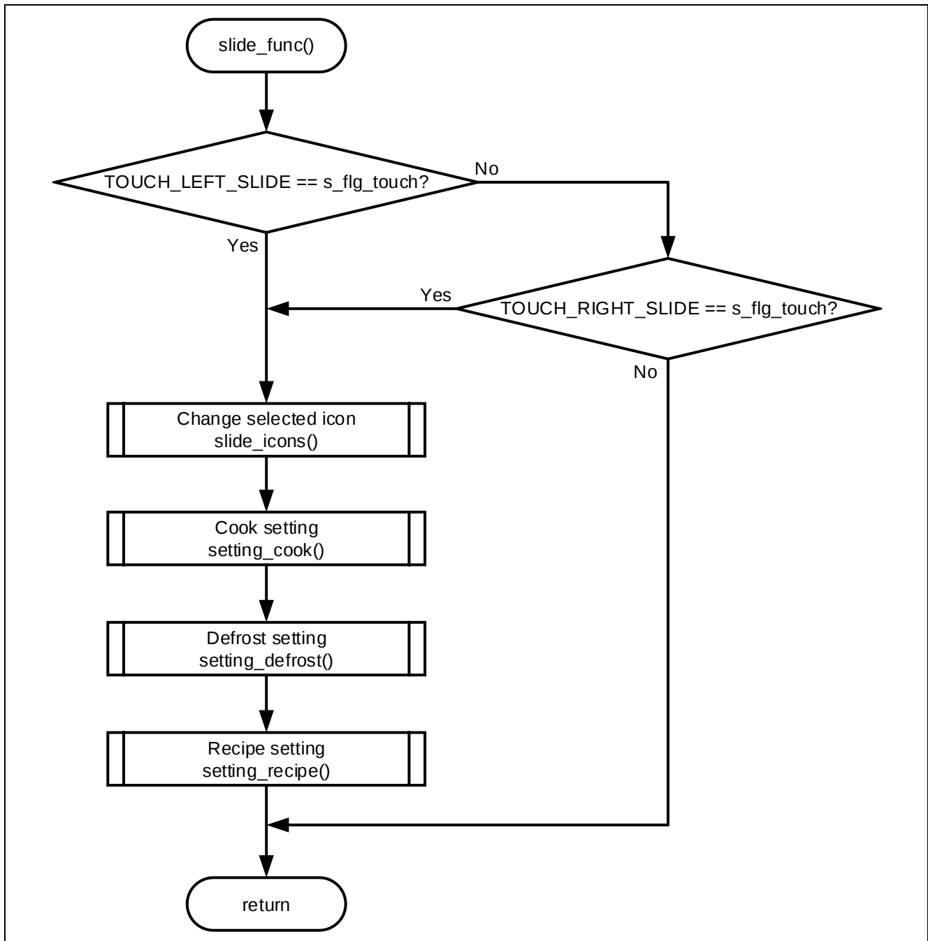
Figure 4-8 Flowchart for touch slider operation
