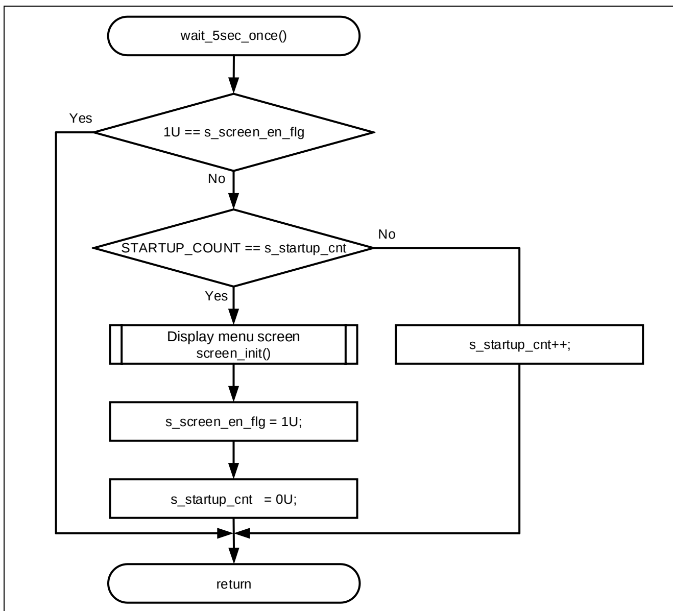
Figure 4-16 Flowchart of 5 seconds wait
