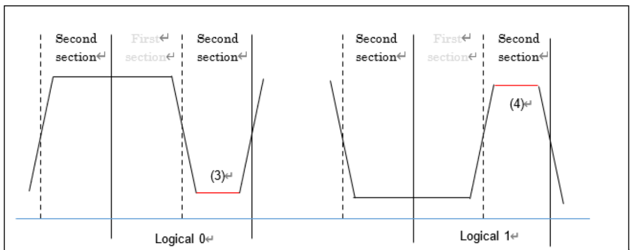
Figure 11 How to determine Double half bit frame data
