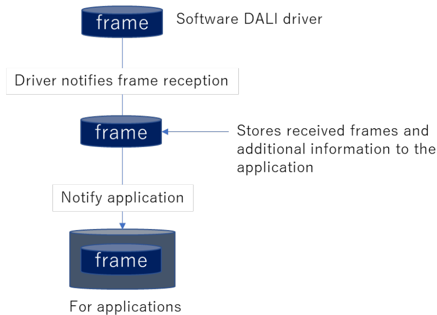
Figure 39 Overview of reception processing
