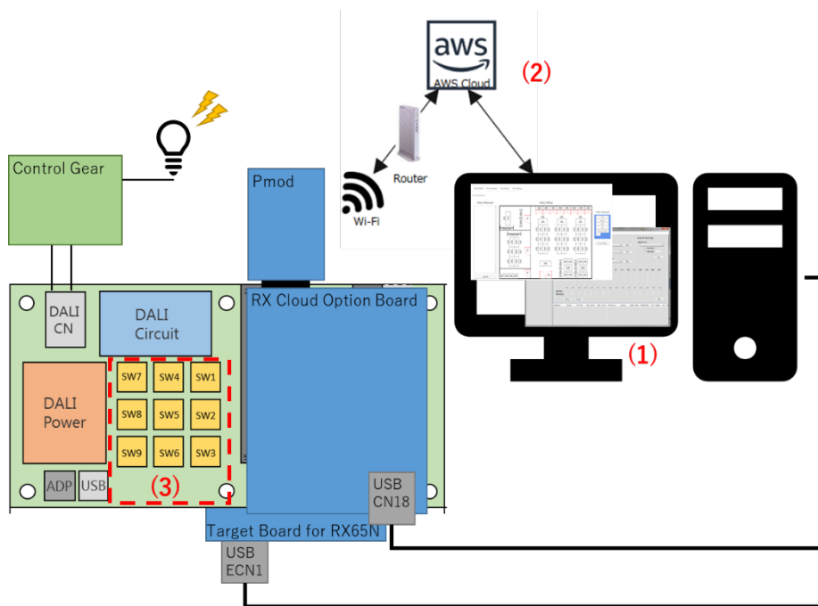
Figure 2 System outline diagram
