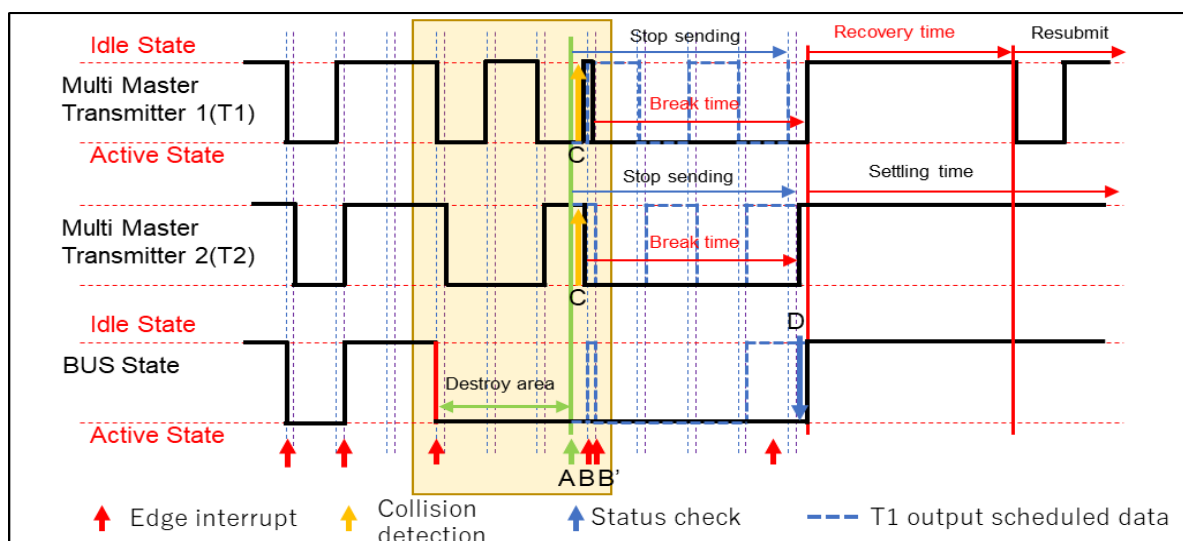
Figure 19 Collision detection in case of Destroy area
