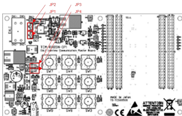
Figure 52 RX65N DALI-2 Option board jumper connection
